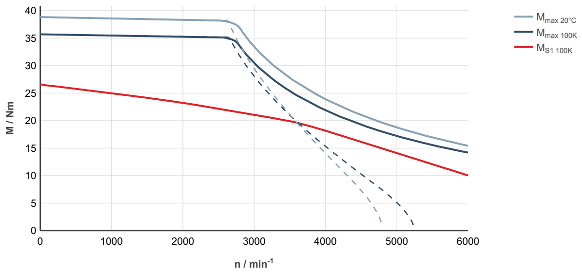
Fig. 165: MS2N07-C0BQL-___0-___-__, ctrlX DRIVE, uncontrolled supply 3 × AC 400 V
