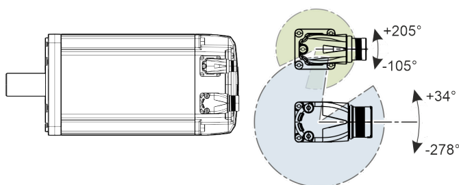
Fig. 381: : Rotating area electrical connection "U"
