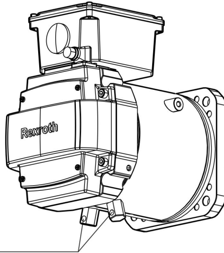
Fig. 392: Coolant connection MS2N10-__L__T__
