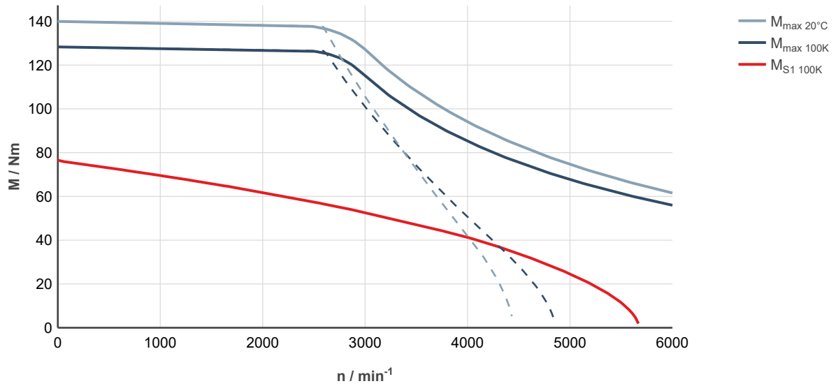
Fig. 184: MS2N07-E1BNL-__0-__-__, ctrlX DRIVE, controlled supply 3 × AC 400 ... 480 V
