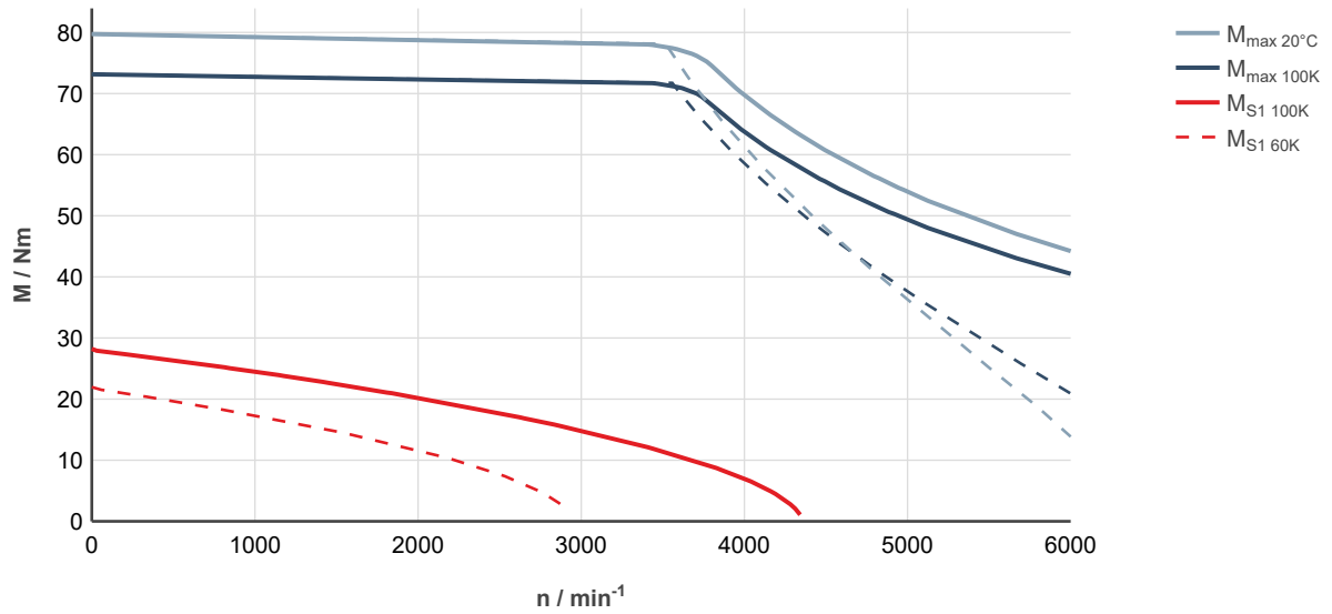
Fig. 106: MS2N07-D0BRN-___0-___-_, ctrlX DRIVE, controlled supply 3 × AC 400 ... 480 V
