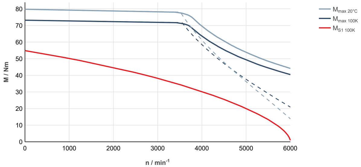
Fig. 174: MS2N07-D0BRL-___0-___-___, ctrlX DRIVE, controlled supply 3 × AC 400 ... 480 V
