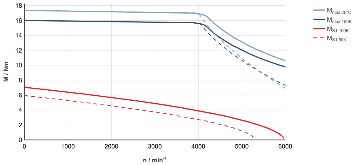
Fig. 72: MS2N06-C0BTN-___0-___-__, ctrlX DRIVE, uncontrolled supply 3 × AC 400 V
