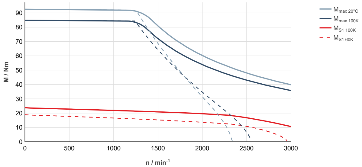
Fig. 108: MS2N07-D1BFN-___0-___-_, ctrlX DRIVE, controlled supply 3 × AC 400 ... 480 V
