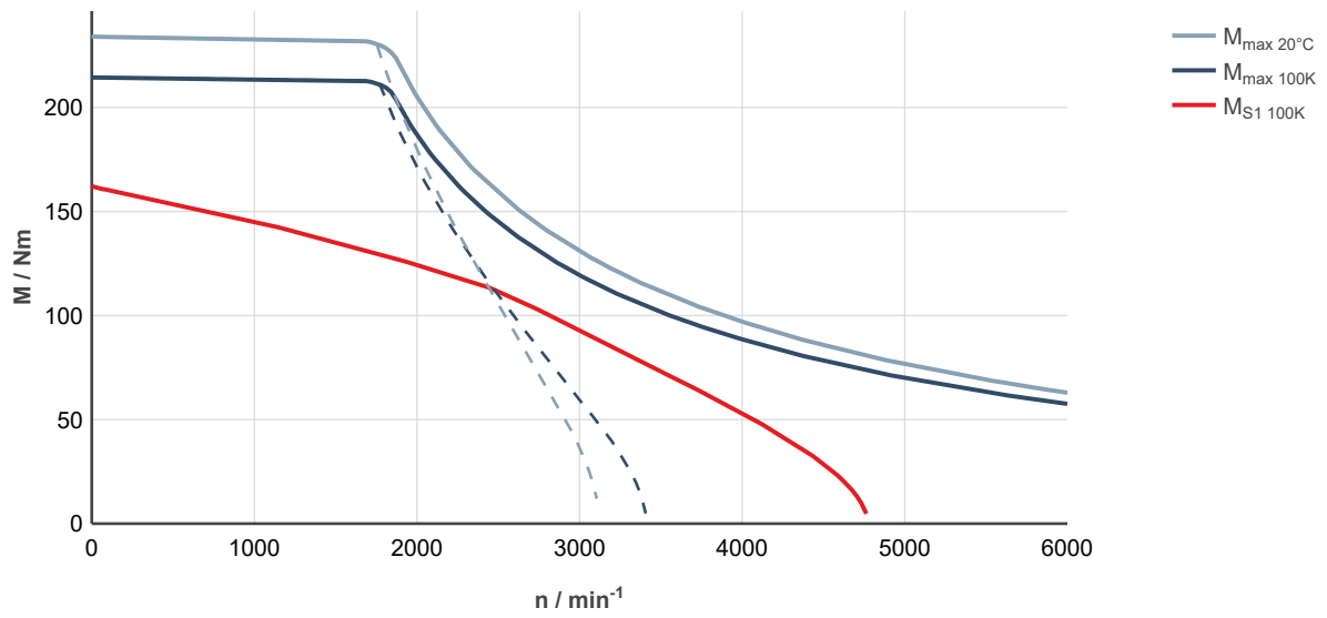
Fig. 276: MS2N10-E0BNL-___0-___-___, ctrlX DRIVE, uncontrolled supply 3 × AC 400 V
