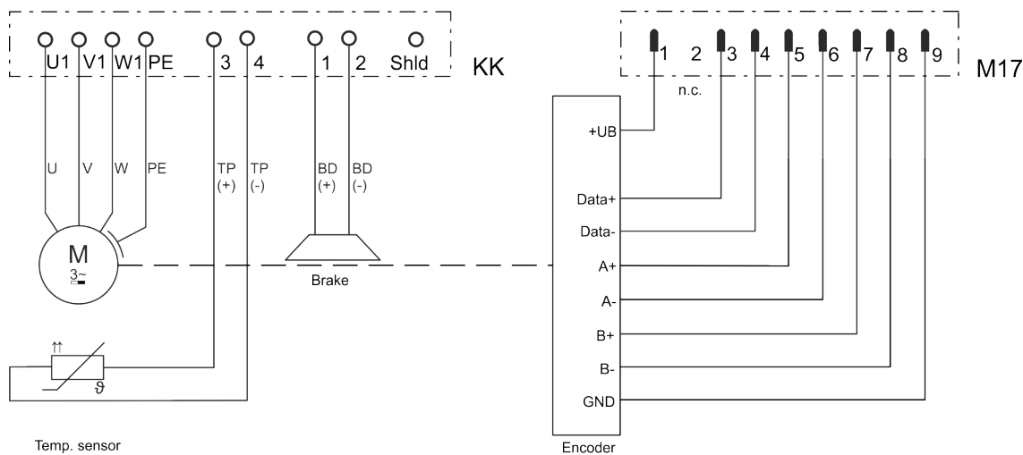
Fig. 361: Double cable connection terminal boxes, analog encoder A, brake optional
