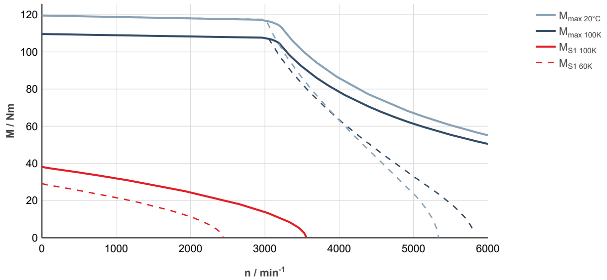
Fig. 120: MS2N07-E0BQN-___0-___-, ctrlX DRIVE, controlled supply 3 × AC 400 ... 480 V
