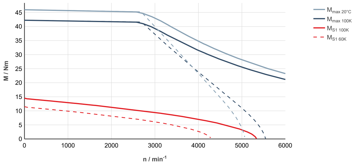
Fig. 97: MS2N07-C1BRN-___0-___-__, ctrlX DRIVE, uncontrolled supply 3 × AC 400 V
