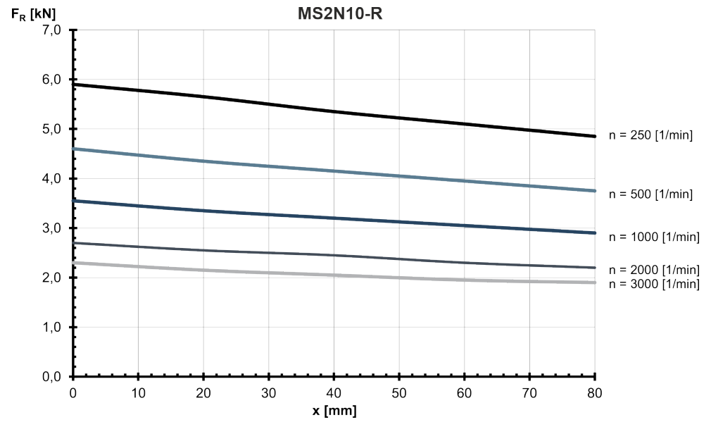
Fig. 301: MS2N10-R: Radial force in distance x from the shaft shoulder at a nominal bearing service life of L_{h10} = 30000 h
