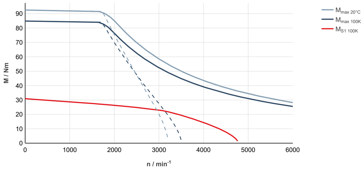
Fig. 147: MS2N07-D1BNA-___0-___- , ctrlX DRIVE, uncontrolled supply 3 × AC 400 V
