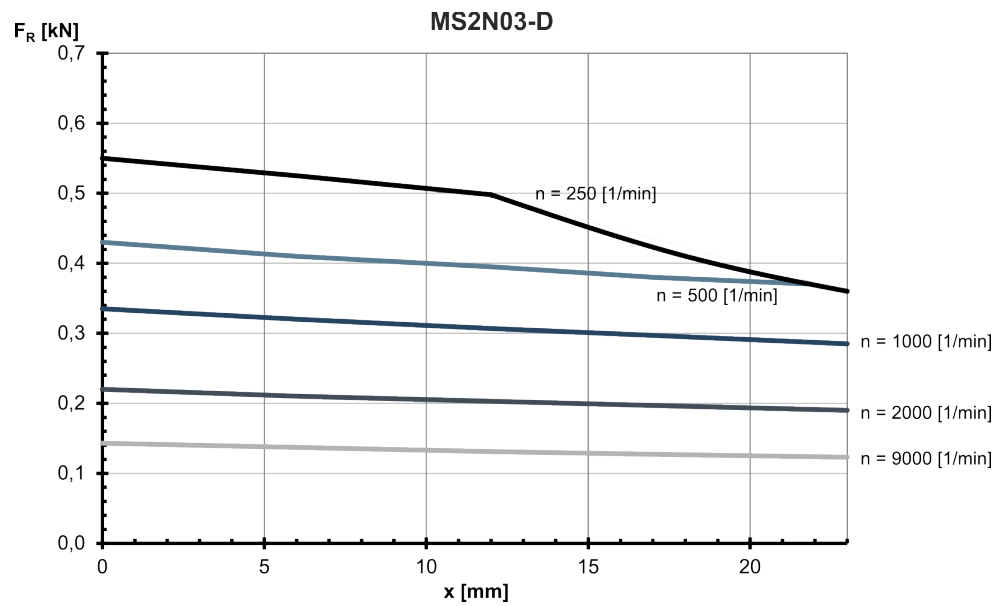
Fig. 33: MS2N03-D: Radial force in distance x from the shaft shoulder at a nominal bearing service life of L_{h10} = 30000 h
