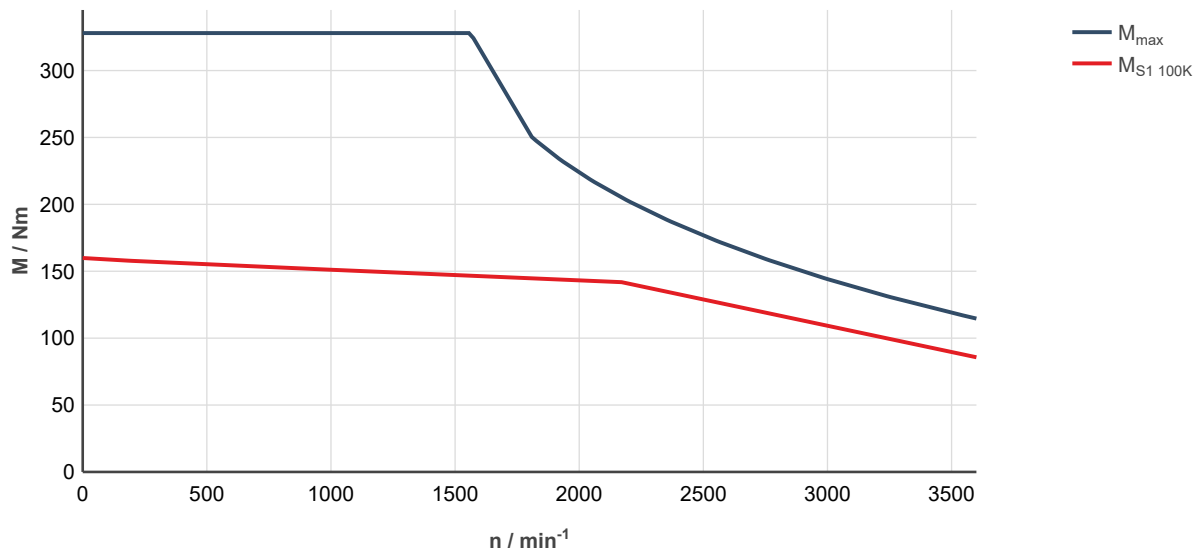
Fig. 318: MS2N13-B1BHC-___0-___-_, ctrIX DRIVE, uncontrolled supply 3 × AC 400 V M_{\text{max}} Characteristic curve applies to maximum torque 20 °C (cold)
