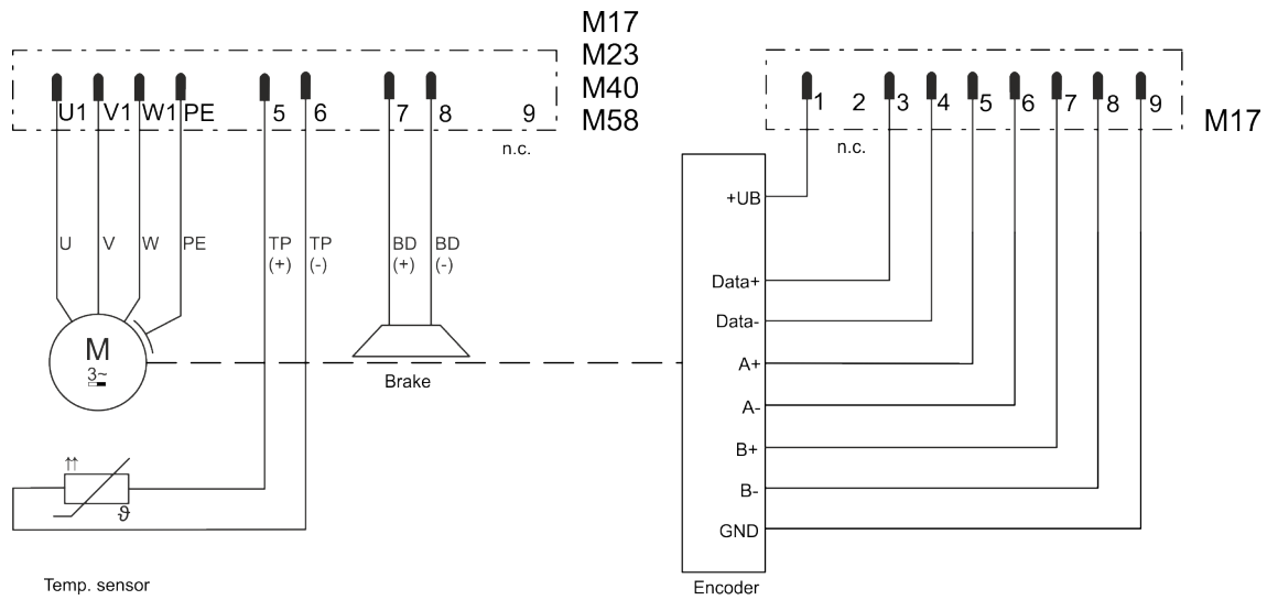
Fig. 359: Double cable connection, analog encoder A, brake optional
