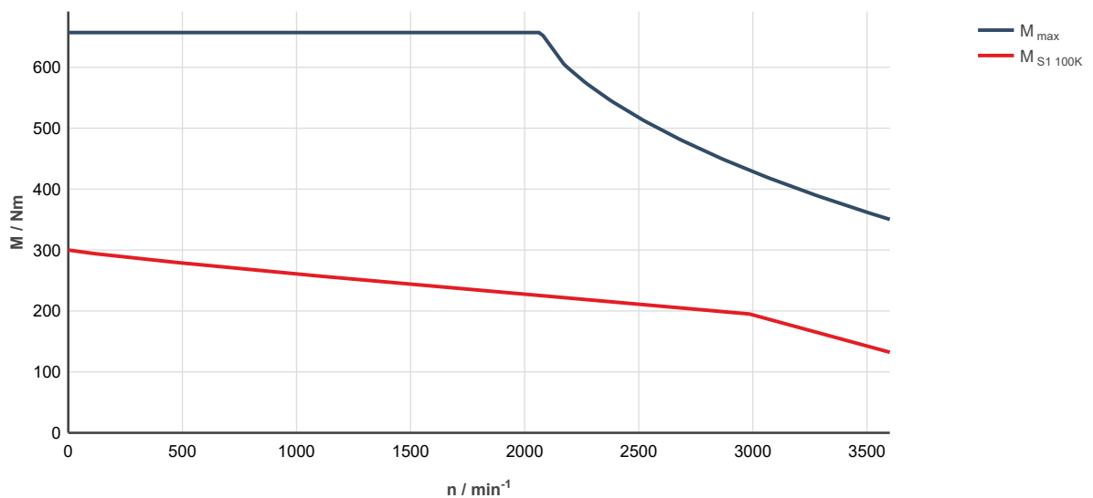
Fig. 331: MS2N13-E1BHC-___0-___-_, ctrlX DRIVE, controlled supply 3 × AC 400 ... 480 V M_{\text{max}} Characteristic curve applies to maximum torque 20 °C (cold)
