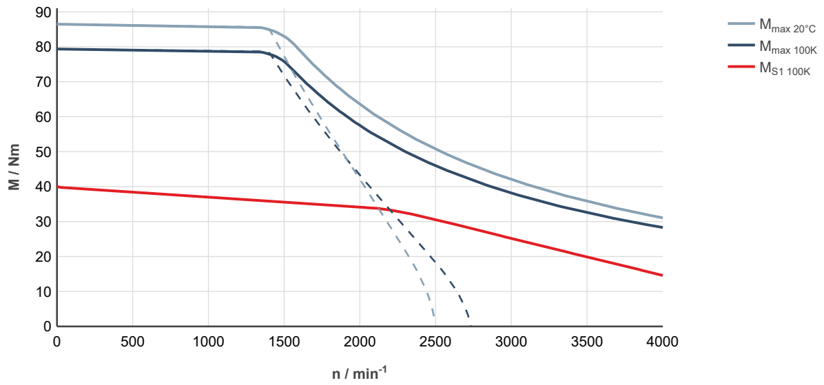
Fig. 232: MS2N10-C1BHA-___0-___-_, ctrIX DRIVE, uncontrolled supply 3 x AC 400 V
