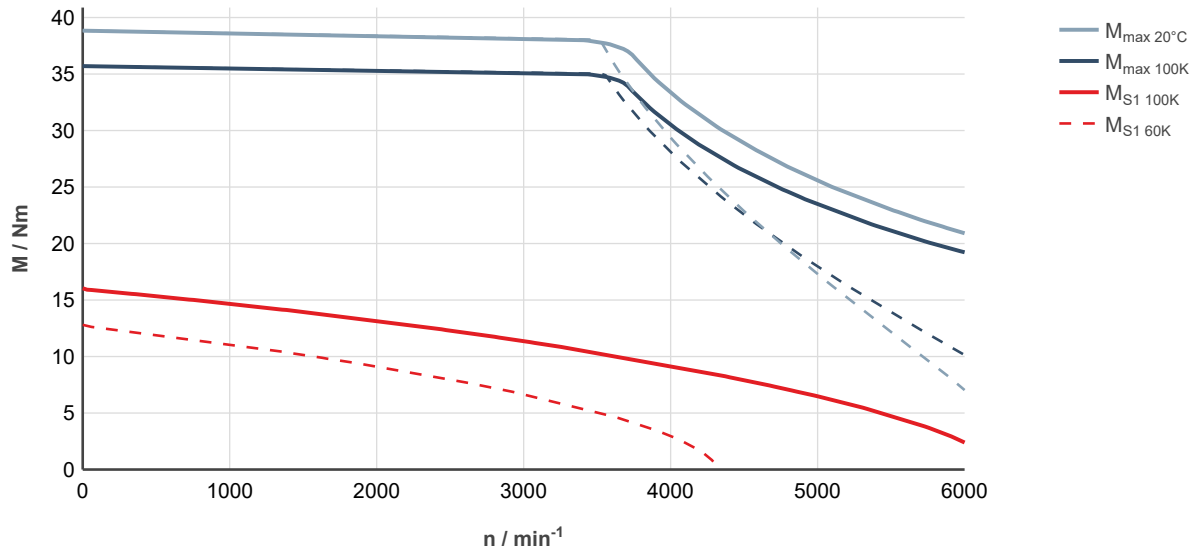
Fig. 94: MS2N07-C0BQN-___0-___-_, ctrlX DRIVE, controlled supply 3 × AC 400 ... 480 V
