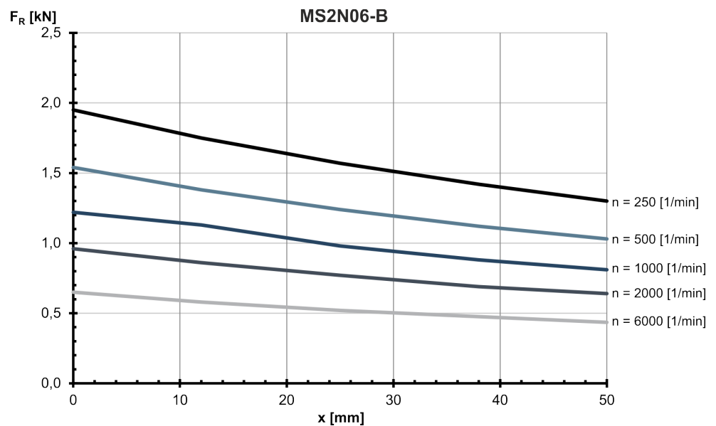
Fig. 85: MS2N06-B: Radial force in distance x from the shaft shoulder at a nominal bearing service life of L_{h10} = 30000 h
