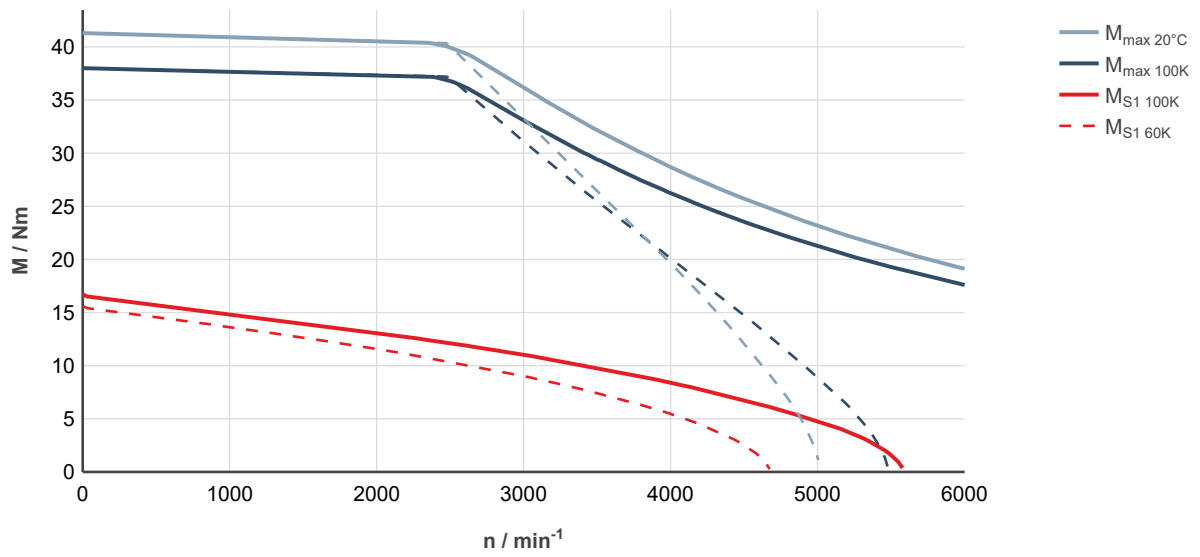
Fig. 192: MS2N10-B1BQN-___0-___-_, ctrlX DRIVE, uncontrolled supply 3 × AC 400 V
