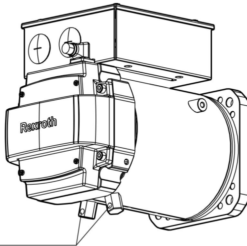
Fig. 393: Coolant connection MS2N10-__L__C__
