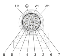
Fig. 376: Connector view of M17 single cable connector
