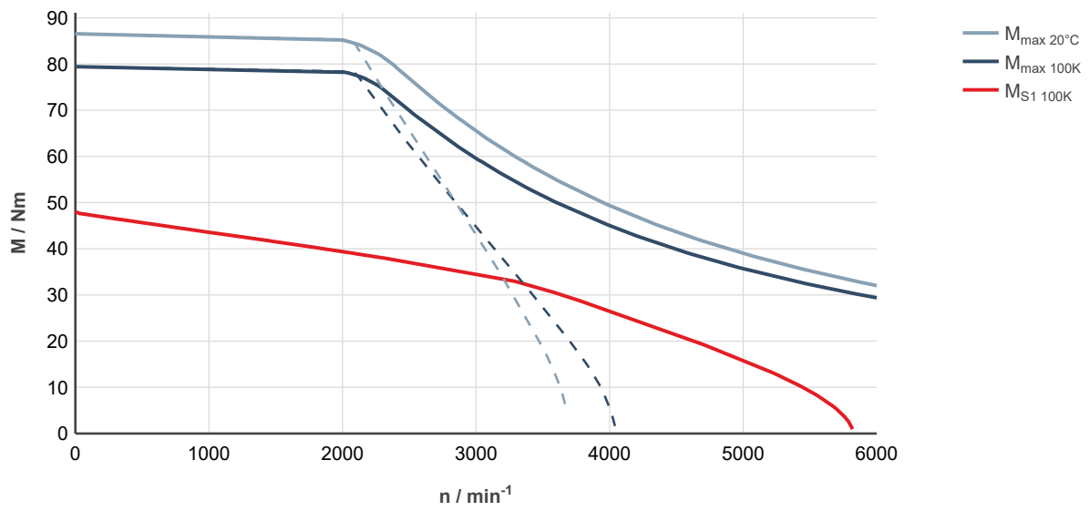
Fig. 266: MS2N10-C1BNL-___0-___-___, ctrIX DRIVE, uncontrolled supply 3 × AC 400 V
