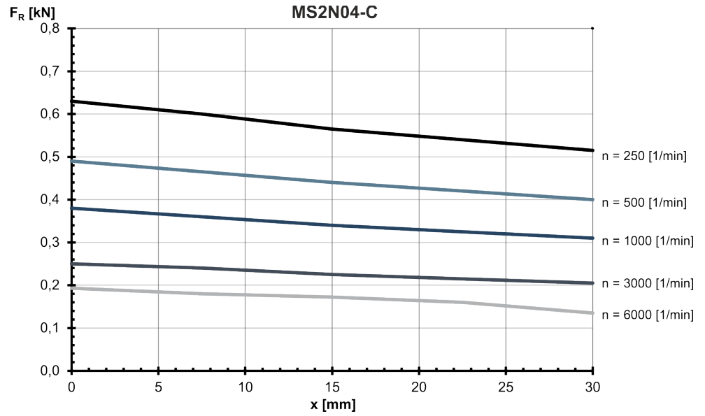
Fig. 49: MS2N04-C: Radial force in distance x from the shaft shoulder at a nominal bearing service life of L_{h10} = 30000 h
