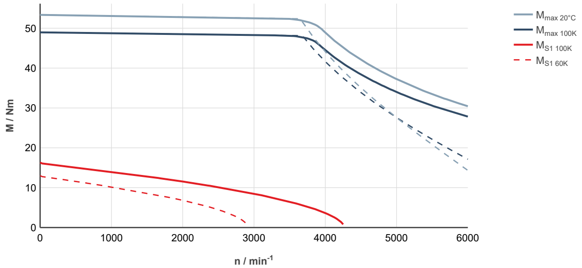
Fig. 83: MS2N06-E0BRN-___0-___-__, ctrlX DRIVE, controlled supply 3 × AC 400 ... 480 V
