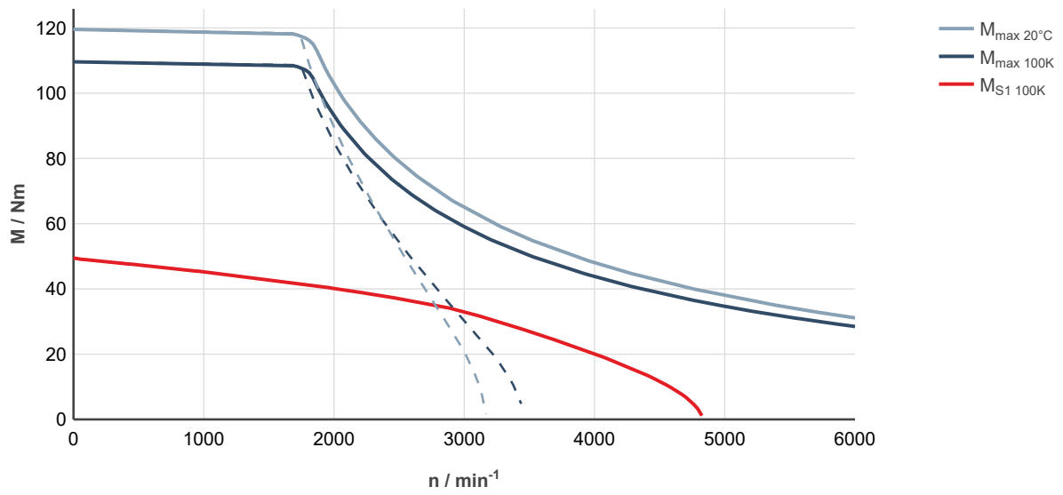
Fig. 153: MS2N07-E0BNA-___0-___-_, ctrIX DRIVE, uncontrolled supply 3 × AC 400 V
