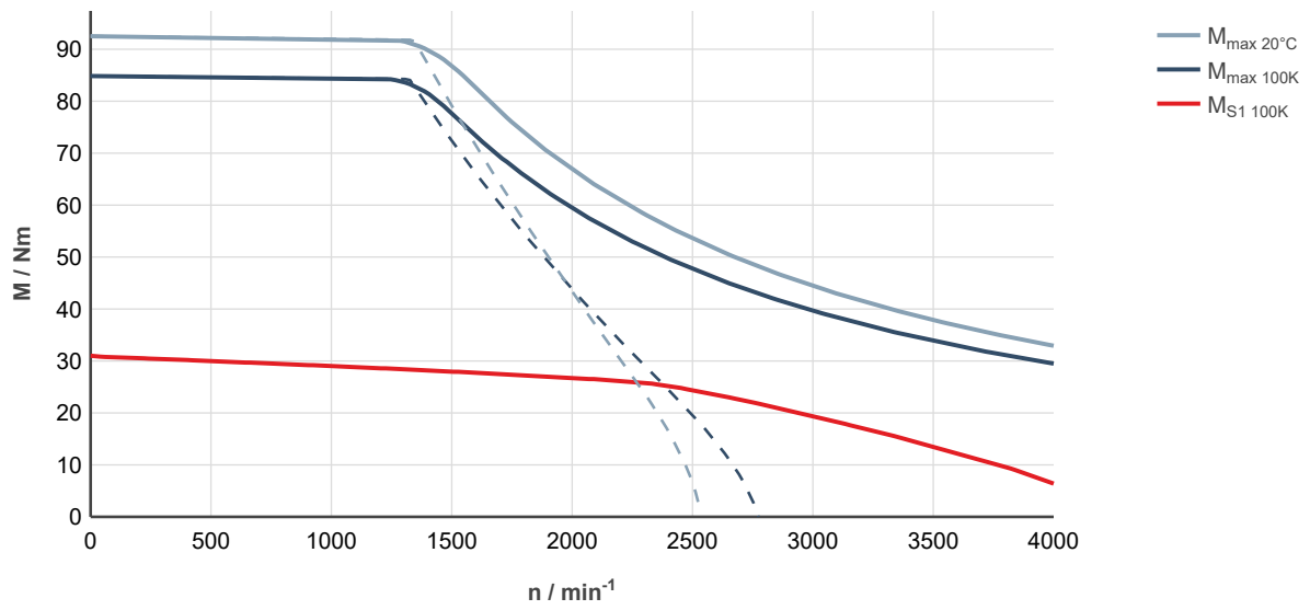
Fig. 145: MS2N07-D1BHA-___0-___-_, ctrlX DRIVE, uncontrolled supply 3 × AC 400 V
