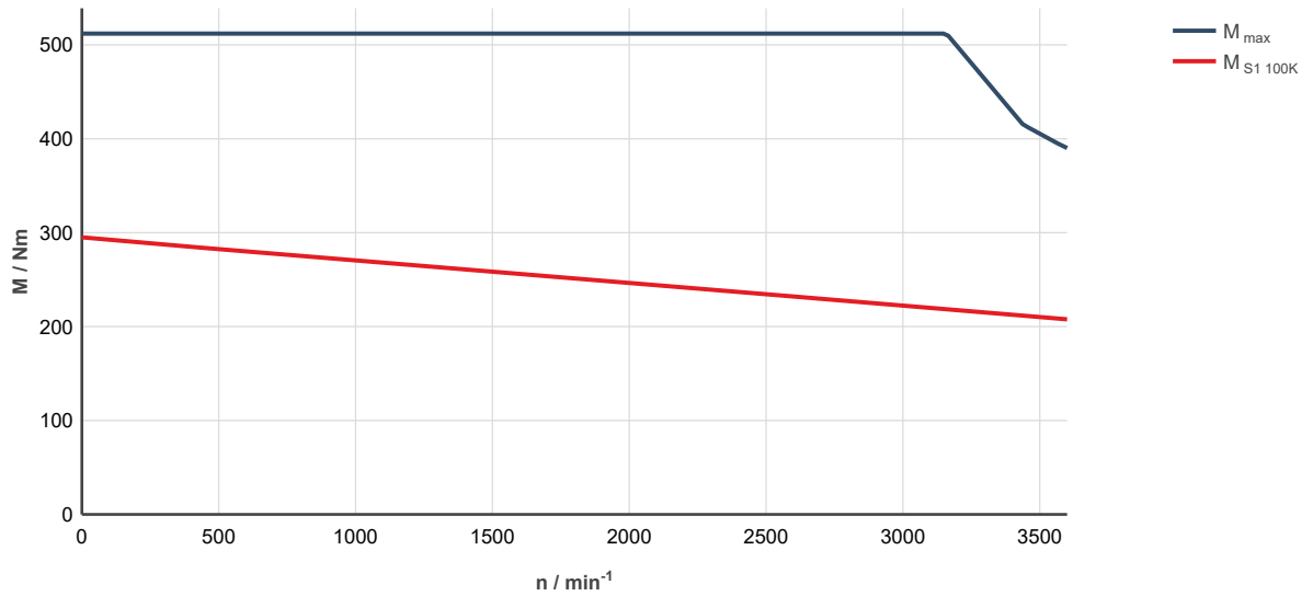
Fig. 345: MS2N13-D1BNL-___0-___-__, ctrlX DRIVE, controlled supply 3 x AC 400 ... 480 V
