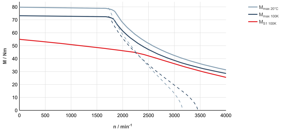
Fig. 170: MS2N07-D0BHL-___0-___-___, ctrIX DRIVE, controlled supply 3 × AC 400 ... 480 V
