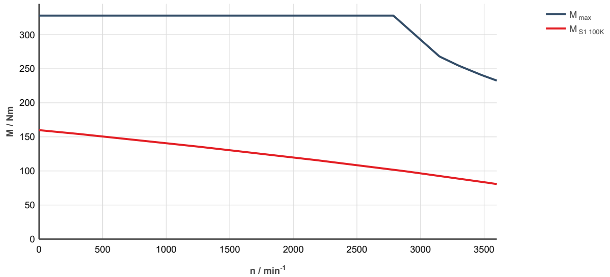
Fig. 321: MS2N13-B1BNC-___0-___-_, ctrlX DRIVE, controlled supply 3 x AC 400 ... 480 V
