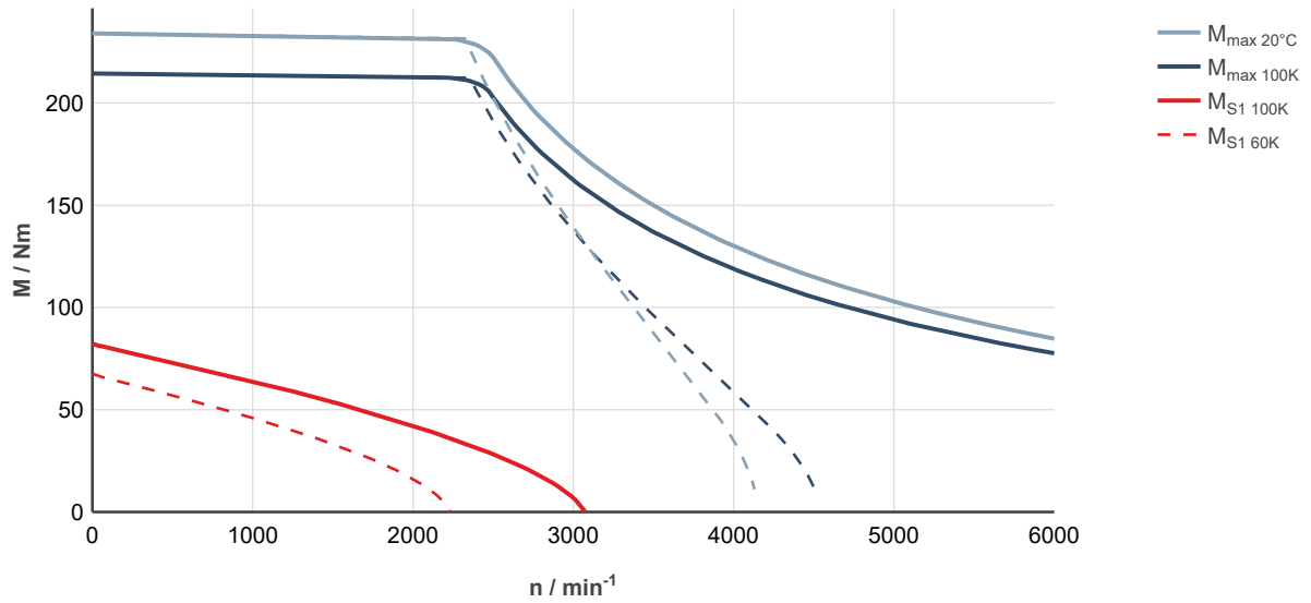
Fig. 213: MS2N10-E0BNN-___0-___-_, ctrlX DRIVE, controlled supply 3 × AC 400 ... 480 V
