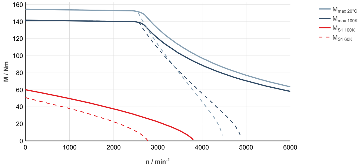
Fig. 205: MS2N10-D0BNN-___0-___-_, ctrlX DRIVE, controlled supply 3 × AC 400 ... 480 V
