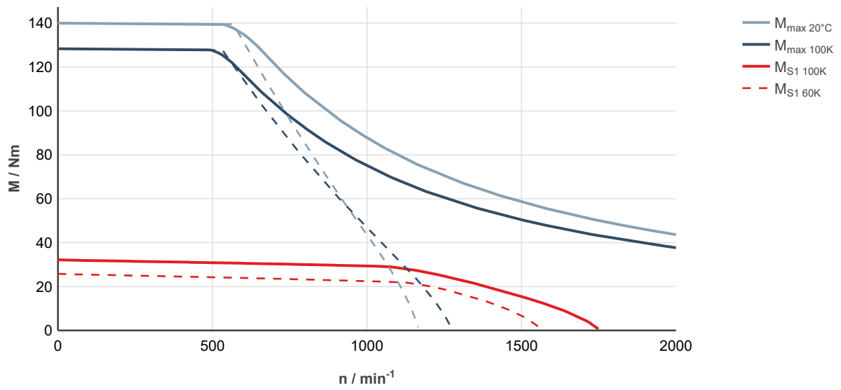
Fig. 121: MS2N07-E1BDN-___0-___-_, ctrlX DRIVE, uncontrolled supply 3 × AC 400 V
