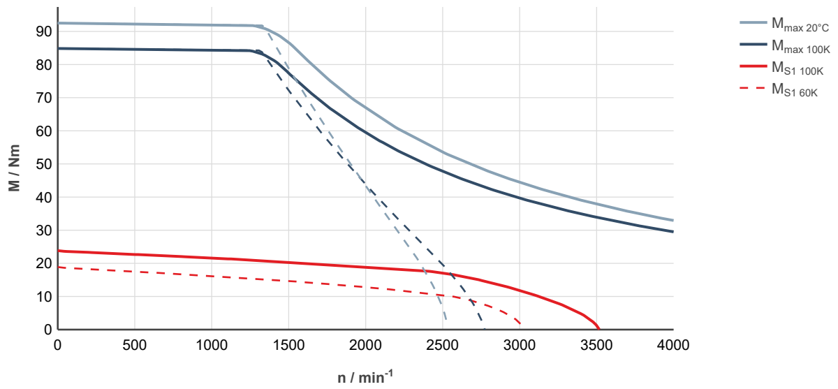
Fig. 109: MS2N07-D1BHN-___0-___-_, ctrlX DRIVE, uncontrolled supply 3 × AC 400 V
