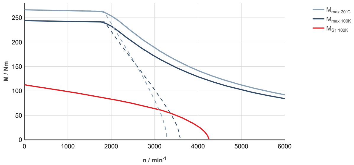
Fig. 250: MS2N10-E1BNA-___0-___-_, ctrIX DRIVE, uncontrolled supply 3 × AC 400 V
