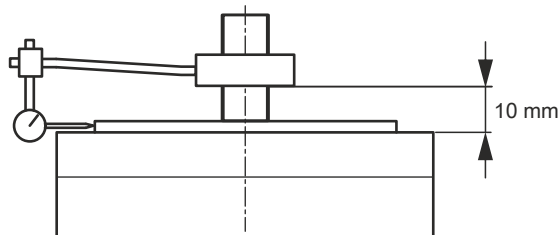
Fig. 14: Measuring system of coaxiality
