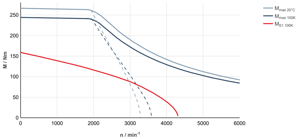
Fig. 278: MS2N10-E1BNL-__0-__-__, ctrlX DRIVE, uncontrolled supply 3 × AC 400 V
