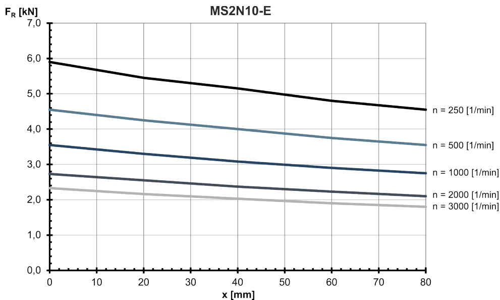
Fig. 299: MS2N10-E: Radial force in distance x from the shaft shoulder at a nominal bearing service life of L_{h10} = 30000 h
