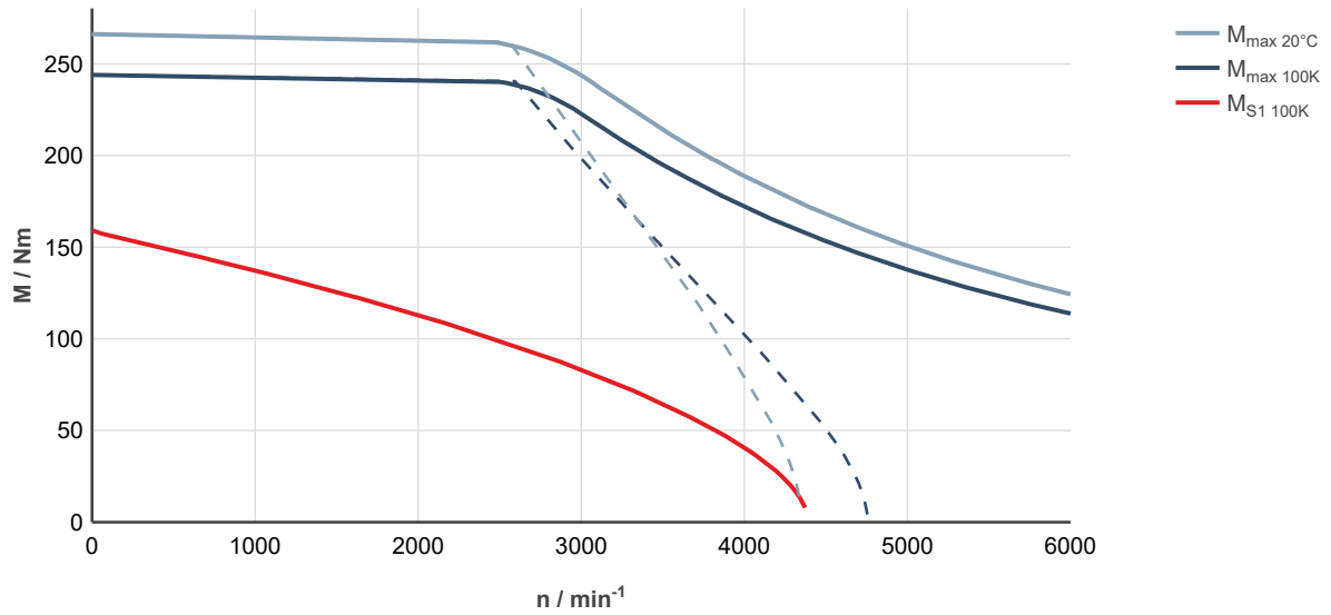
Fig. 279: MS2N10-E1BNL-__0-__-__, ctrlX DRIVE, controlled supply 3 × AC 400 ... 480 V
