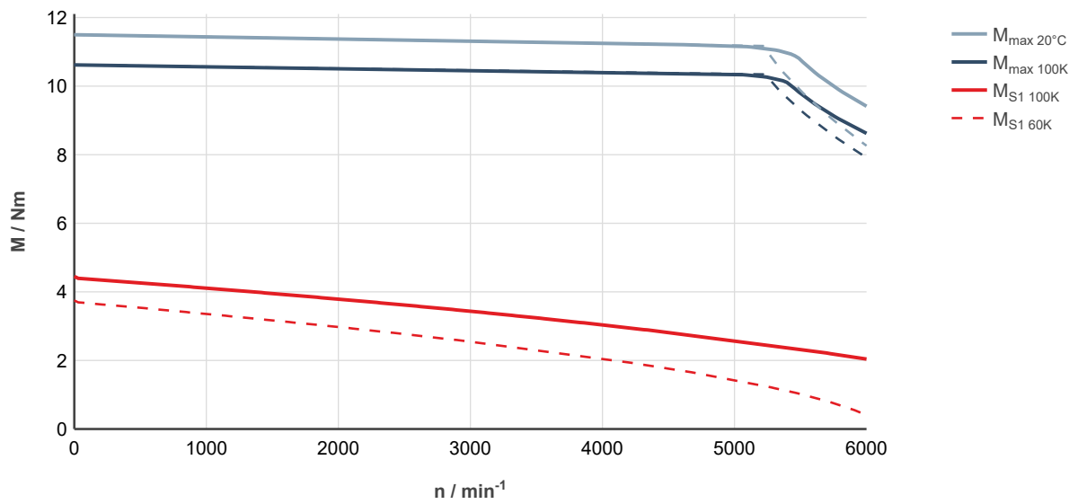
Fig. 54: MS2N05-B0BTN-___0-___-__, ctrlX DRIVE, controlled supply 3 × AC 400 ... 480 V
