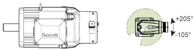
Fig. 370: Rotating area electrical connection “T”
