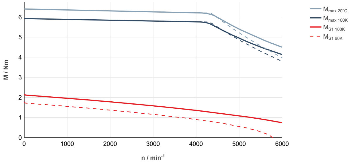
Fig. 37: MS2N04-B0BTN-___0-___-__, ctrlX DRIVE, controlled supply 3 × AC 400 ... 480 V
