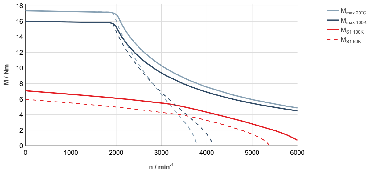
Fig. 70: MS2N06-C0BNN-___0-___-_, ctrlX DRIVE, uncontrolled supply 3 × AC 400 V
