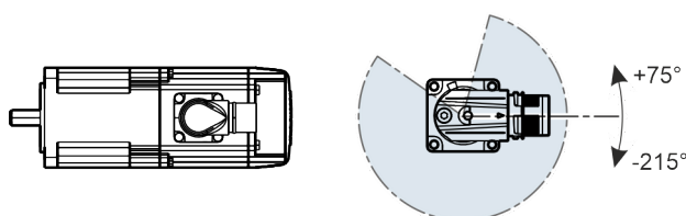
Fig. 377: Rotating area electrical connection "H"
