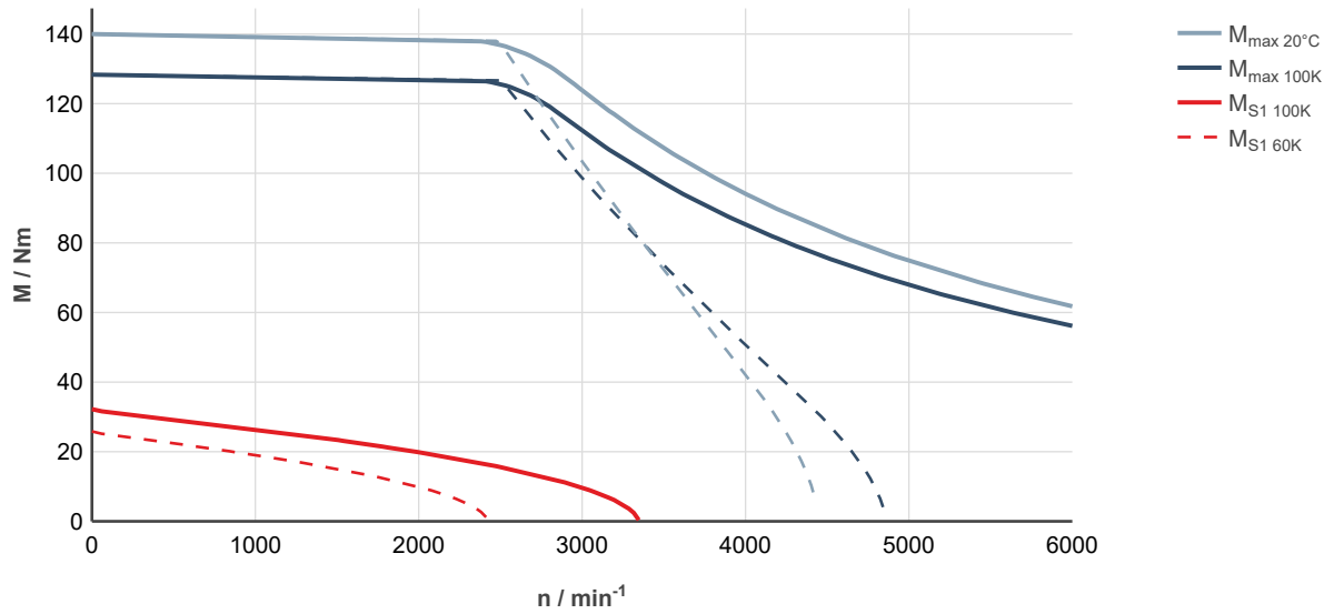
Fig. 126: MS2N07-E1BNN-___0-___-_, ctrlX DRIVE, controlled supply 3 × AC 400 ... 480 V
