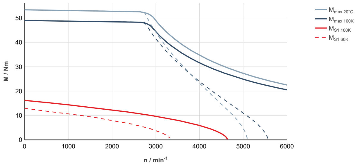
Fig. 82: MS2N06-E0BRN-___0-___-__, ctrlX DRIVE, uncontrolled supply 3 × AC 400 V
