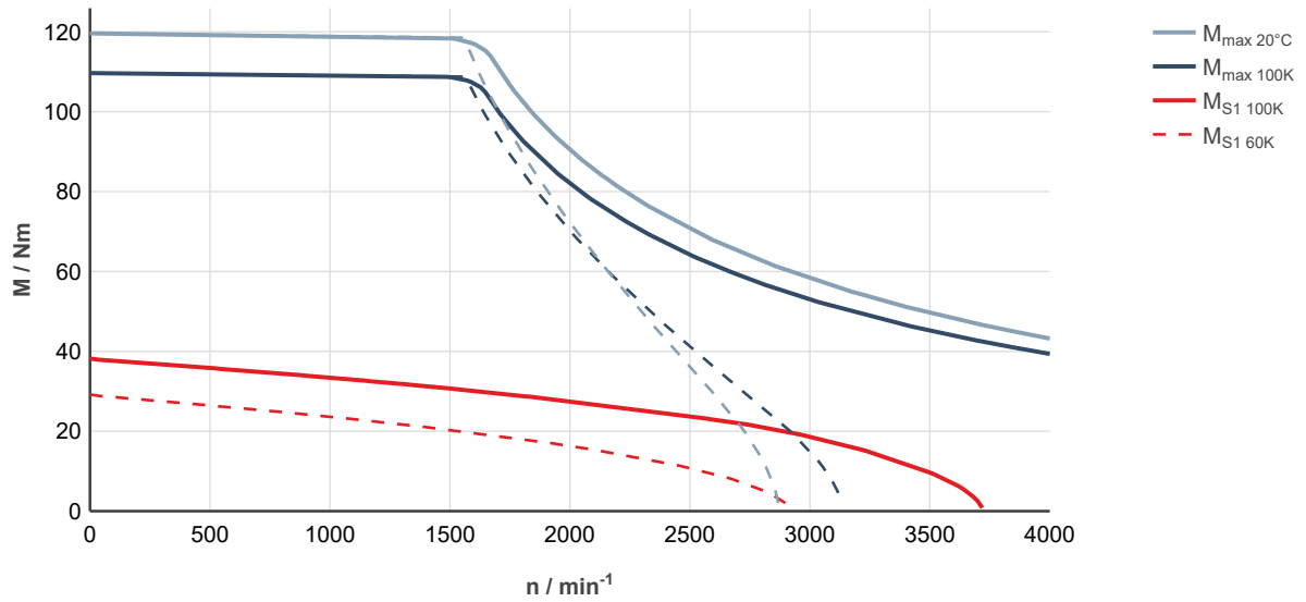
Fig. 116: MS2N07-E0BHN-___0-___-_, ctrlX DRIVE, controlled supply 3 × AC 400 ... 480 V
