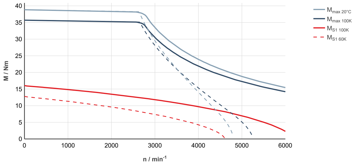
Fig. 93: MS2N07-C0BQN-___0-___-_, ctrlX DRIVE, uncontrolled supply 3 × AC 400 V
