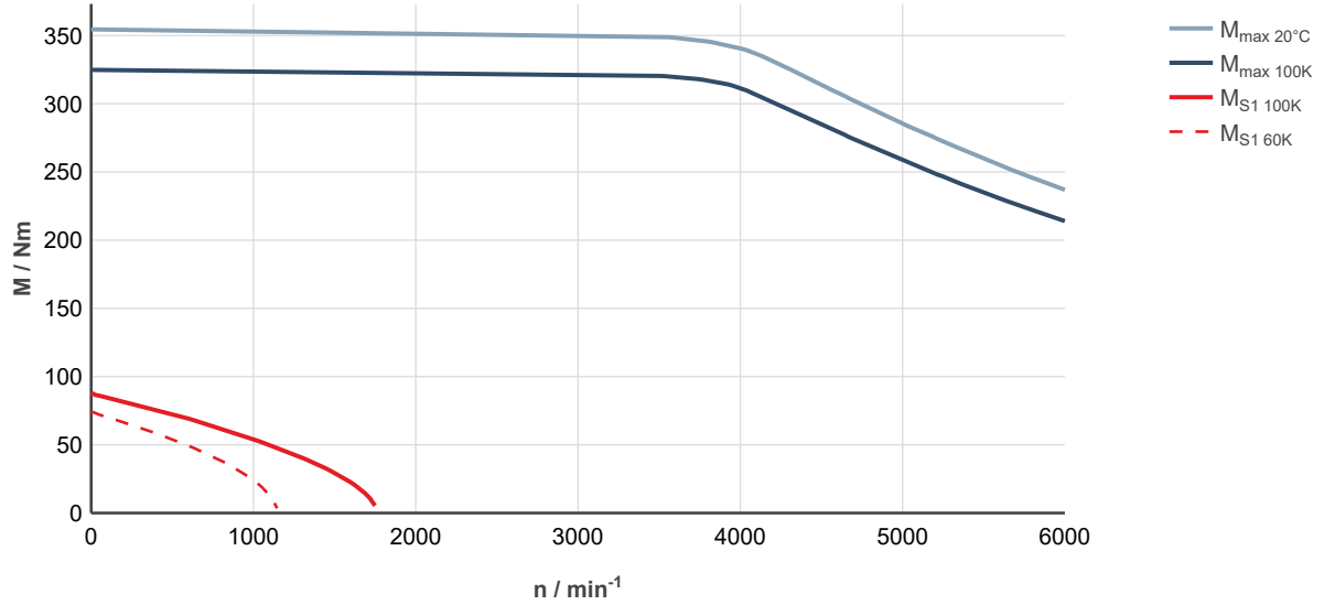
Fig. 227: MS2N10-R0BQN-___0-N___-, ctrlX DRIVE, controlled supply 3 x AC 400 ... 480 V
