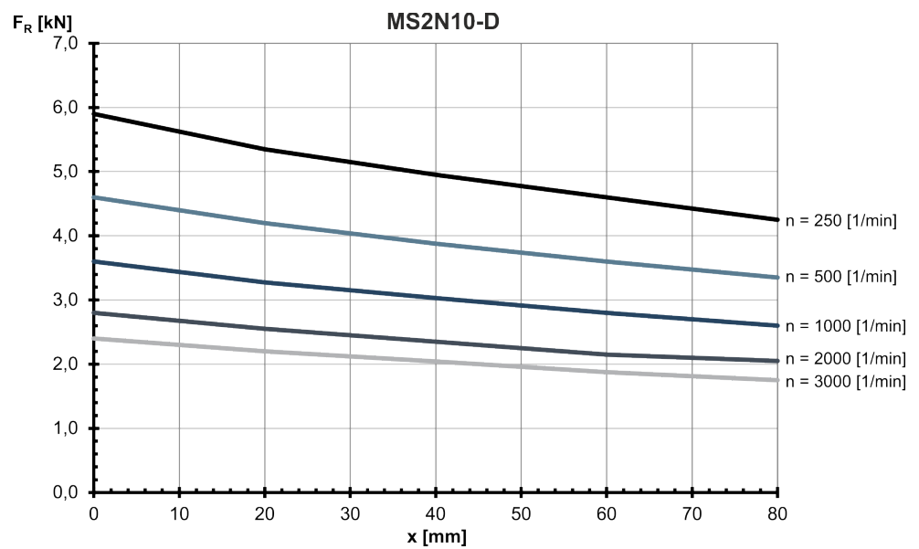
Fig. 298: MS2N10-D: Radial force in distance x from the shaft shoulder at a nominal bearing service life of L_{h10} = 30000 h
