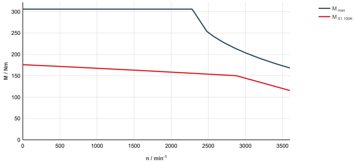
Fig. 335: MS2N13-B1BHL-__0-__-__, ctrlX DRIVE, controlled supply 3 x AC 400 ... 480 V
