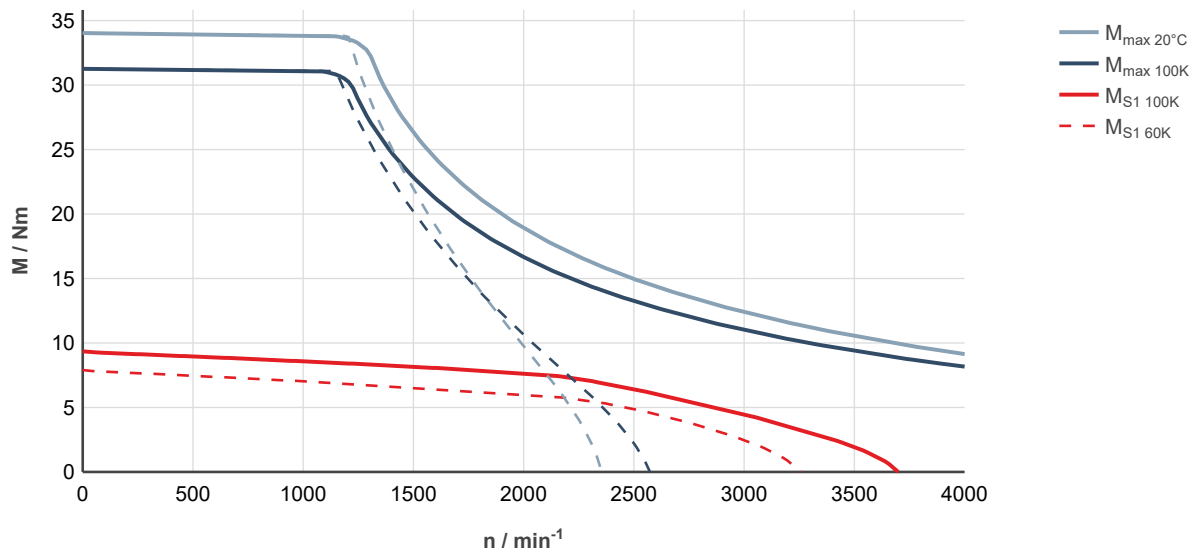
Fig. 59: MS2N05-D0BHN-___0-___-_, ctrlX DRIVE, uncontrolled supply 3 × AC 400 V
