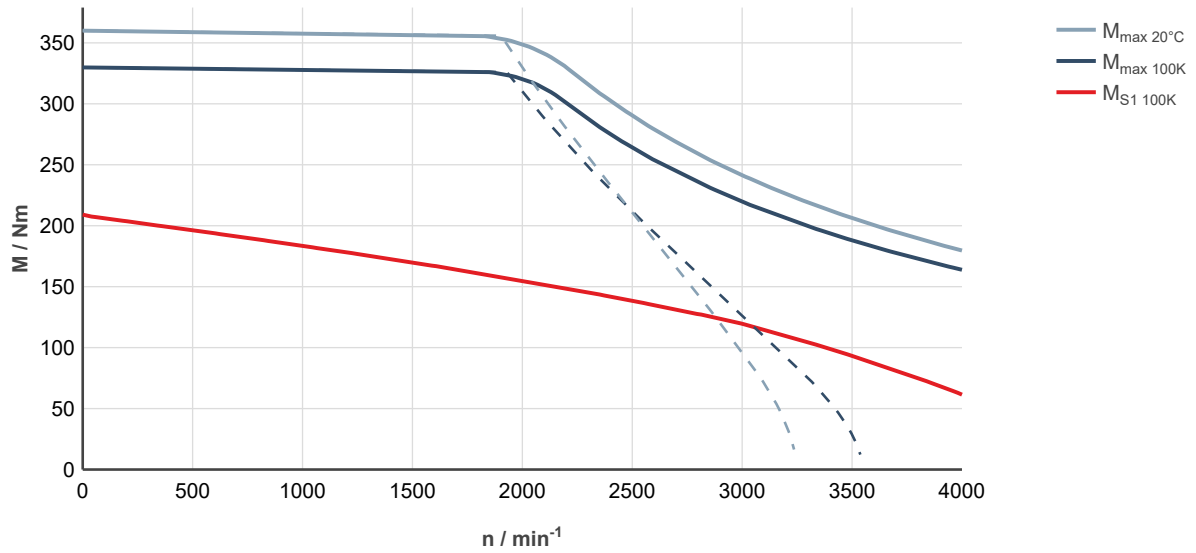
Fig. 285: MS2N10-F1BHL-___0-___-__, ctrlX DRIVE, controlled supply 3 × AC 400 ... 480 V
