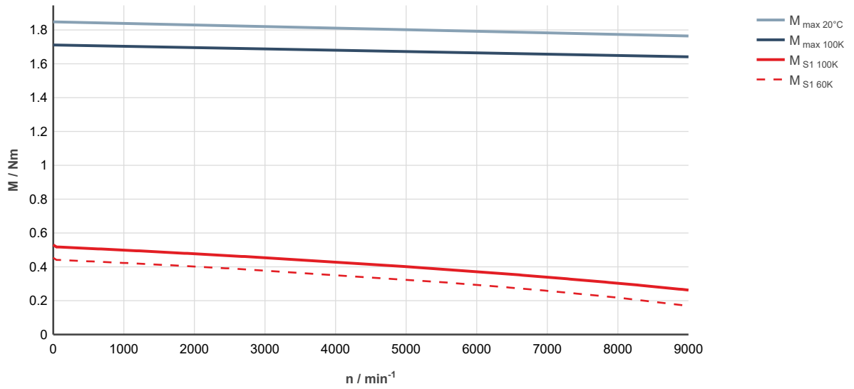
Fig. 24: MS2N03-A0BYN-___0-___-__, ctrlX DRIVE, controlled supply 3 x AC 400 ... 480 V
