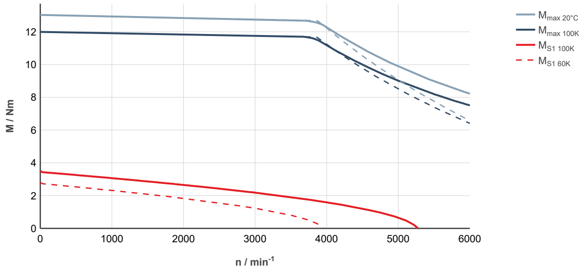
Fig. 41: MS2N04-C0BTN-___0-___-__, ctrlX DRIVE, controlled supply 3 × AC 400 ... 480 V
