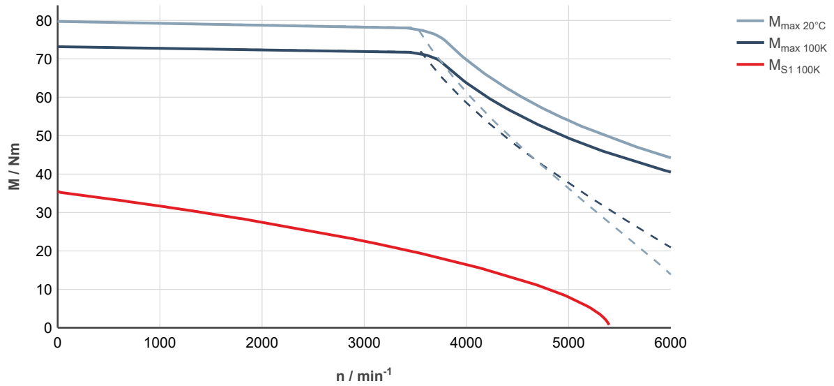
Fig. 142: MS2N07-D0BRA-___0-___-_, ctrlX DRIVE, controlled supply 3 × AC 400 ... 480 V
