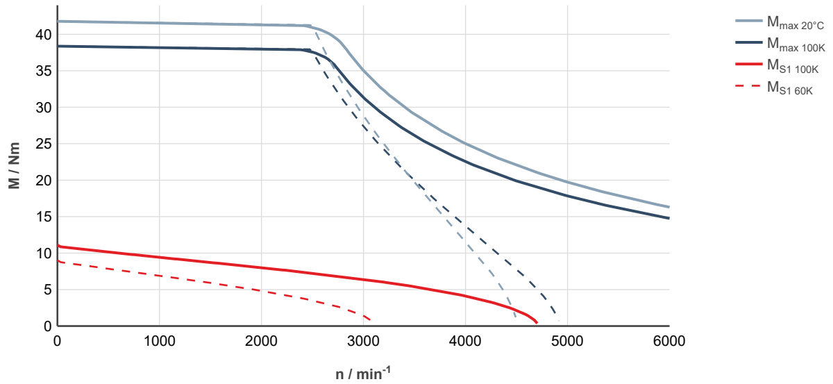
Fig. 79: MS2N06-D1BNN-___0-___-_, ctrlX DRIVE, controlled supply 3 × AC 400 ... 480 V
