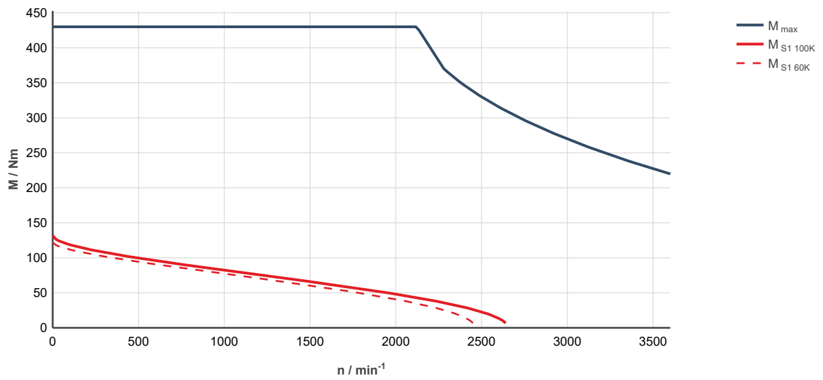
Fig. 308: MS2N13-C1BNN-___0-___-_, ctrlX DRIVE, uncontrolled supply 3 × AC 400 V
