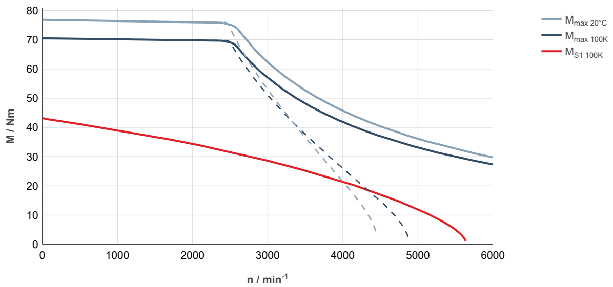
Fig. 231: MS2N10-C0BNA-___0-___-_, ctrlX DRIVE, controlled supply 3 × AC 400 ... 480 V
