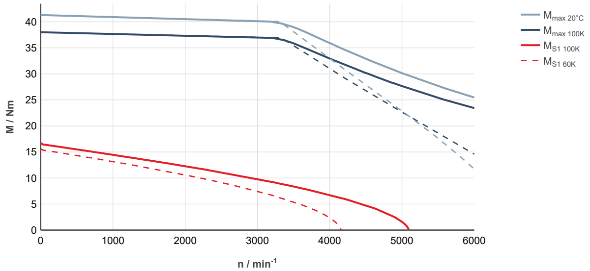
Fig. 193: MS2N10-B1BQN-___0-___-_, ctrlX DRIVE, controlled supply 3 × AC 400 ... 480 V
