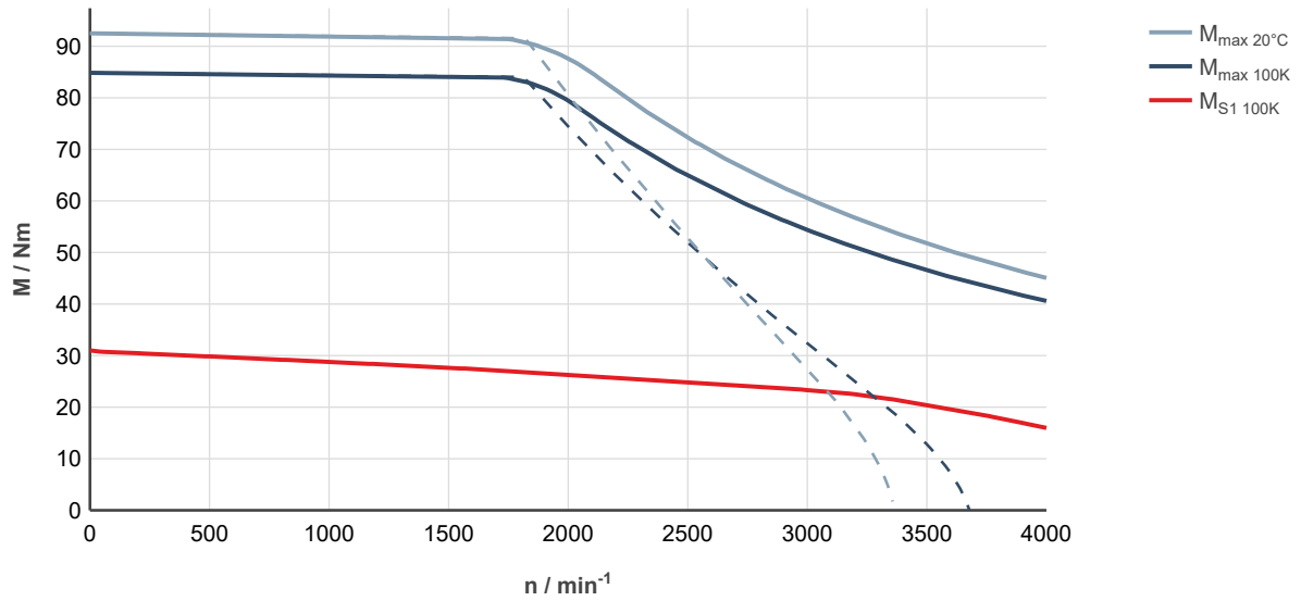
Fig. 146: MS2N07-D1BHA-___0-___-_, ctrlX DRIVE, controlled supply 3 × AC 400 ... 480 V
