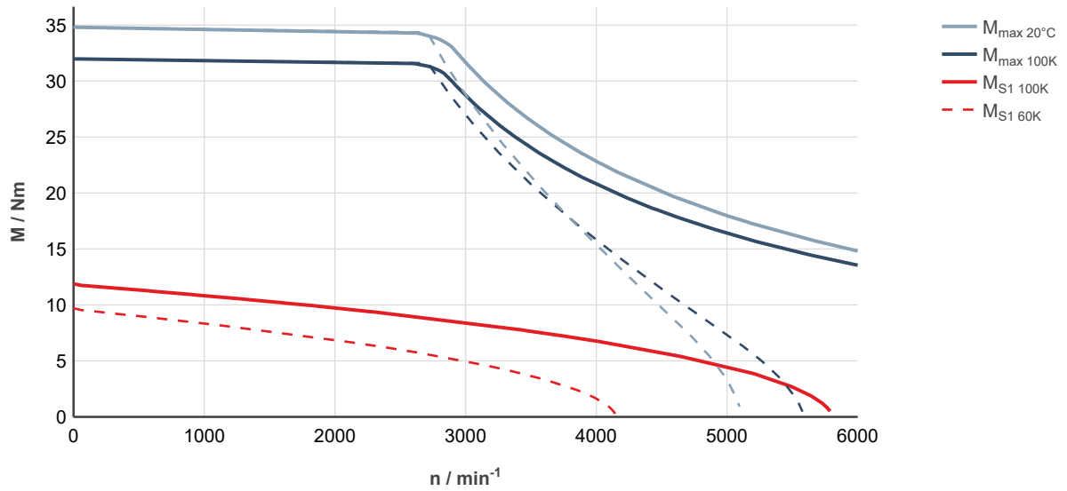
Fig. 75: MS2N06-D0BNN-___0-___-_, ctrlX DRIVE, controlled supply 3 × AC 400 ... 480 V
