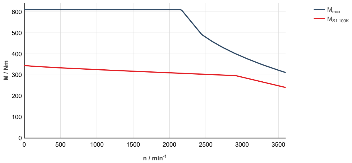
Fig. 348: MS2N13-E1BNL-___0-___-__, ctrlX DRIVE, uncontrolled supply 3 × AC 400 V
