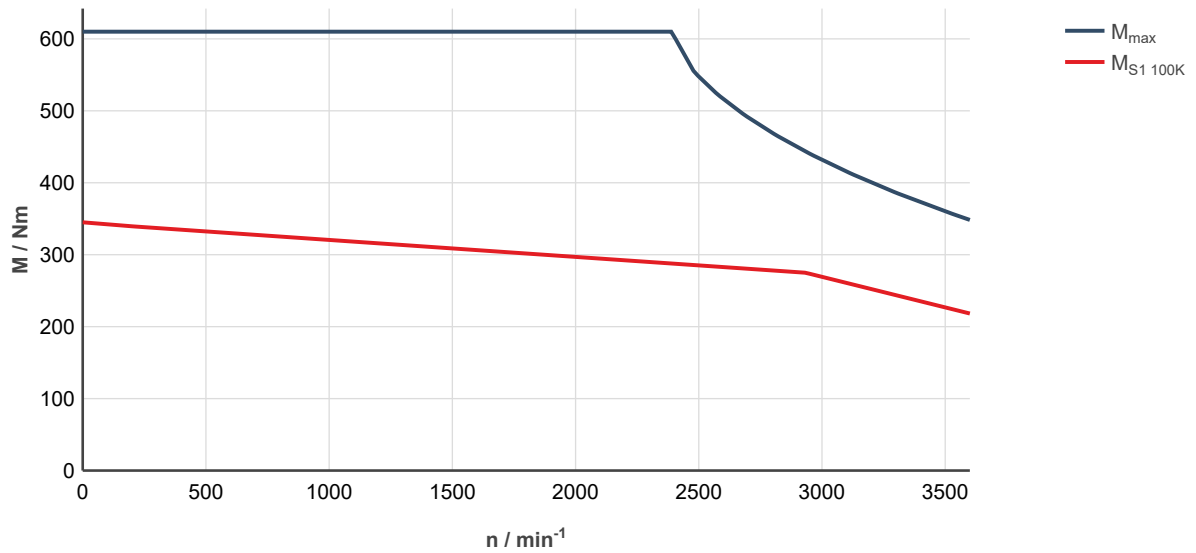
Fig. 347: MS2N13-E1BHL-___0-___-___, ctrlX DRIVE, controlled supply 3 × AC 400 ... 480 V M_{max} Characteristic curve applies to maximum torque 20 °C (cold)
