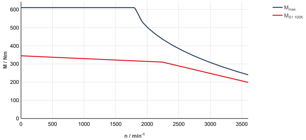
Fig. 346: MS2N13-E1BHL-___0-___-___, ctrlX DRIVE, uncontrolled supply 3 × AC 400 V M_{max} Characteristic curve applies to maximum torque 20 °C (cold)
