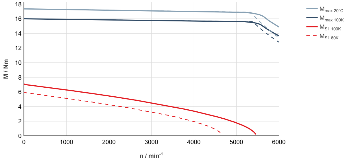
Fig. 73: MS2N06-C0BTN-___0-___-__, ctrlX DRIVE, controlled supply 3 × AC 400 ... 480 V
