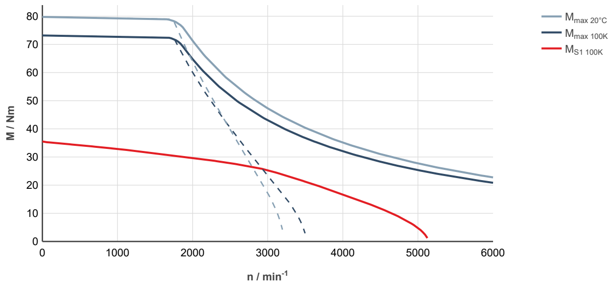
Fig. 139: MS2N07-D0BNA-___0-___-_, ctrlX DRIVE, uncontrolled supply 3 × AC 400 V
