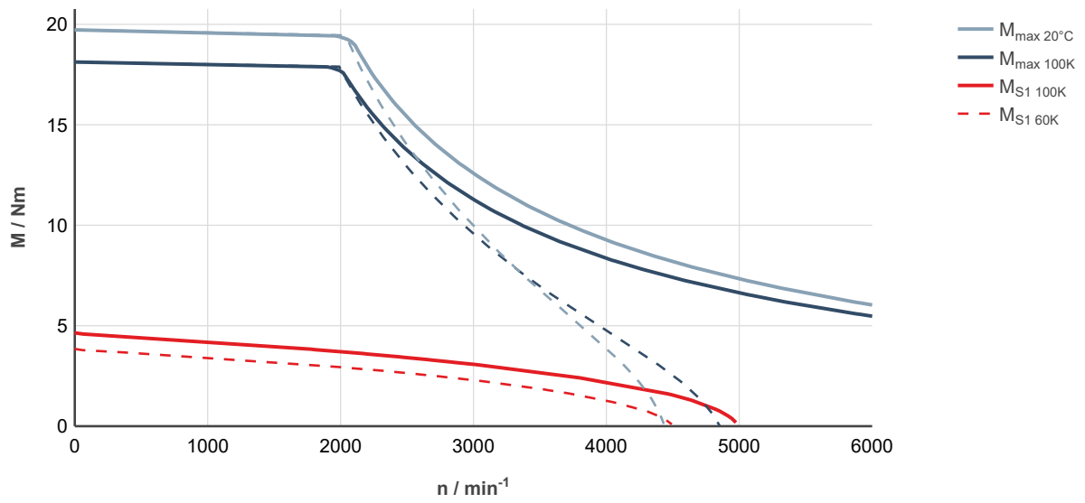
Fig. 44: MS2N04-D0BQN-___0-___-__, ctrlX DRIVE, uncontrolled supply 3 × AC 400 V
