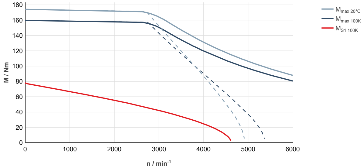
Fig. 243: MS2N10-D1BNA-___0-___-_, ctrlX DRIVE, controlled supply 3 × AC 400 ... 480 V
