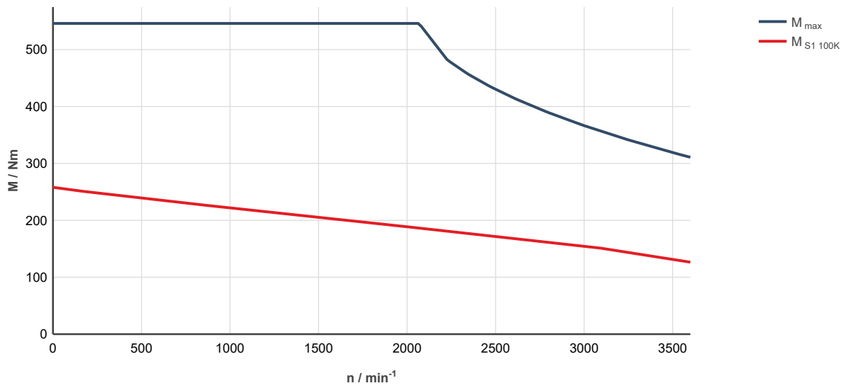
Fig. 328: MS2N13-D1BNC-___0-___-_, ctrlX DRIVE, uncontrolled supply 3 × AC 400 V
