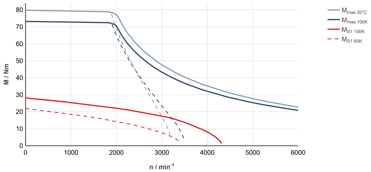
Fig. 103: MS2N07-D0BNN-___0-___-, ctrlX DRIVE, uncontrolled supply 3 × AC 400 V
