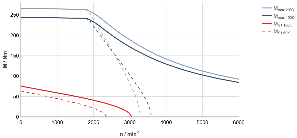
Fig. 216: MS2N10-E1BNN-___0-___-_, ctrlX DRIVE, uncontrolled supply 3 × AC 400 V
