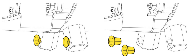
Fig. 395: Protective plug MS2N07, MS2N10 water cooling
