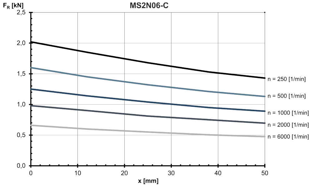
Fig. 86: MS2N06-C: Radial force in distance x from the shaft shoulder at a nominal bearing service life of L_{h10} = 30000 h
