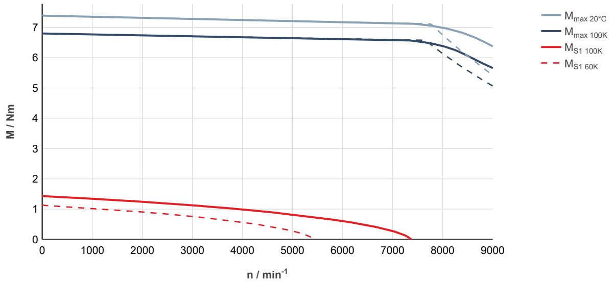
Fig. 28: MS2N03-D0BYN-___0-___-__, ctrlX DRIVE, controlled supply 3 × AC 400 ... 480 V
