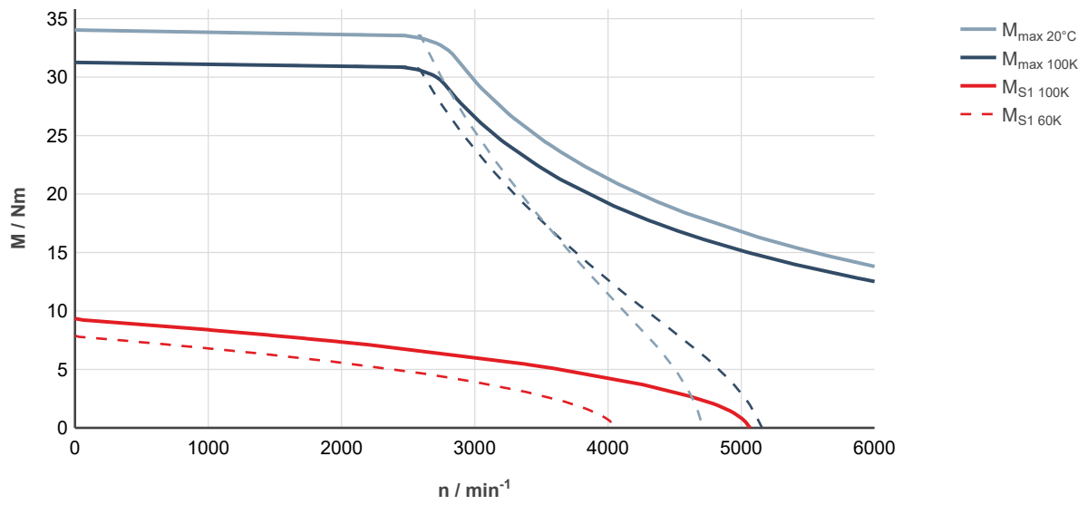
Fig. 61: MS2N05-D0BRN-___0-___-__, ctrlX DRIVE, uncontrolled supply 3 × AC 400 V
