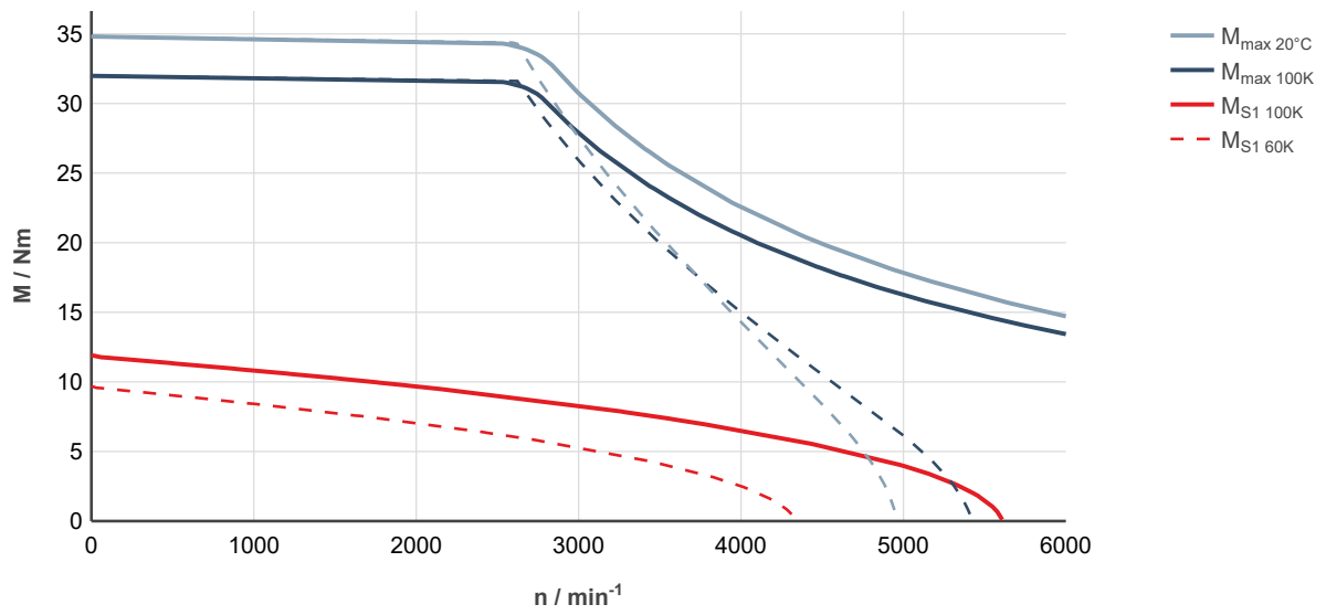
Fig. 76: MS2N06-D0BRN-___0-___-__, ctrlX DRIVE, uncontrolled supply 3 × AC 400 V
