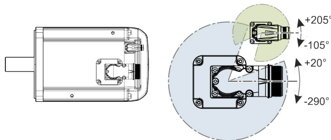
Fig. 383: : Rotating area electrical connection "V"
