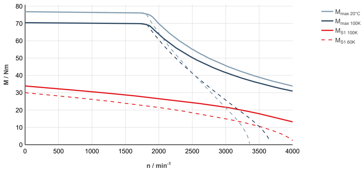
Fig. 195: MS2N10-C0BHN-___0-___-_, ctrlX DRIVE, controlled supply 3 × AC 400 ... 480 V
