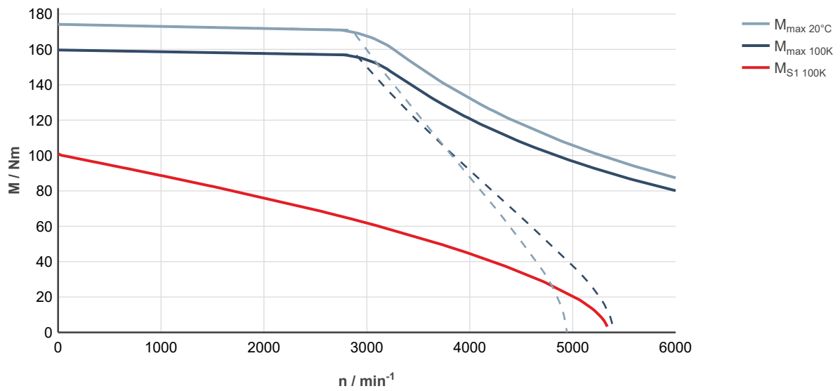
Fig. 273: MS2N10-D1BNL-___0-___-___, ctrIX DRIVE, controlled supply 3 × AC 400 ... 480 V
