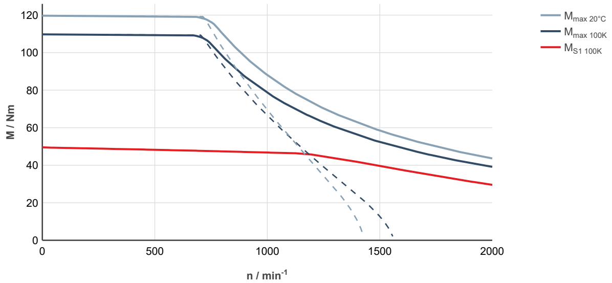
Fig. 150: MS2N07-E0BDA-___0-___-__, ctrlX DRIVE, controlled supply 3 × AC 400 ... 480 V
