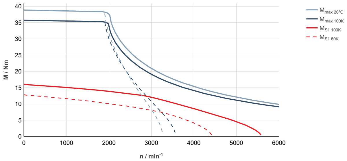
Fig. 91: MS2N07-C0BNN-___0-___-_, ctrlX DRIVE, uncontrolled supply 3 × AC 400 V
