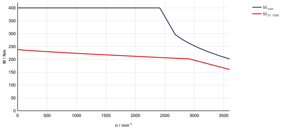
Fig. 339: MS2N13-C1BHL-___0-___-__, ctrlX DRIVE, controlled supply 3 × AC 400 ... 480 V M_{\text{max}} Characteristic curve applies to maximum torque 20 °C (cold)
