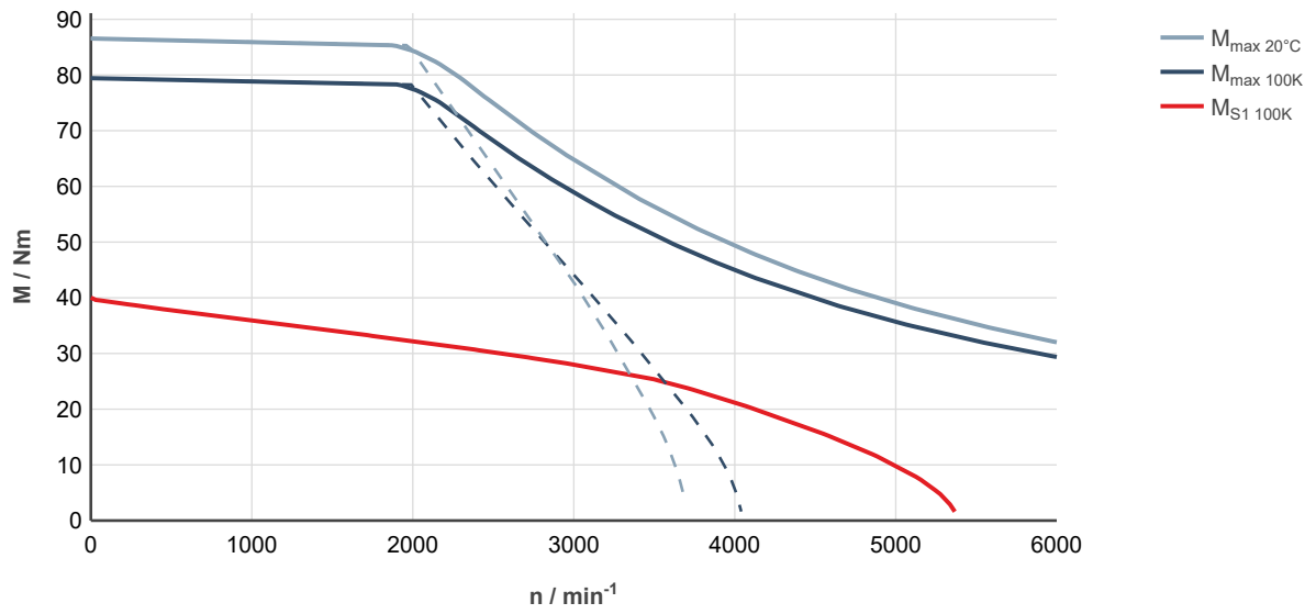
Fig. 234: MS2N10-C1BNA-___0-___-_, ctrlX DRIVE, uncontrolled supply 3 × AC 400 V
