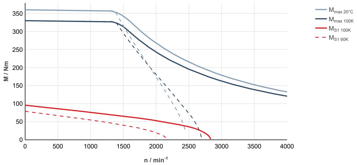
Fig. 224: MS2N10-F1BHN-___0-___-_, ctrlX DRIVE, uncontrolled supply 3 × AC 400 V
