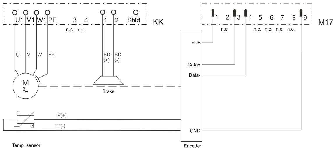
Fig. 362: Double cable connection terminal boxes, digital encoder C and D, brake optional
