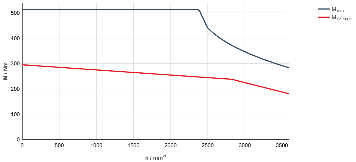
Fig. 344: MS2N13-D1BNL-___0-___-__, ctrlX DRIVE, uncontrolled supply 3 × AC 400 V
