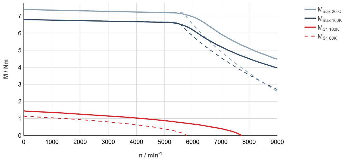
Fig. 27: MS2N03-D0BYN-___0-___-__, ctrlX DRIVE, uncontrolled supply 3 × AC 400 V
