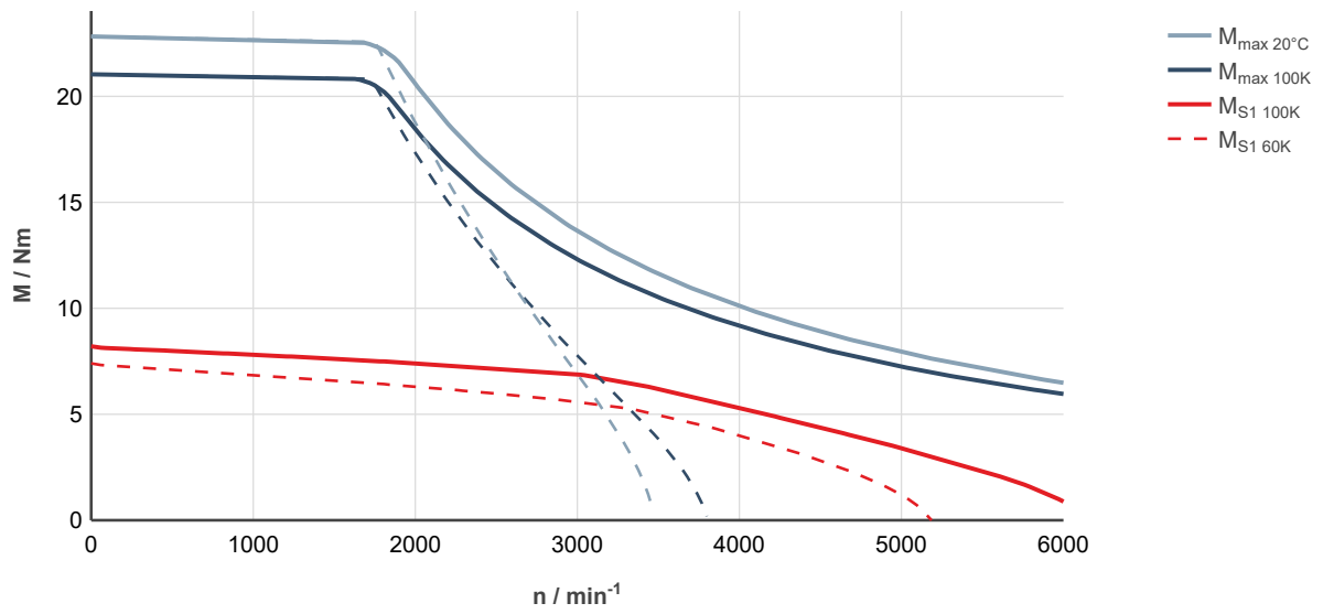
Fig. 89: MS2N07-B1BNN-___0-___-__, ctrlX DRIVE, uncontrolled supply 3 × AC 400 V
