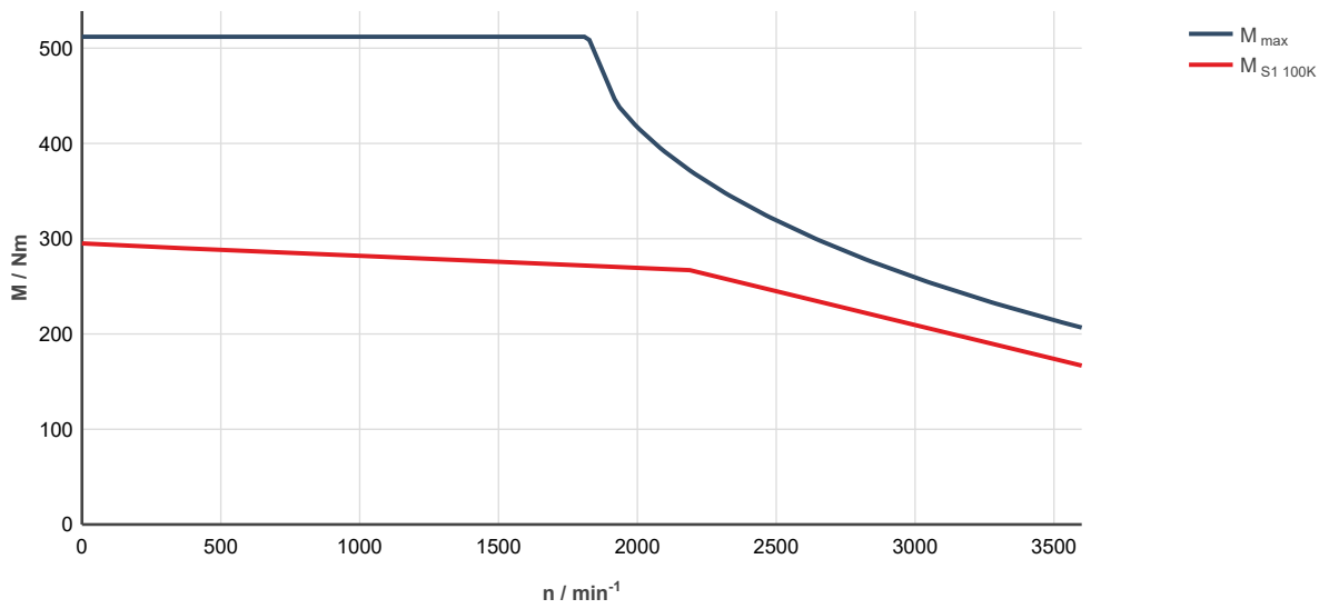
Fig. 342: MS2N13-D1BHL-__0-__-__, ctrlX DRIVE, uncontrolled supply 3 × AC 400 V
