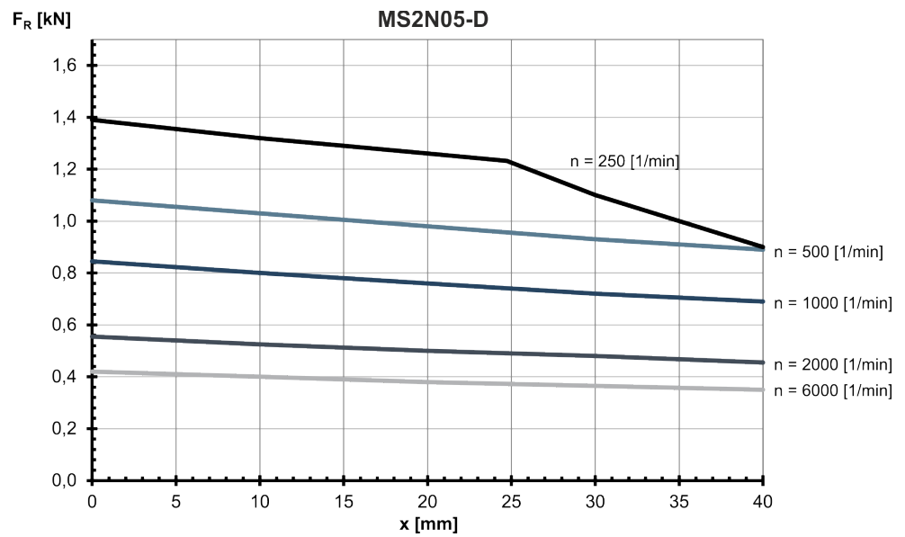
Fig. 67: MS2N05-D: Radial force in distance x from the shaft shoulder at a nominal bearing service life of L_{h10} = 30000 h
