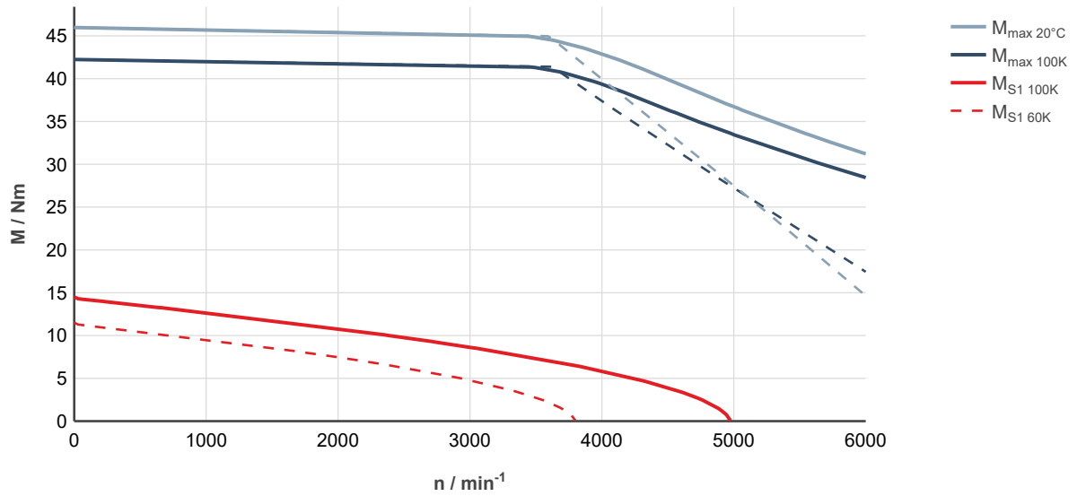
Fig. 98: MS2N07-C1BRN-___0-___-__, ctrlX DRIVE, controlled supply 3 × AC 400 ... 480 V
