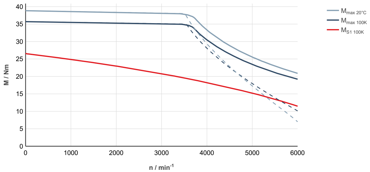
Fig. 166: MS2N07-C0BQL-___0-___-__, ctrlX DRIVE, controlled supply 3 × AC 400 ... 480 V
