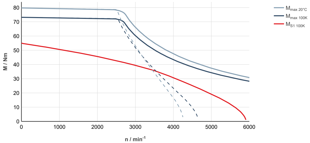
Fig. 172: MS2N07-D0BNL-__0-__-__, ctrlX DRIVE, controlled supply 3 × AC 400 ... 480 V
