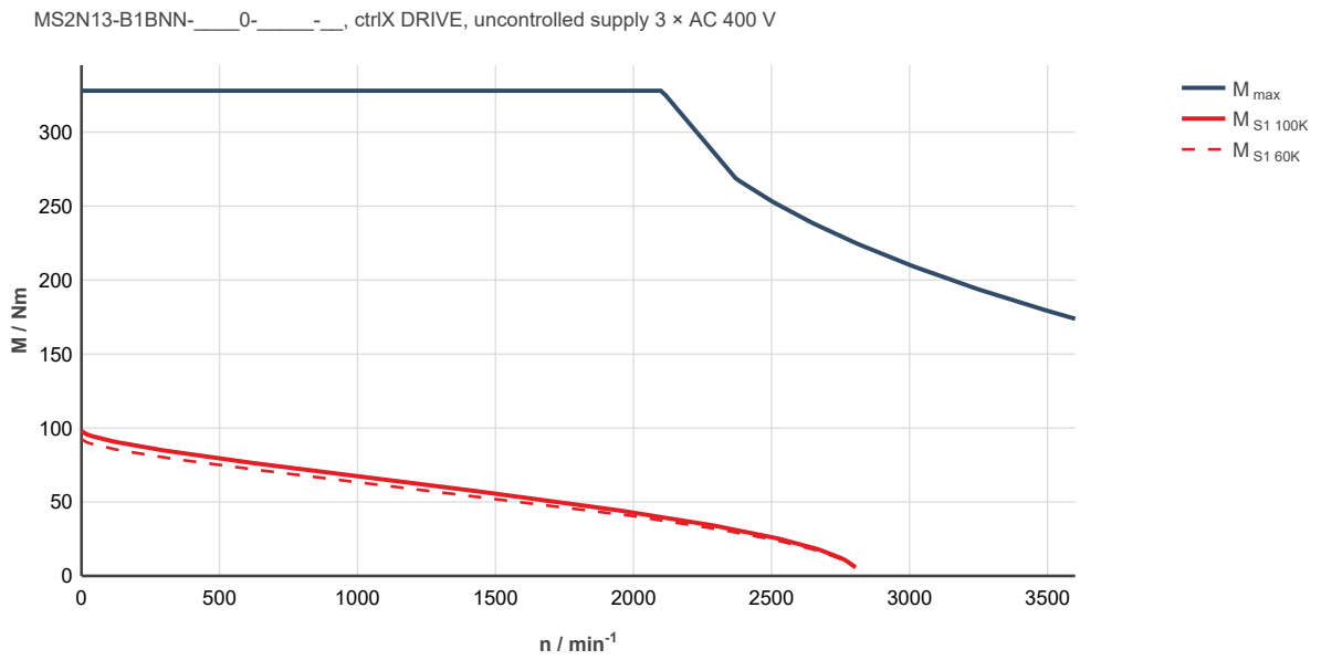
Fig. 304: MS2N13-B1BNN-___0-___-___, ctrlX DRIVE, uncontrolled supply 3 × AC 400 V
