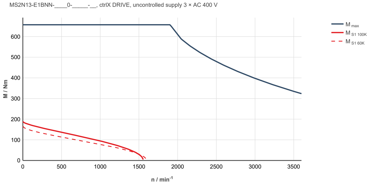
Fig. 316: MS2N13-E1BNN-___0-___-___, ctrlX DRIVE, uncontrolled supply 3 × AC 400 V
