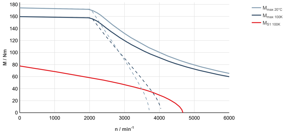
Fig. 242: MS2N10-D1BNA-___0-___-_, ctrlX DRIVE, uncontrolled supply 3 × AC 400 V
