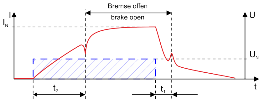
Fig. 7: Switching times of static hold mode t 1 Connection time (close) t 2 Disconnection time (open)
