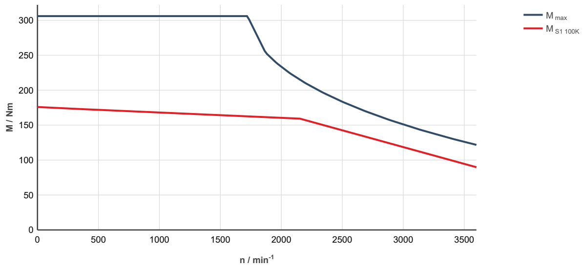
Fig. 334: MS2N13-B1BHL-__0-__-__, ctrlX DRIVE, uncontrolled supply 3 × AC 400 V
