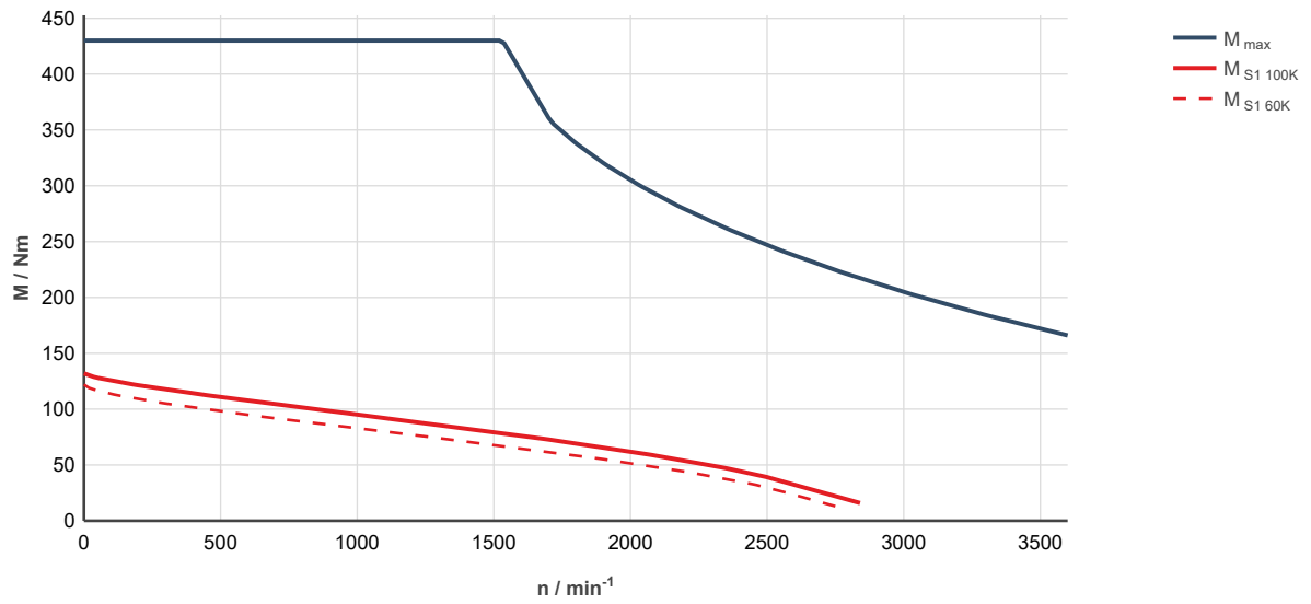
Fig. 306: MS2N13-C1BHN-___0-___-_, ctrlX DRIVE, uncontrolled supply 3 × AC 400 V
