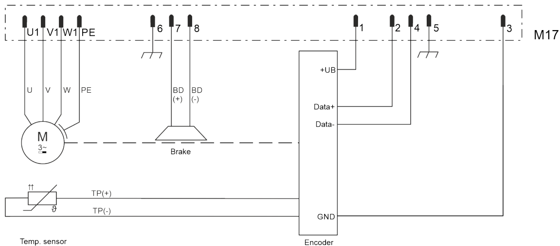
Fig. 357: M17 Single cable connection, digital encoder C, D, H, optional brake
