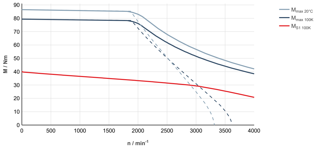
Fig. 233: MS2N10-C1BHA-___0-___-_, ctrIX DRIVE, controlled supply 3 x AC 400 ... 480 V
