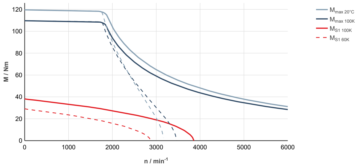
Fig. 117: MS2N07-E0BNN-___0-___-_, ctrlX DRIVE, uncontrolled supply 3 × AC 400 V
