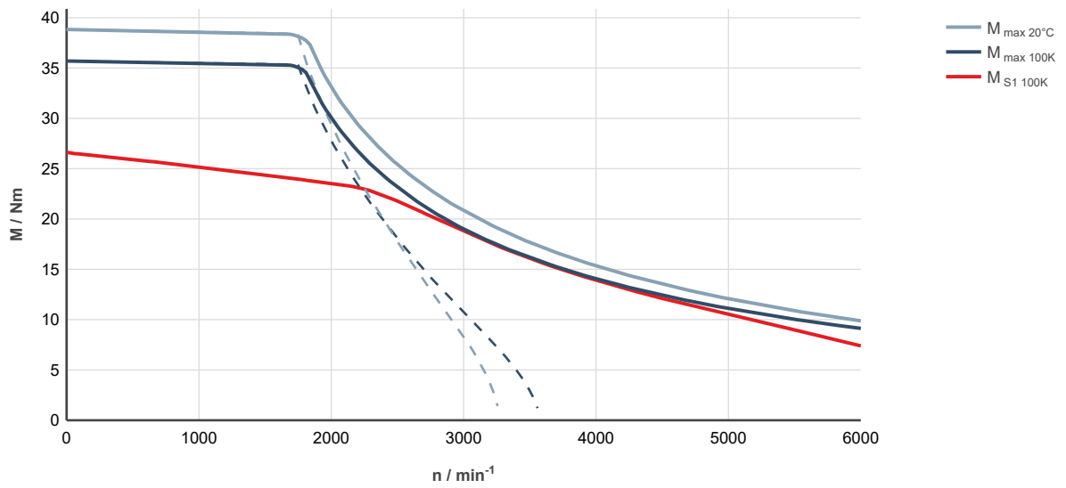
Fig. 163: MS2N07-C0BNL-___0-___-___, ctrIX DRIVE, uncontrolled supply 3 x AC 400 V
