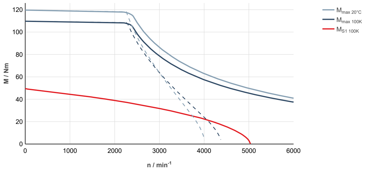
Fig. 155: MS2N07-E0BQA-___0-___-_, ctrlX DRIVE, uncontrolled supply 3 × AC 400 V
