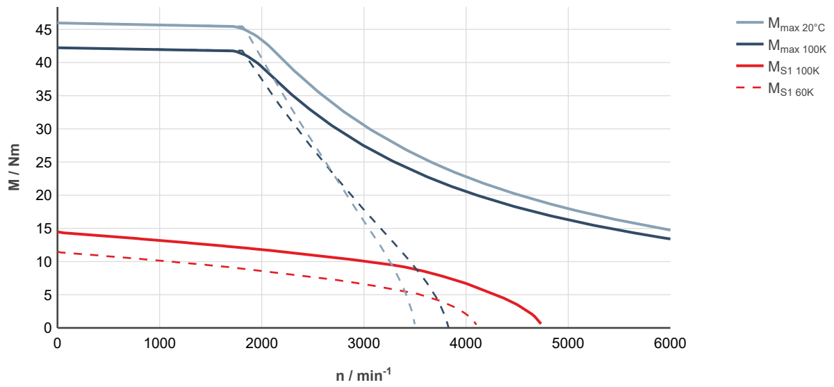
Fig. 95: MS2N07-C1BNN-___0-___-__, ctrlX DRIVE, uncontrolled supply 3 × AC 400 V
