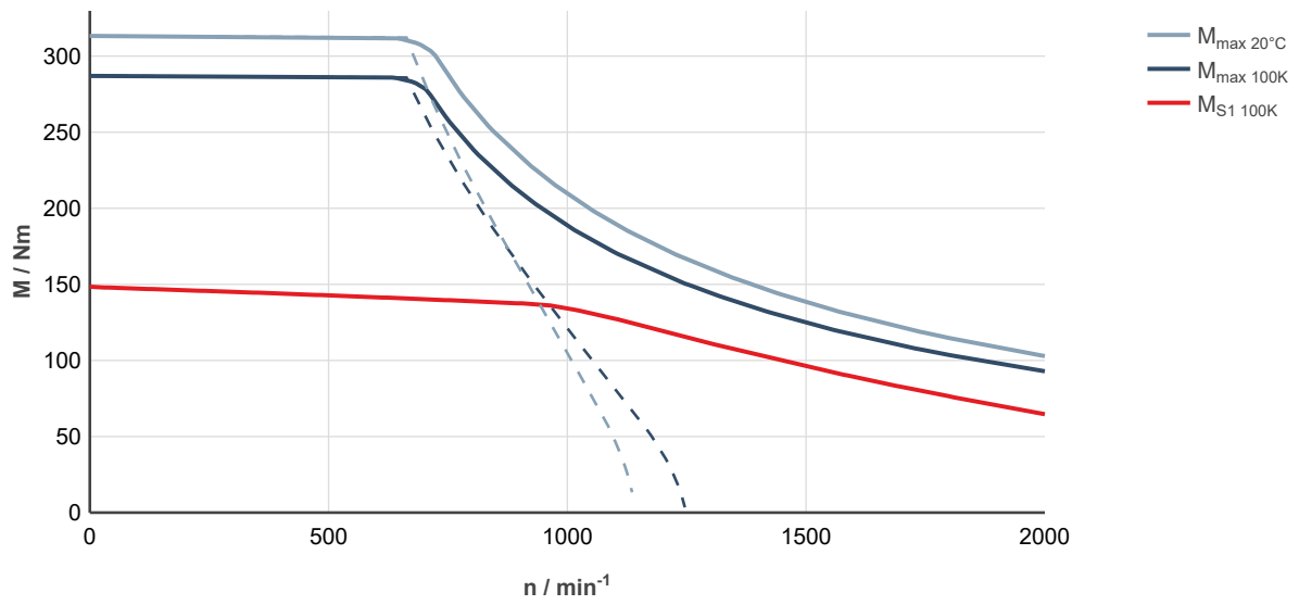
Fig. 252: MS2N10-F0BDA-___0-___-_, ctrlX DRIVE, uncontrolled supply 3 × AC 400 V
