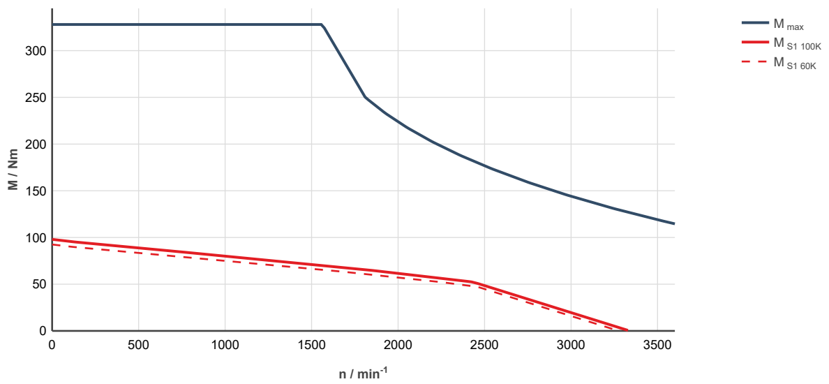
Fig. 302: MS2N13-B1BHN-___0-___-__ (modified), ctrlX DRIVE, uncontrolled supply 3 × AC 400 V
