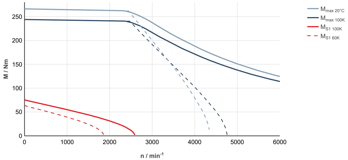
Fig. 217: MS2N10-E1BNN-___0-___-_, ctrlX DRIVE, controlled supply 3 × AC 400 ... 480 V
