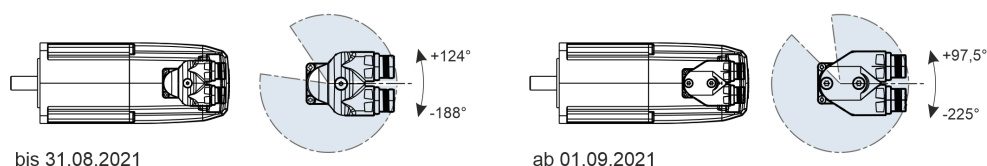
Fig. 375: Rotating area electrical connection "D"
