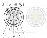
Fig. 374: Connector view double plug M17 power
