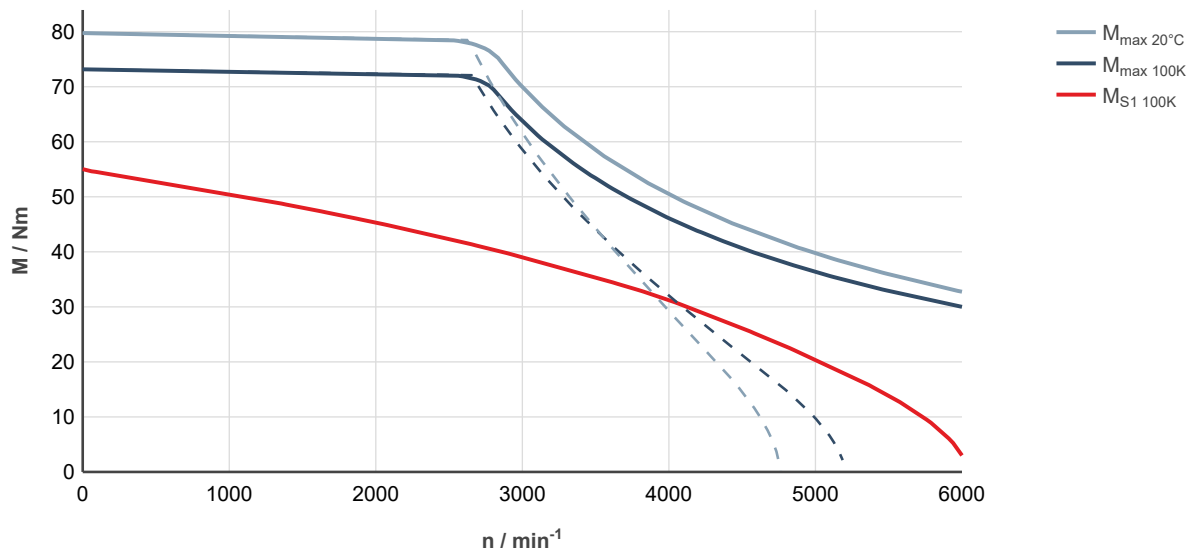
Fig. 173: MS2N07-D0BRL-___0-___-___, ctrlX DRIVE, uncontrolled supply 3 × AC 400 V
