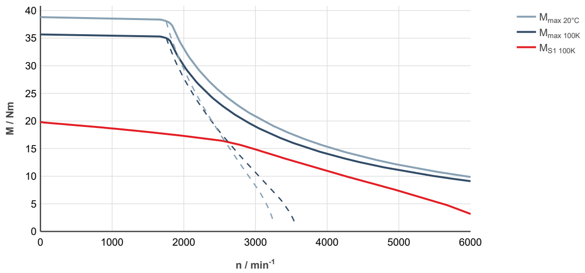
Fig. 127: MS2N07-C0BNA-___0-___-_, ctrlX DRIVE, uncontrolled supply 3 × AC 400 V
