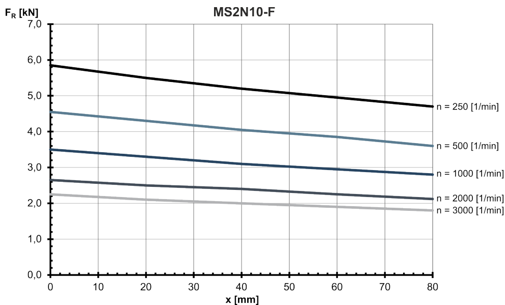
Fig. 300: MS2N10-F: Radial force in distance x from the shaft shoulder at a nominal bearing service life of L_{h10} = 30000 h
