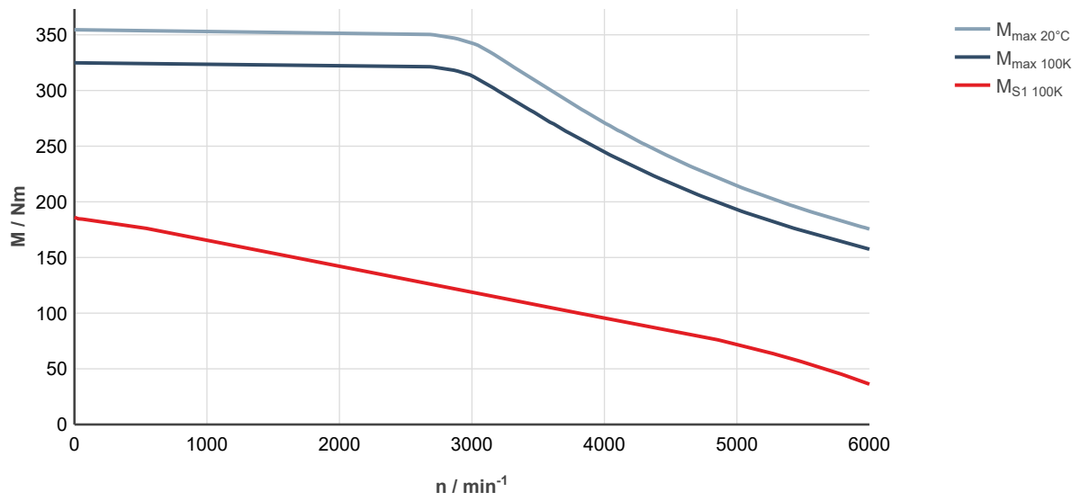
Fig. 288: MS2N10-R0BQL-__0-__-__, ctrlX DRIVE, uncontrolled supply 3 × AC 400 V
