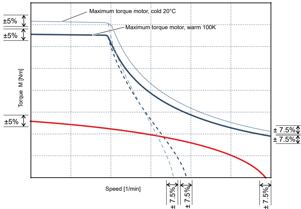
Fig. 21: Temperature influence and tolerances
