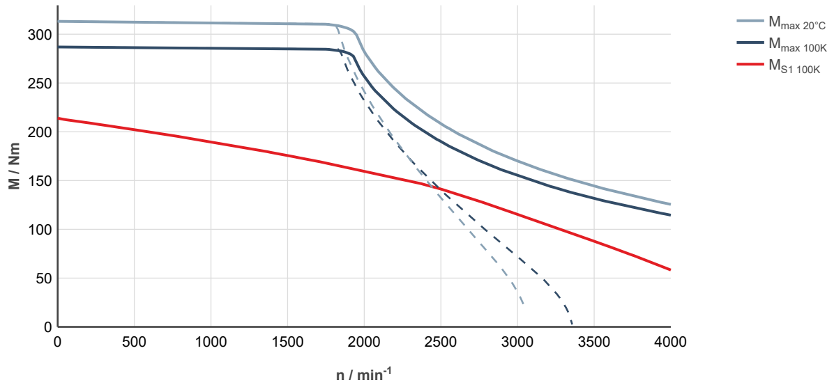
Fig. 281: MS2N10-F0BHL-___0-___-__, ctrlX DRIVE, controlled supply 3 × AC 400 ... 480 V
