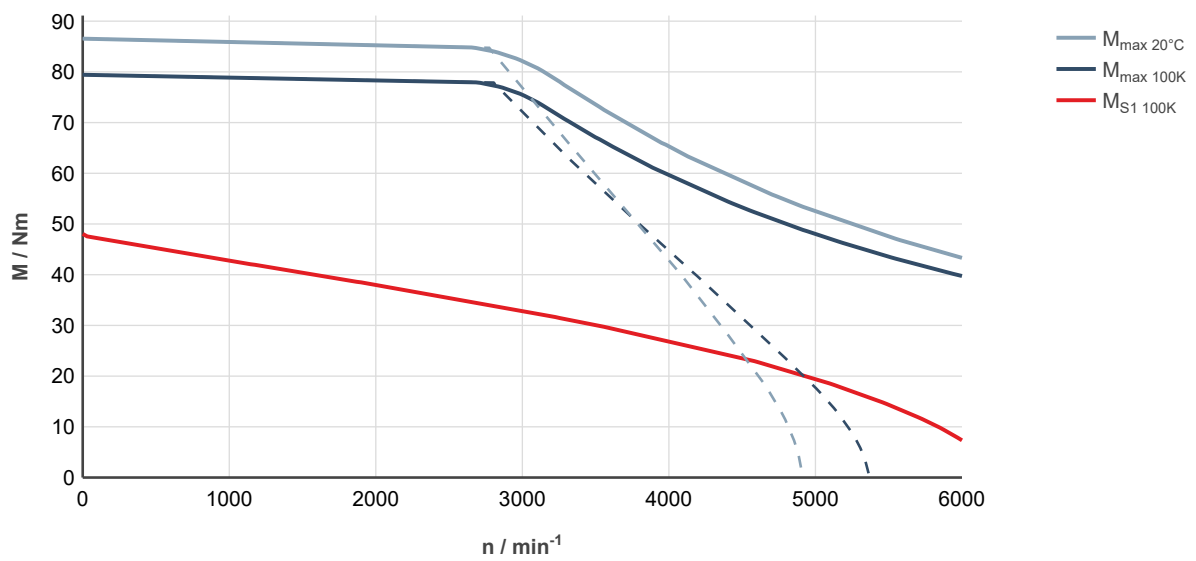
Fig. 267: MS2N10-C1BNL-___0-___-___, ctrIX DRIVE, controlled supply 3 × AC 400 ... 480 V
