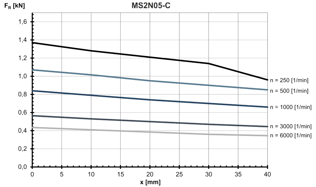
Fig. 66: MS2N05-C: Radial force in distance x from the shaft shoulder at a nominal bearing service life of L_{h10} = 30000 h
