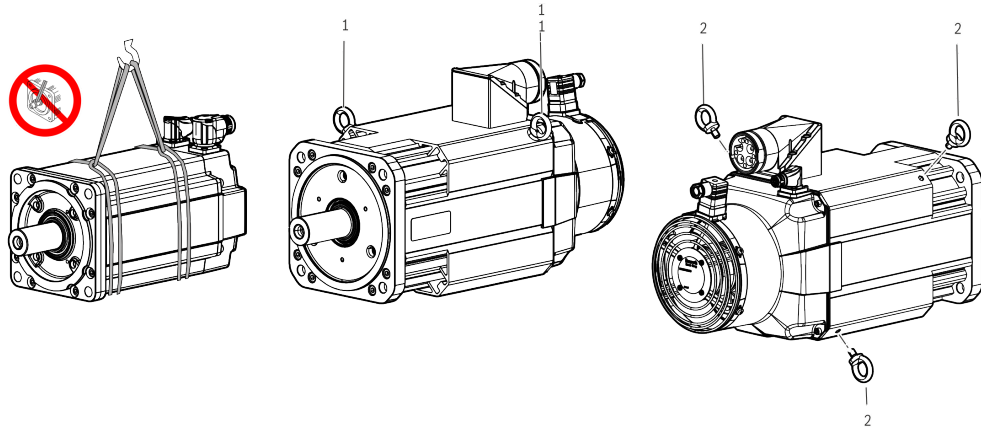
Fig. 400: Lifting and transporting motors
