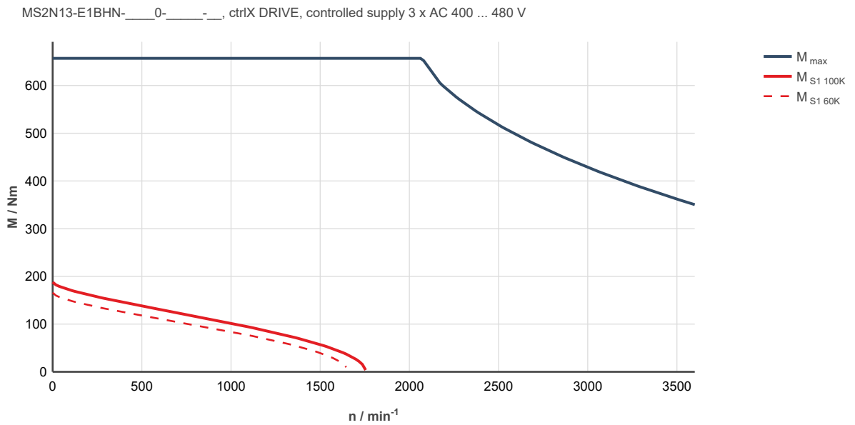
Fig. 315: MS2N13-E1BHN-___0-___-___, ctrlX DRIVE, controlled supply 3 x AC 400 ... 480 V
