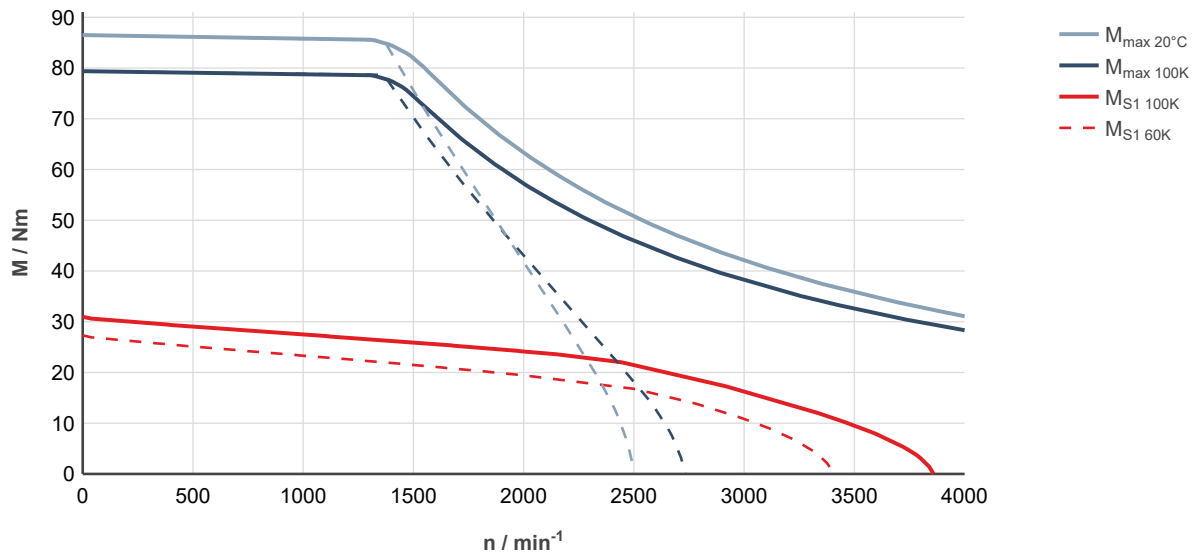
Fig. 198: MS2N10-C1BHN-___0-___-_, ctrlX DRIVE, uncontrolled supply 3 × AC 400 V
