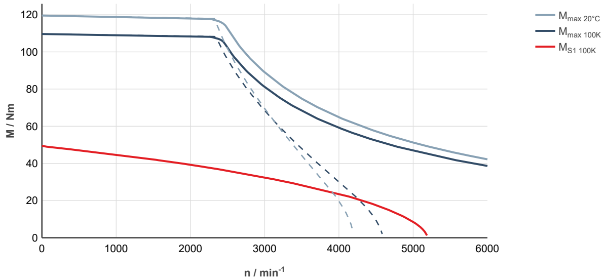
Fig. 154: MS2N07-E0BNA-___0-___-_, ctrIX DRIVE, controlled supply 3 × AC 400 ... 480 V
