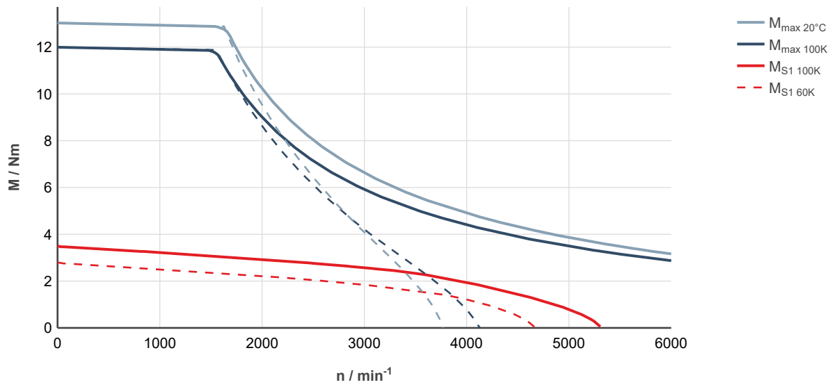
Fig. 38: MS2N04-C0BNN-___0-___-__, ctrlX DRIVE, uncontrolled supply 3 × AC 400 V
