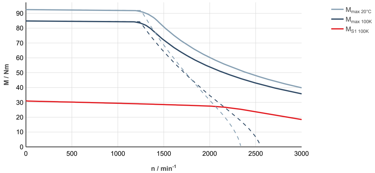
Fig. 144: MS2N07-D1BFA-___0-___-__, ctrlX DRIVE, controlled supply 3 × AC 400 ... 480 V
