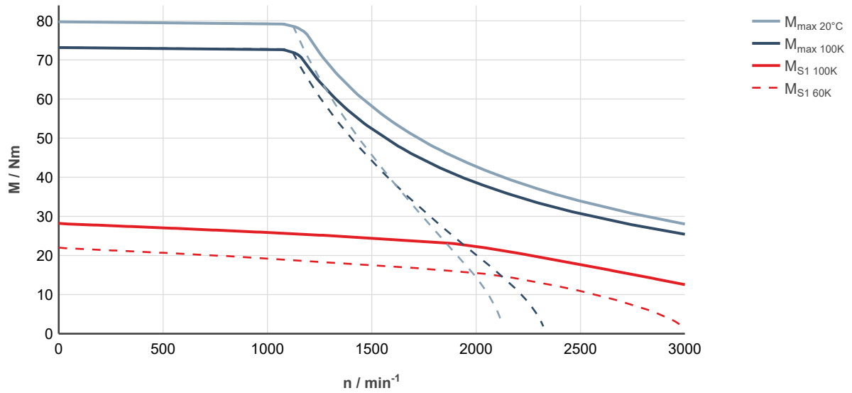
Fig. 100: MS2N07-D0BFN-___0-___-__, ctrlX DRIVE, controlled supply 3 × AC 400 ... 480 V
