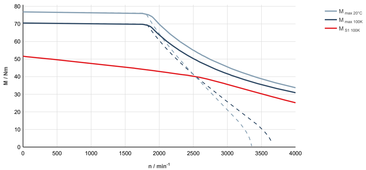
Fig. 263: MS2N10-C0BHL-___0-___-_0, ctrlX DRIVE, controlled supply 3 x AC 400 ... 480 V
