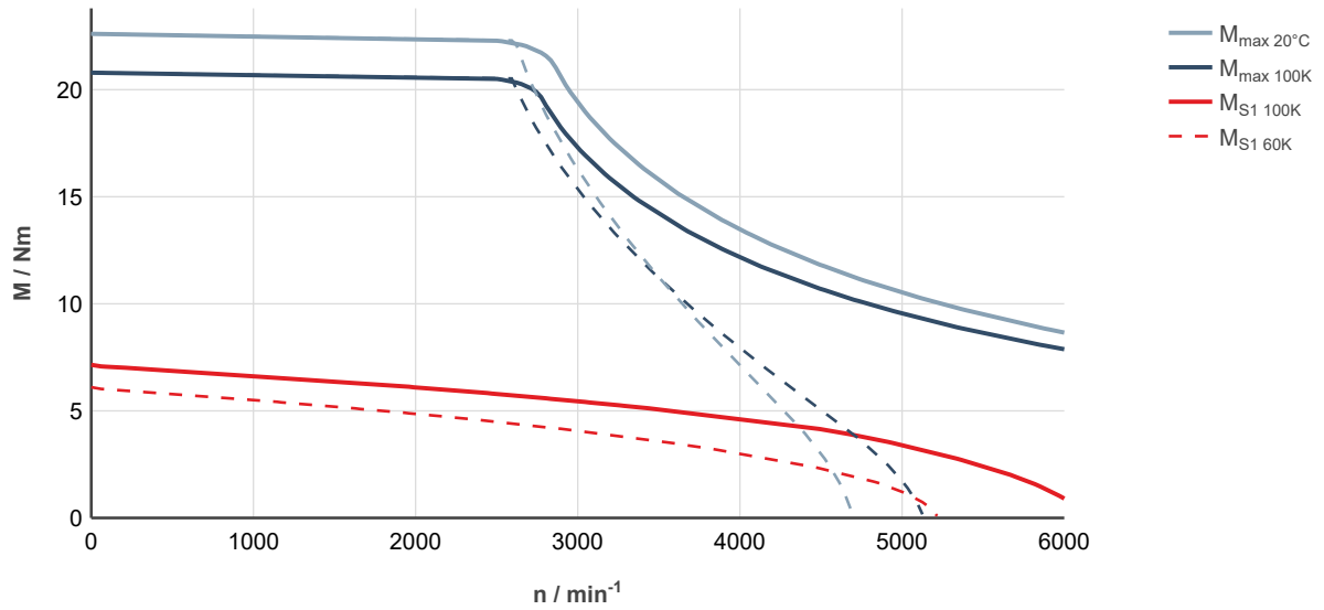
Fig. 56: MS2N05-C0BNN-___0-___-_, ctrlX DRIVE, controlled supply 3 × AC 400 ... 480 V
