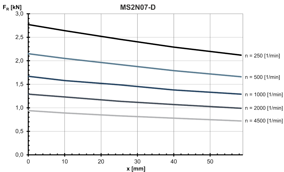
Fig. 190: MS2N07-D: Radial force in distance x from the shaft shoulder at a nominal bearing service life of L_{h10} = 30000 h
