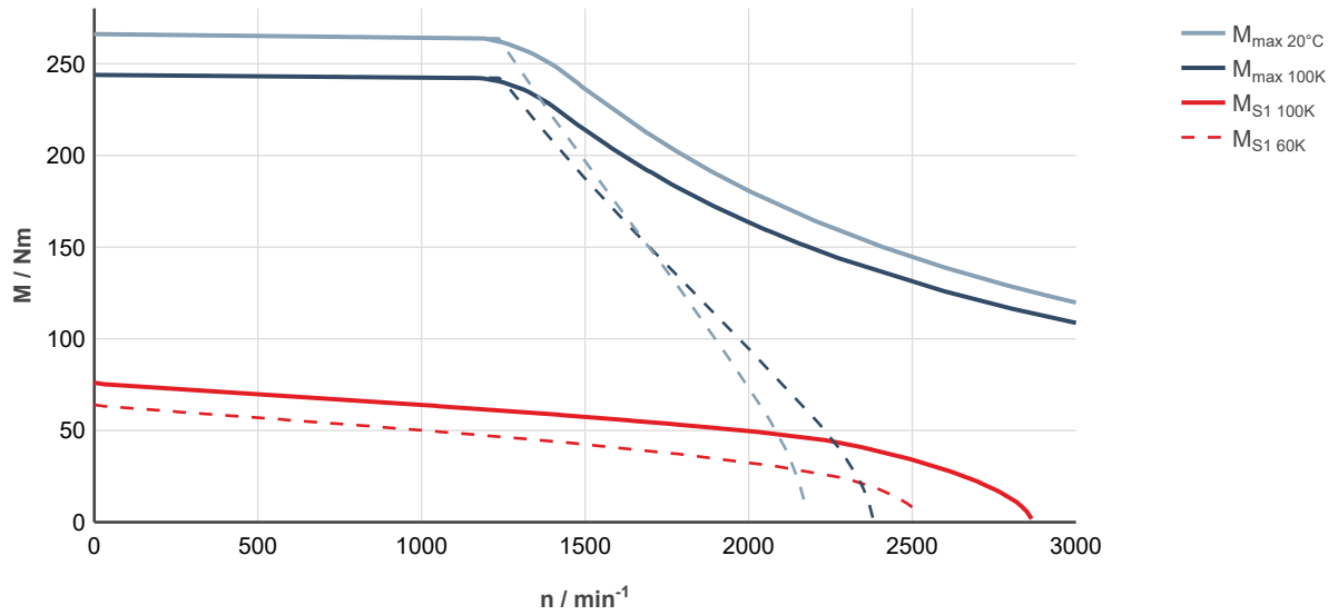
Fig. 215: MS2N10-E1BFN-___0-___-__, ctrlX DRIVE, controlled supply 3 × AC 400 ... 480 V
