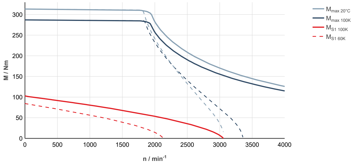
Fig. 221: MS2N10-F0BHN-___0-___-_, ctrlX DRIVE, controlled supply 3 × AC 400 ... 480 V
