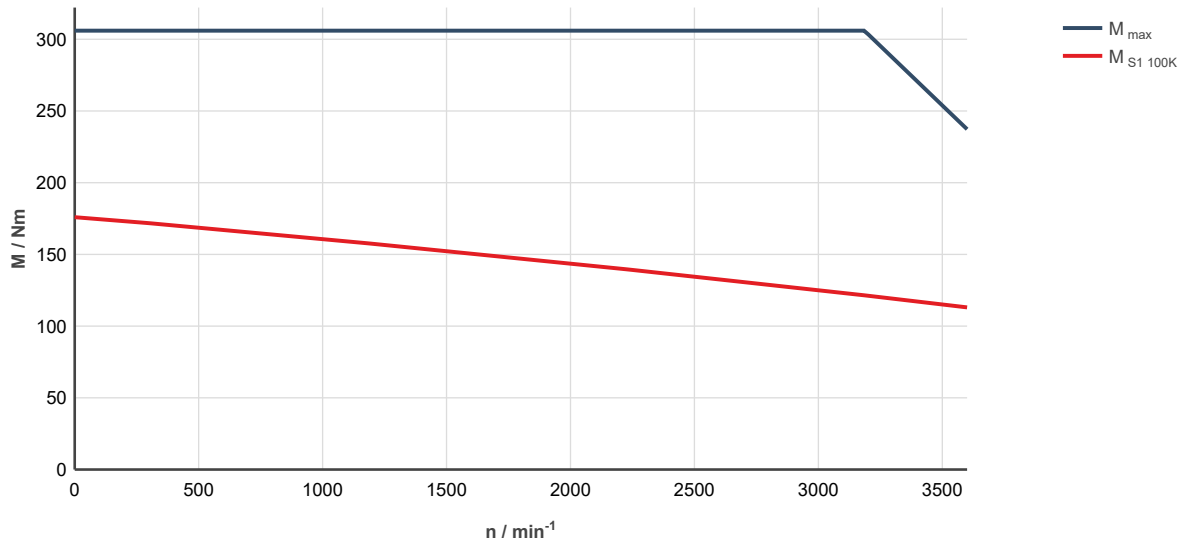
Fig. 337: MS2N13-B1BNL-___0-___-__, ctrlX DRIVE, controlled supply 3 x AC 400 ... 480 V
