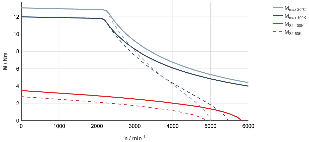
Fig. 39: MS2N04-C0BNN-___0-___-__, ctrlX DRIVE, controlled supply 3 × AC 400 ... 480 V
