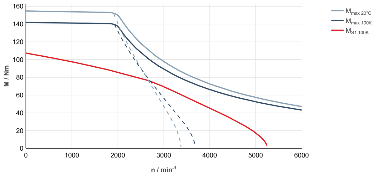
Fig. 270: MS2N10-D0BNL-___0-___-___, ctrIX DRIVE, uncontrolled supply 3 × AC 400 V
