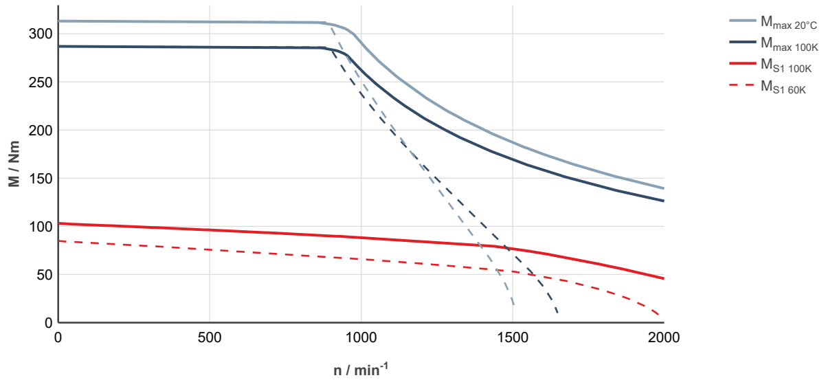
Fig. 219: MS2N10-F0BDN-___0-___-_, ctrlX DRIVE, controlled supply 3 × AC 400 ... 480 V
