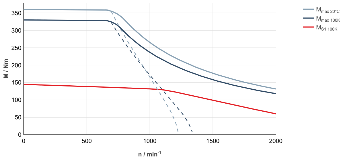
Fig. 256: MS2N10-F1BDA-___0-___-__, ctrlX DRIVE, uncontrolled supply 3 × AC 400 V
