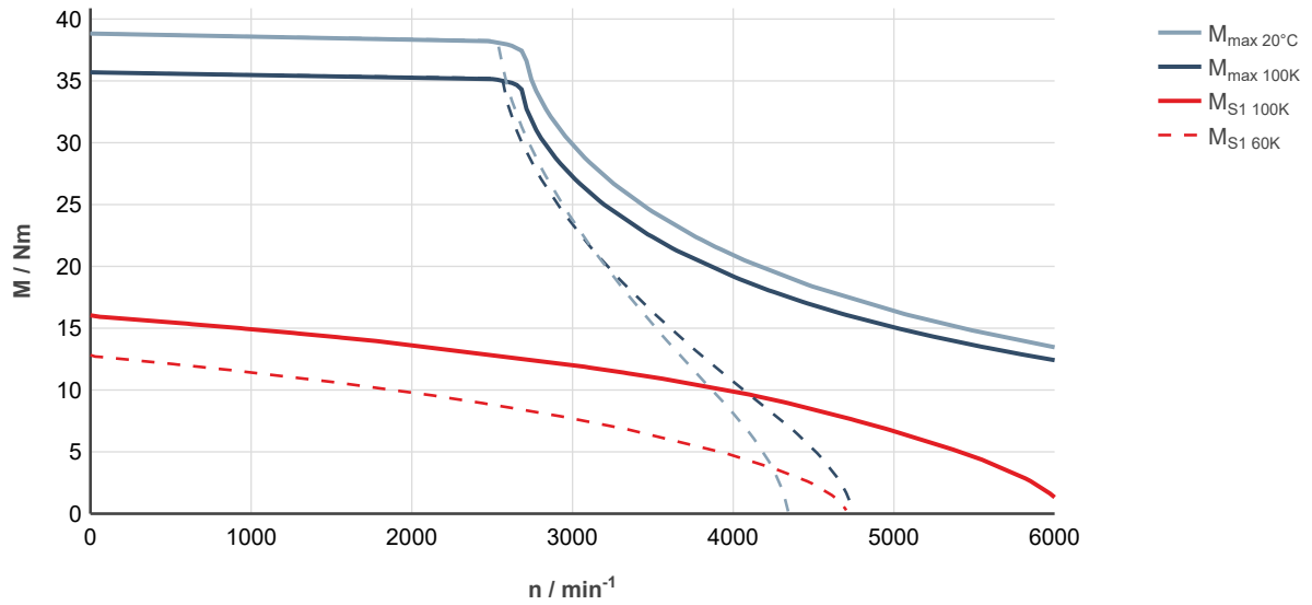
Fig. 92: MS2N07-C0BNN-___0-___-_, ctrlX DRIVE, controlled supply 3 × AC 400 ... 480 V
