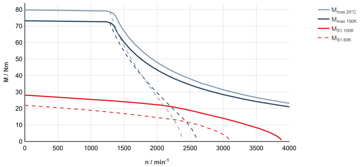
Fig. 101: MS2N07-D0BHN-___0-___-_, ctrlX DRIVE, uncontrolled supply 3 × AC 400 V
