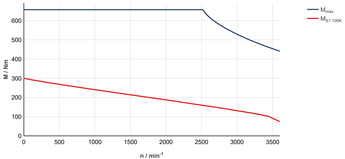
Fig. 333: MS2N13-E1BNC-___0-___-_, ctrIX DRIVE, controlled supply 3 x AC 400 ... 480 V M_{\text{max}} Characteristic curve applies to maximum torque 20 °C (cold)
