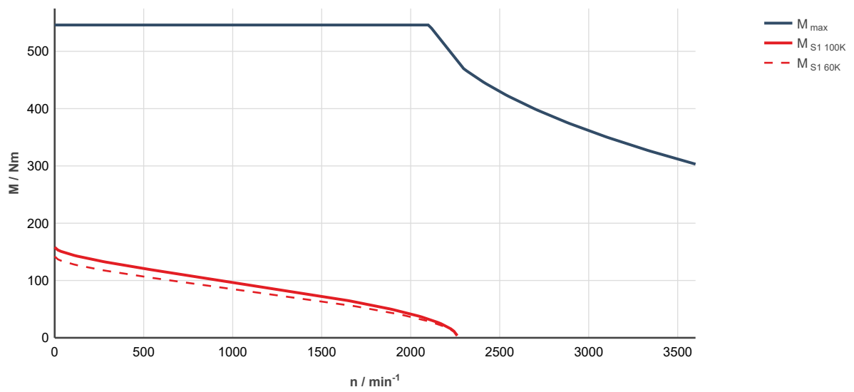
Fig. 312: MS2N13-D1BNN-___0-___-_, ctrlX DRIVE, uncontrolled supply 3 × AC 400 V
