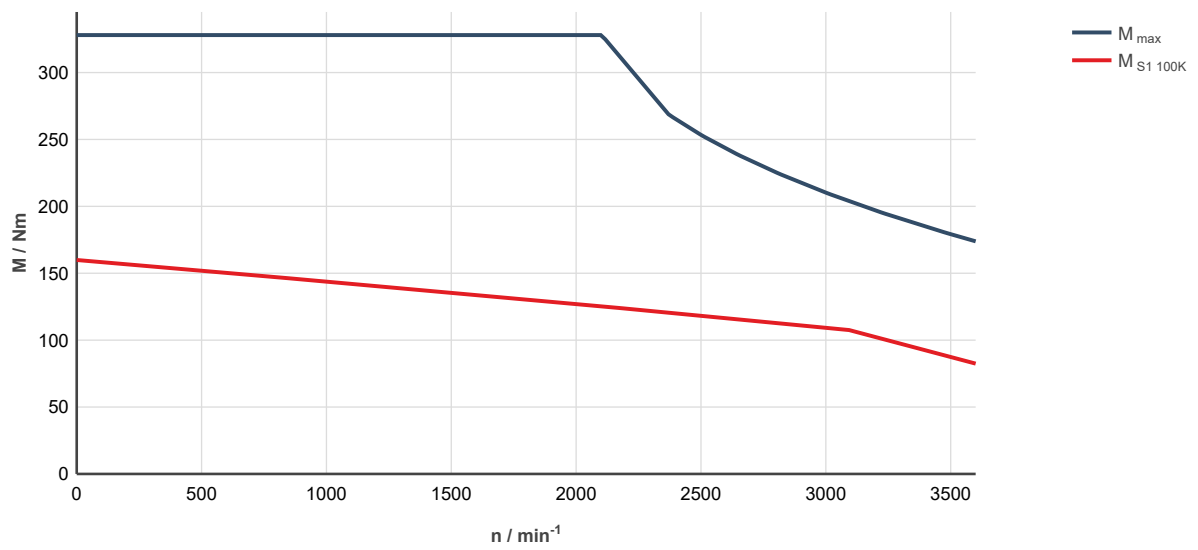
Fig. 320: MS2N13-B1BNC-___0-___-_, ctrlX DRIVE, uncontrolled supply 3 × AC 400 V
