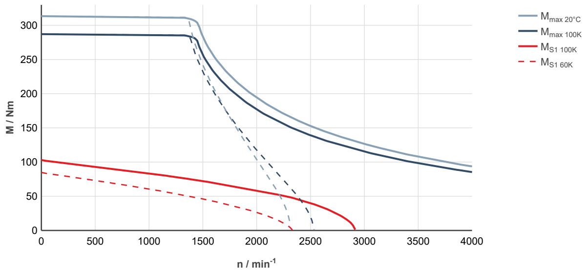
Fig. 220: MS2N10-F0BHN-___0-___-_, ctrlX DRIVE, uncontrolled supply 3 × AC 400 V
