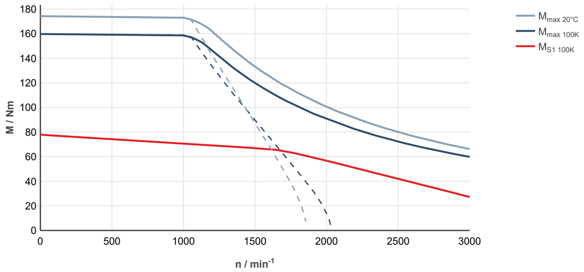
Fig. 240: MS2N10-D1BFA-___0-___-__, ctrlX DRIVE, uncontrolled supply 3 × AC 400 V
