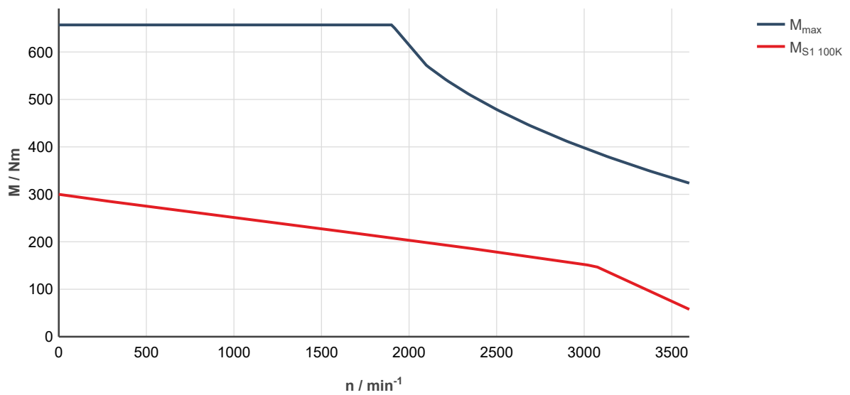
Fig. 332: MS2N13-E1BNC-___0-___-_, ctrIX DRIVE, uncontrolled supply 3 x AC 400 V M_{\text{max}} Characteristic curve applies to maximum torque 20 °C (cold)
