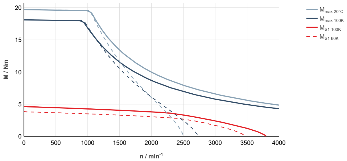
Fig. 42: MS2N04-D0BHN-___0-___-_, ctrlX DRIVE, uncontrolled supply 3 × AC 400 V
