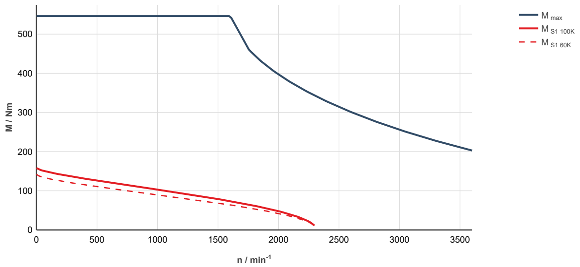
Fig. 310: MS2N13-D1BHN-___0-___-_, ctrlX DRIVE, uncontrolled supply 3 × AC 400 V
