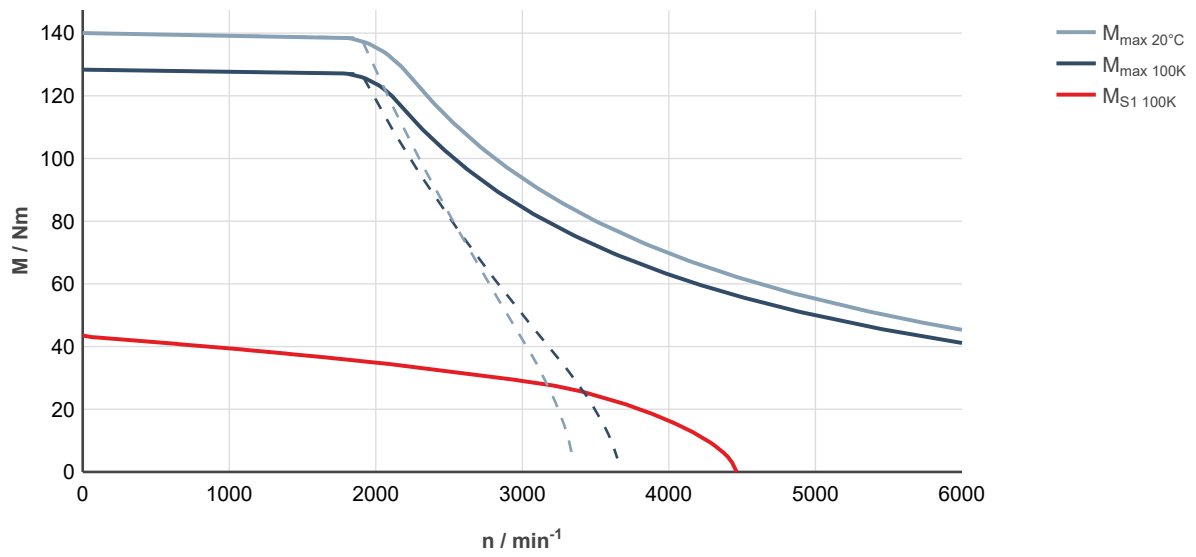
Fig. 161: MS2N07-E1BNA-___0-___-__, ctrlX DRIVE, uncontrolled supply 3 × AC 400 V
