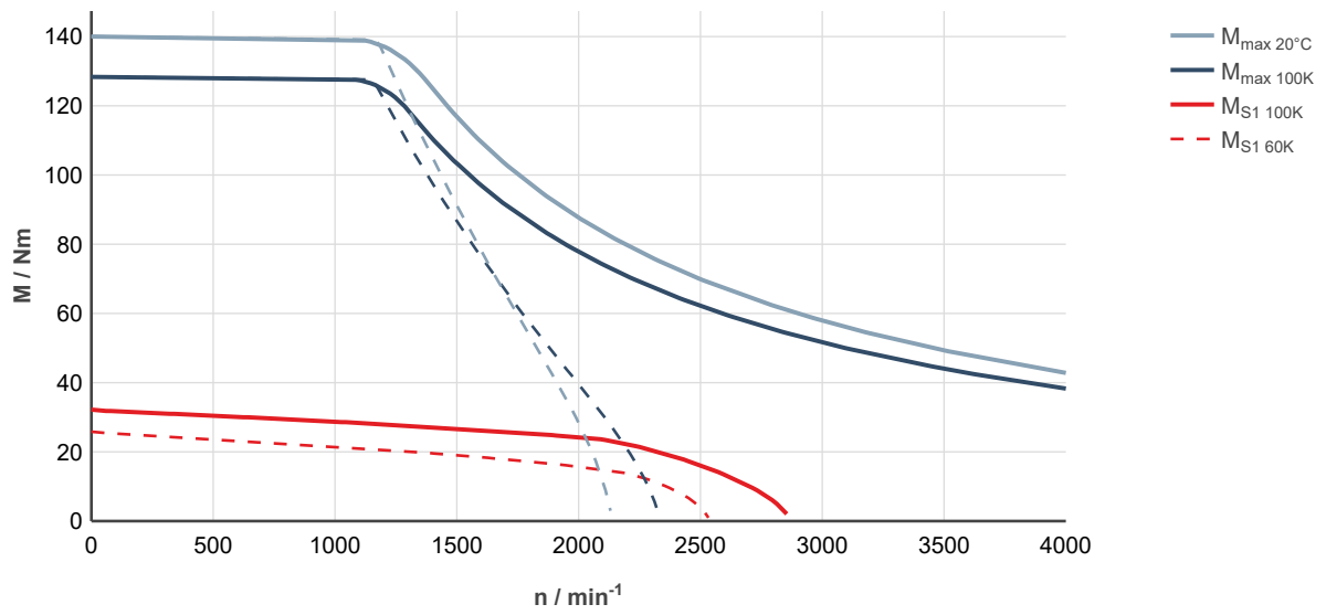
Fig. 123: MS2N07-E1BHN-___0-___-__, ctrlX DRIVE, uncontrolled supply 3 × AC 400 V
