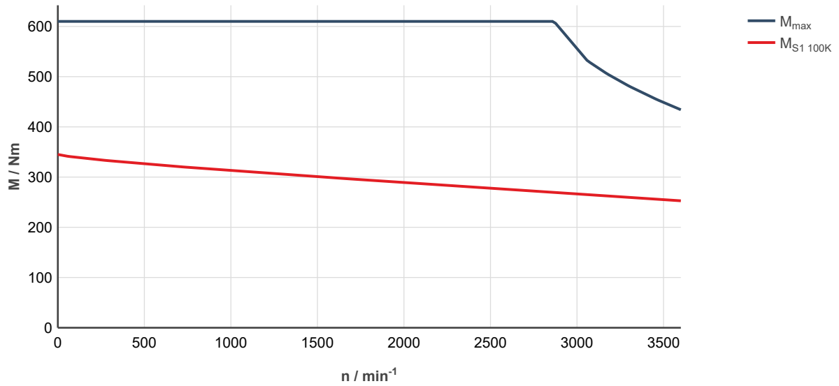
Fig. 349: MS2N13-E1BNL-___0-___-__, ctrlX DRIVE, controlled supply 3 × AC 400 ... 480 V
