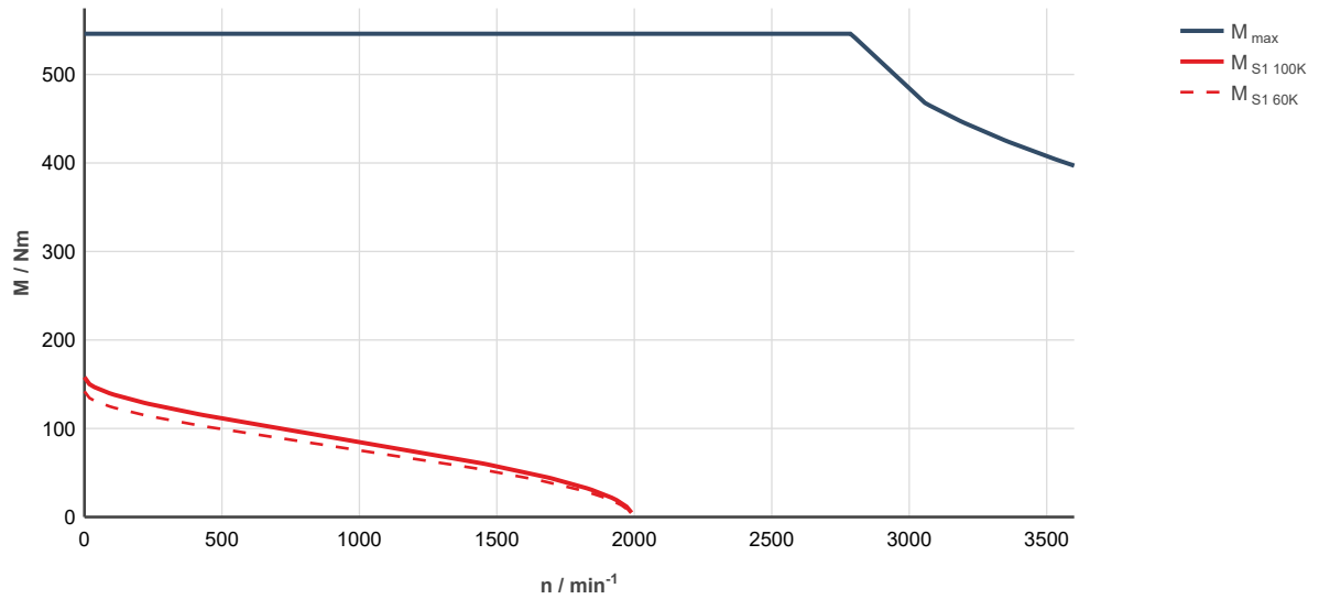
Fig. 313: MS2N13-D1BNN-___0-___-_, ctrlX DRIVE, controlled supply 3 x AC 400 ... 480 V
