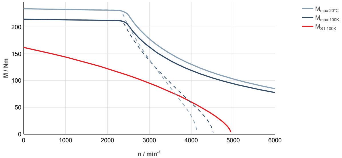
Fig. 277: MS2N10-E0BNL-___0-___-___, ctrlX DRIVE, controlled supply 3 × AC 400 ... 480 V
