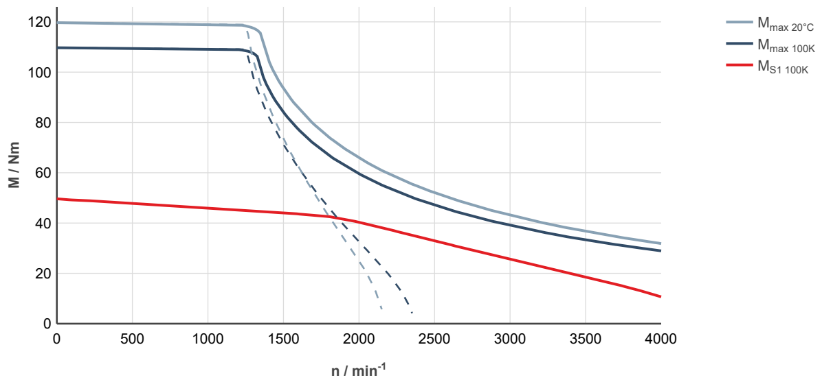
Fig. 151: MS2N07-E0BHA-___0-___-__, ctrlX DRIVE, uncontrolled supply 3 × AC 400 V
