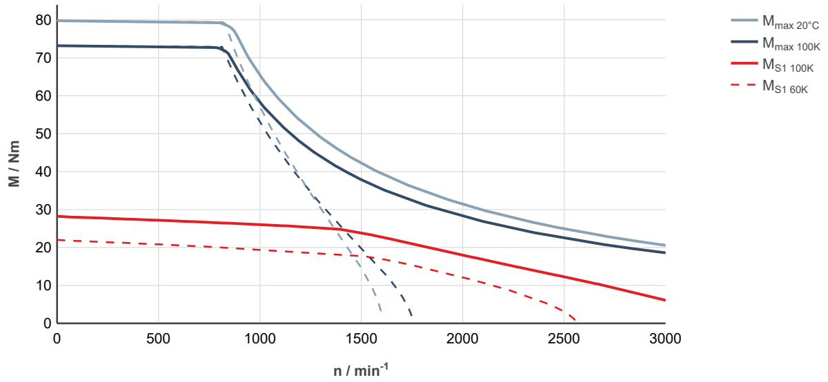
Fig. 99: MS2N07-D0BFN-___0-___-__, ctrlX DRIVE, uncontrolled supply 3 × AC 400 V
