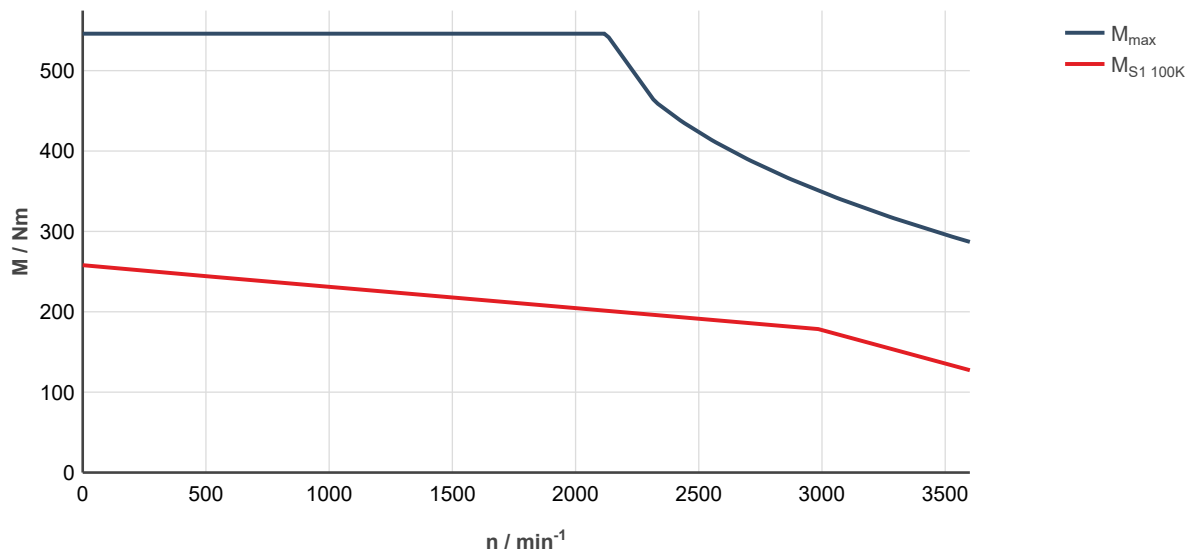
Fig. 327: MS2N13-D1BHC-___0-___-_, ctrlX DRIVE, controlled supply 3 x AC 400 ... 480 V M_{\text{max}} Characteristic curve applies to maximum torque 20 °C (cold)
