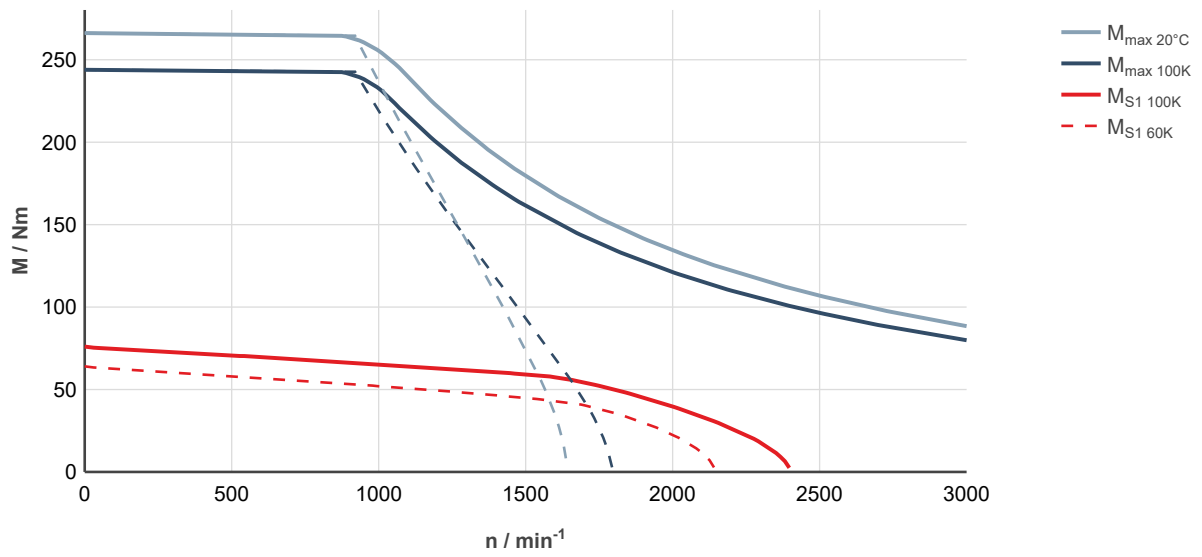
Fig. 214: MS2N10-E1BFN-___0-___-__, ctrlX DRIVE, uncontrolled supply 3 × AC 400 V
