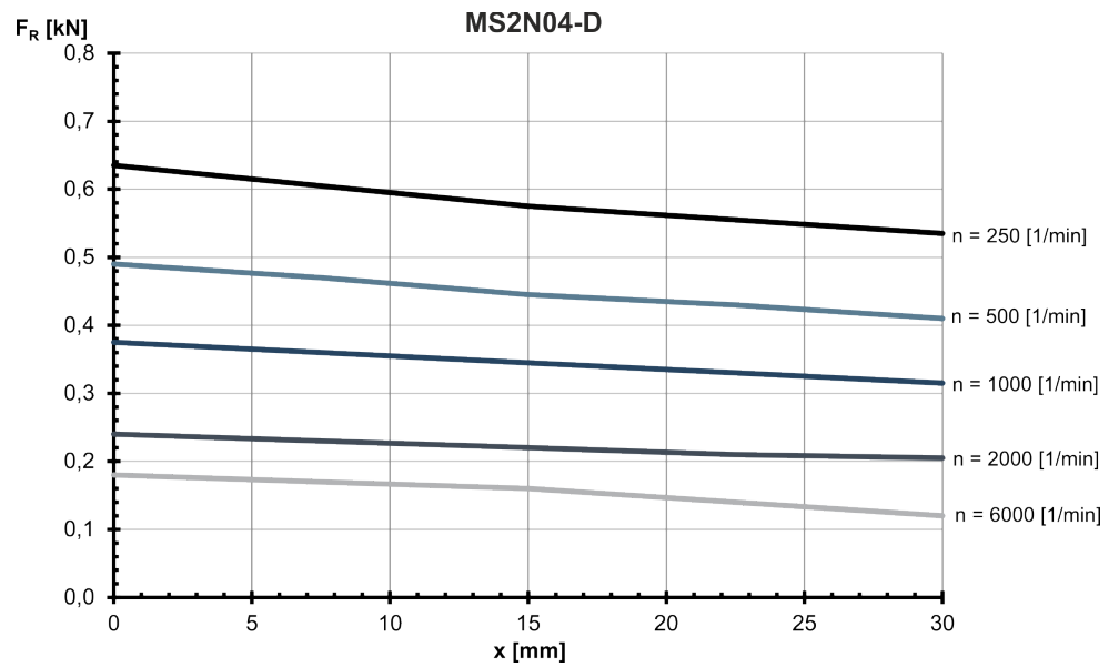
Fig. 50: MS2N04-D: Radial force in distance x from the shaft shoulder at a nominal bearing service life of L_{h10} = 30000 h
