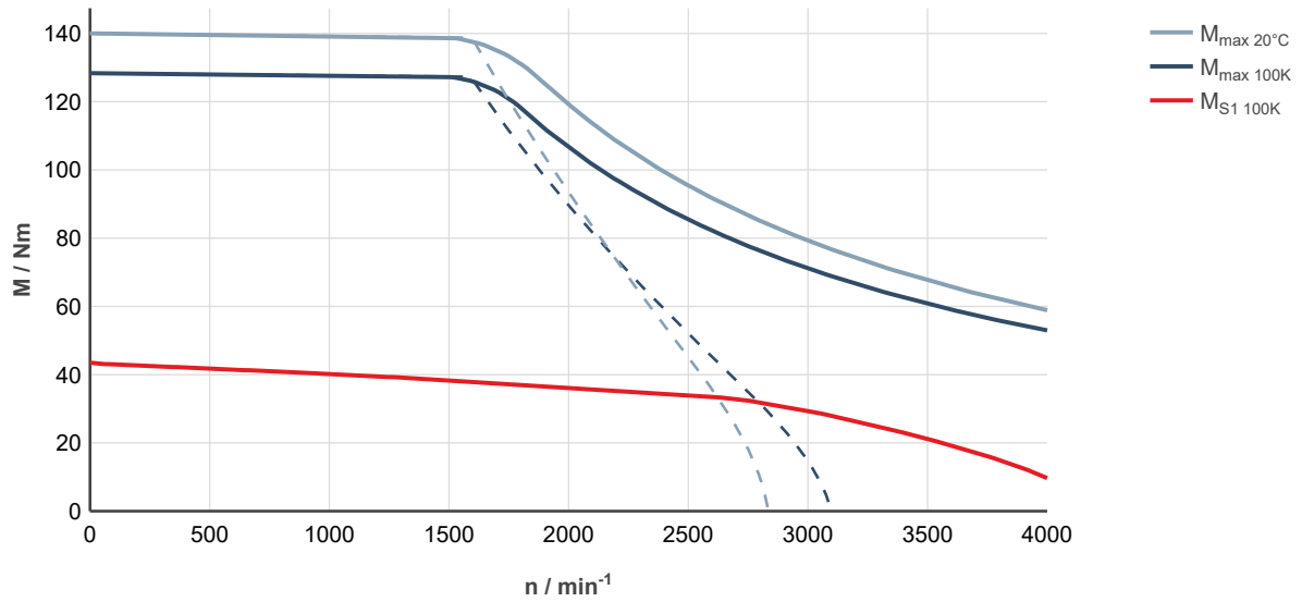
Fig. 160: MS2N07-E1BHA-___0-___-_, ctrlX DRIVE, controlled supply 3 × AC 400 ... 480 V
