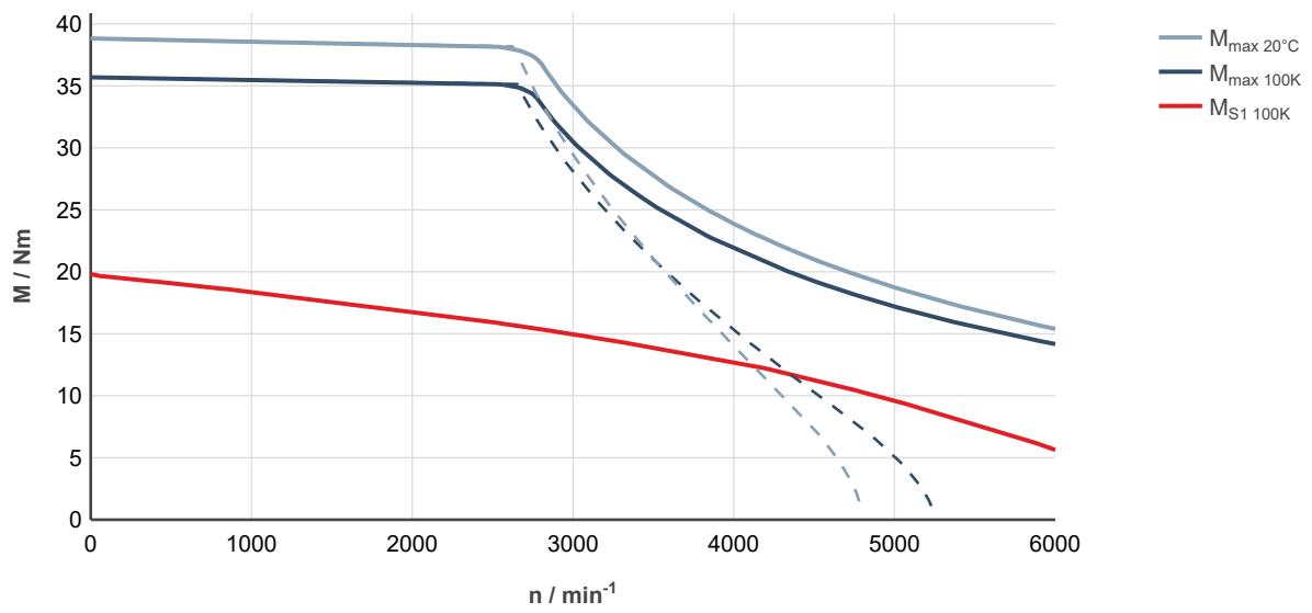
Fig. 129: MS2N07-C0BQA-___0-___-_, ctrlX DRIVE, uncontrolled supply 3 × AC 400 V
