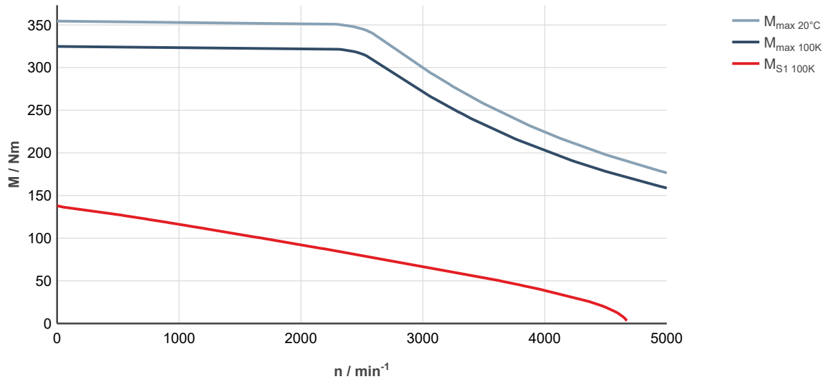
Fig. 261: MS2N10-R0BLA-___-___-__, ctrlX DRIVE, controlled supply 3 x AC 400 ... 480 V
