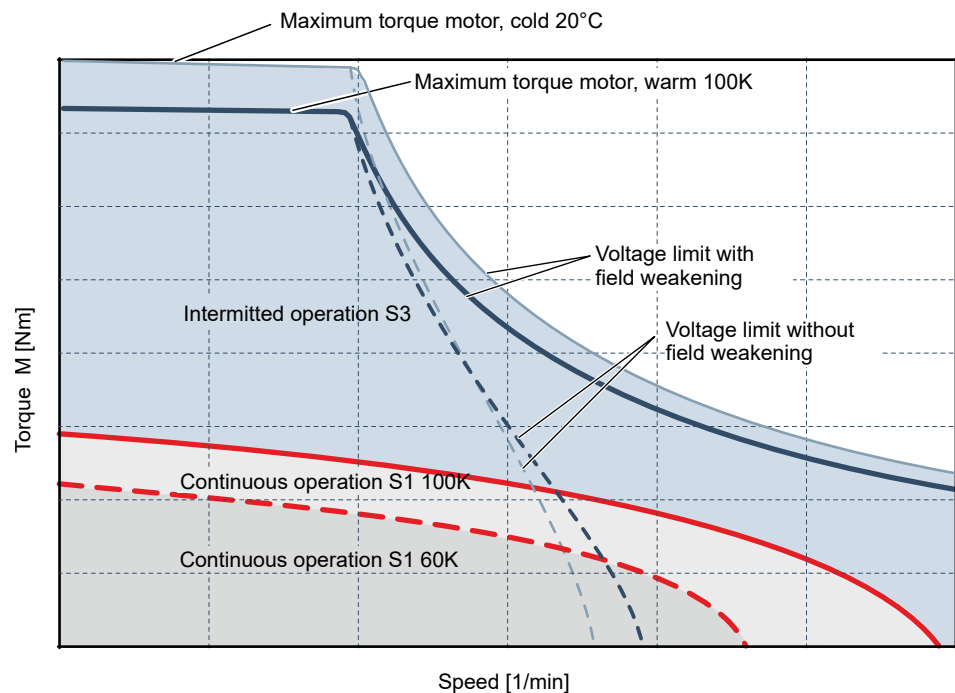
Fig. 18: Operating area of MS2N motors
