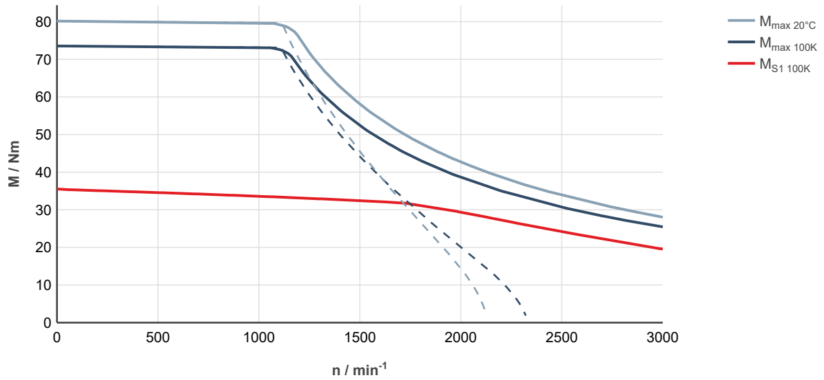
Fig. 136: MS2N07-D0BFA-...0-...-..., ctrlX DRIVE, controlled supply 3 × AC 400 ... 480 V
