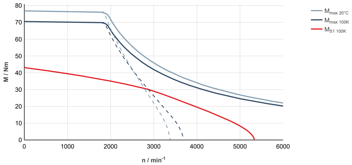
Fig. 230: MS2N10-C0BNA-___0-___-_, ctrlX DRIVE, uncontrolled supply 3 × AC 400 V
