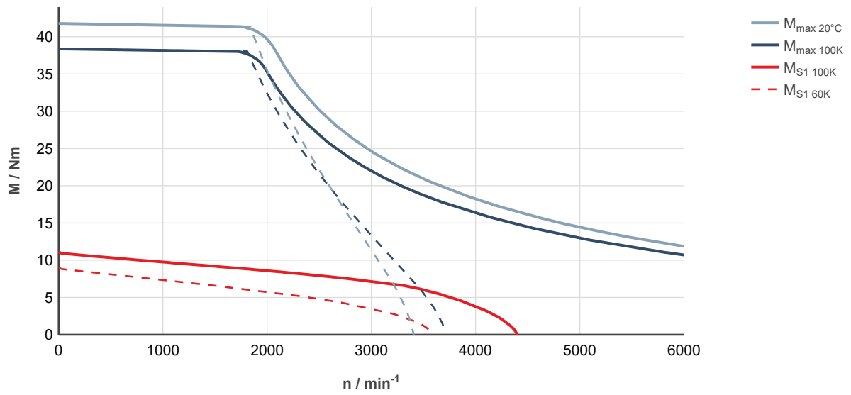
Fig. 78: MS2N06-D1BNN-___0-___-_, ctrlX DRIVE, uncontrolled supply 3 × AC 400 V
