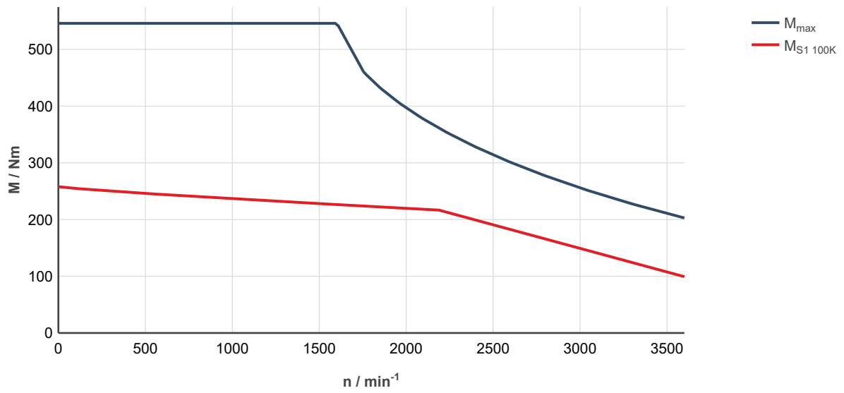
Fig. 326: MS2N13-D1BHC-___0-___-_, ctrlX DRIVE, uncontrolled supply 3 × AC 400 V(1) M_{\text{max}} Characteristic curve applies to maximum torque 20 °C (cold)
