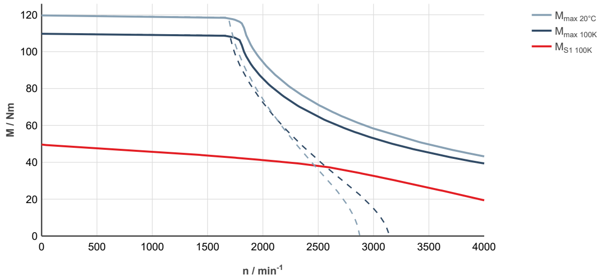
Fig. 152: MS2N07-E0BHA-___0-___-__, ctrlX DRIVE, controlled supply 3 × AC 400 ... 480 V
