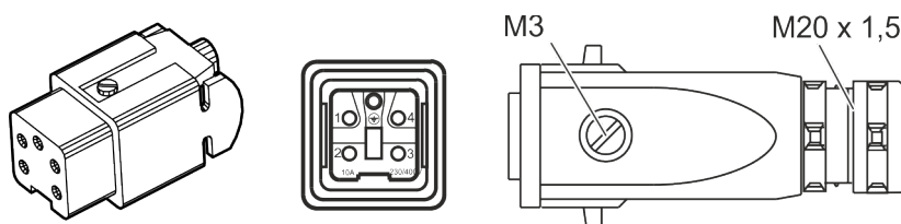
Fig. 388: RLS0782_Single components fan connector
