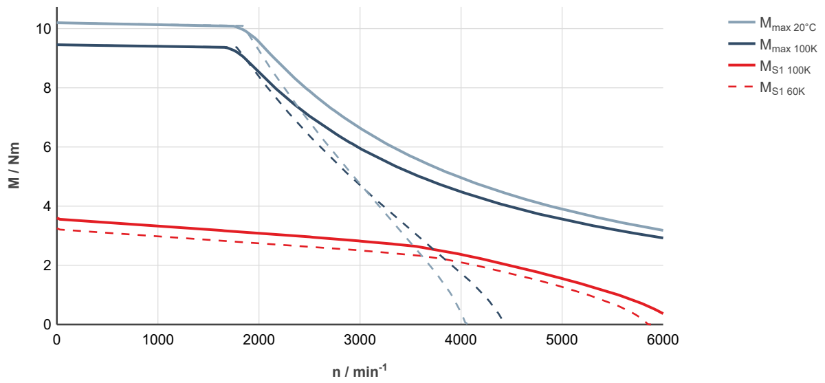
Fig. 68: MS2N06-B1BNN-___0-___-__, ctrlX DRIVE, uncontrolled supply 3 × AC 400 V
