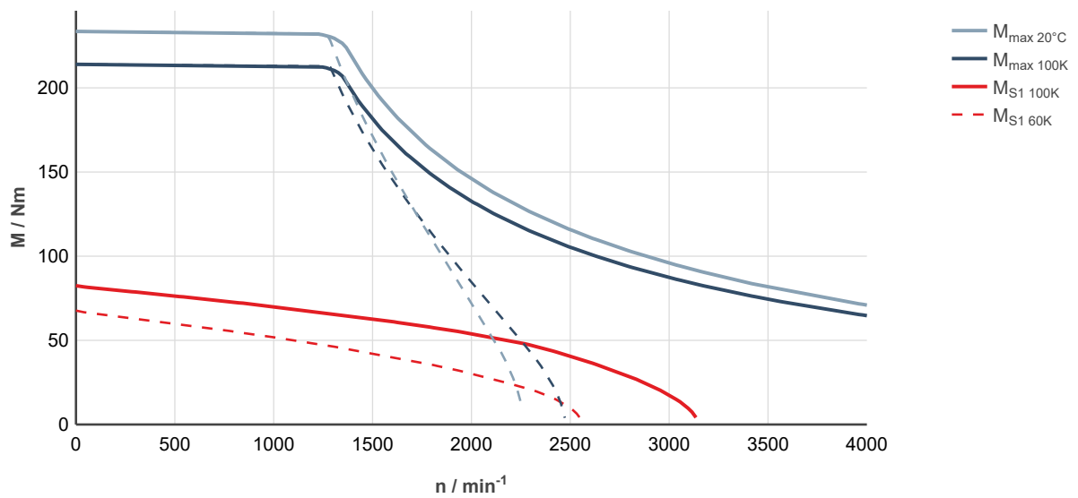
Fig. 210: MS2N10-E0BHN-___0-___-_, ctrlX DRIVE, uncontrolled supply 3 × AC 400 V
