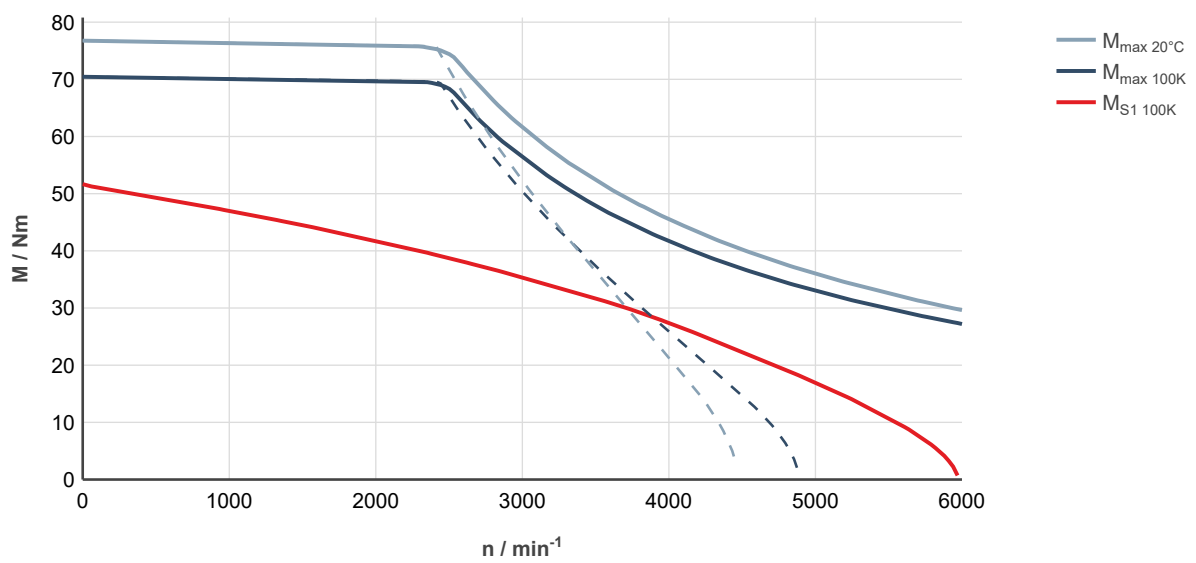
Fig. 265: MS2N10-C0BNL-___0-___-___, ctrIX DRIVE, controlled supply 3 × AC 400 ... 480 V
