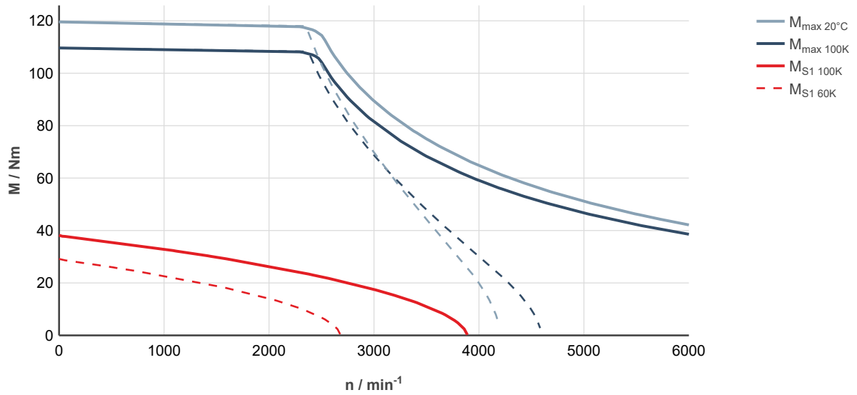
Fig. 118: MS2N07-E0BNN-___0-___-_, ctrlX DRIVE, controlled supply 3 × AC 400 ... 480 V
