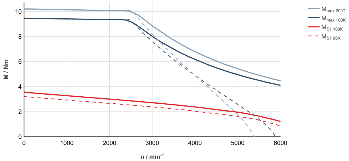
Fig. 69: MS2N06-B1BNN-___0-___-__, ctrlX DRIVE, controlled supply 3 × AC 400 ... 480 V
