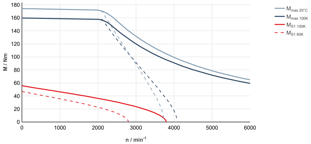
Fig. 208: MS2N10-D1BNN-___0-___-_, ctrlX DRIVE, uncontrolled supply 3 × AC 400 V
