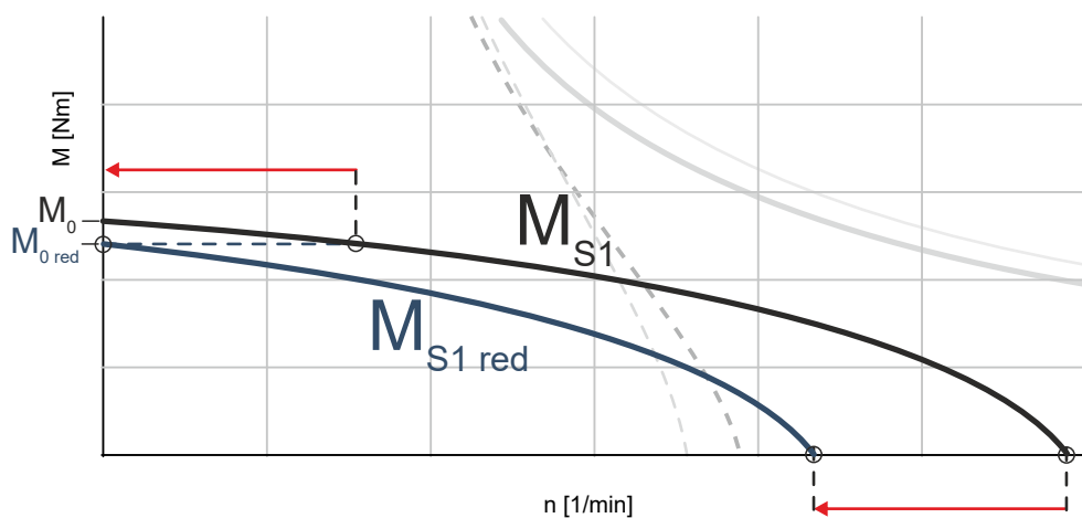
Fig. 399: Determine S1-characteristic curve M_{S1\ red} with derating factor f_{TH}
