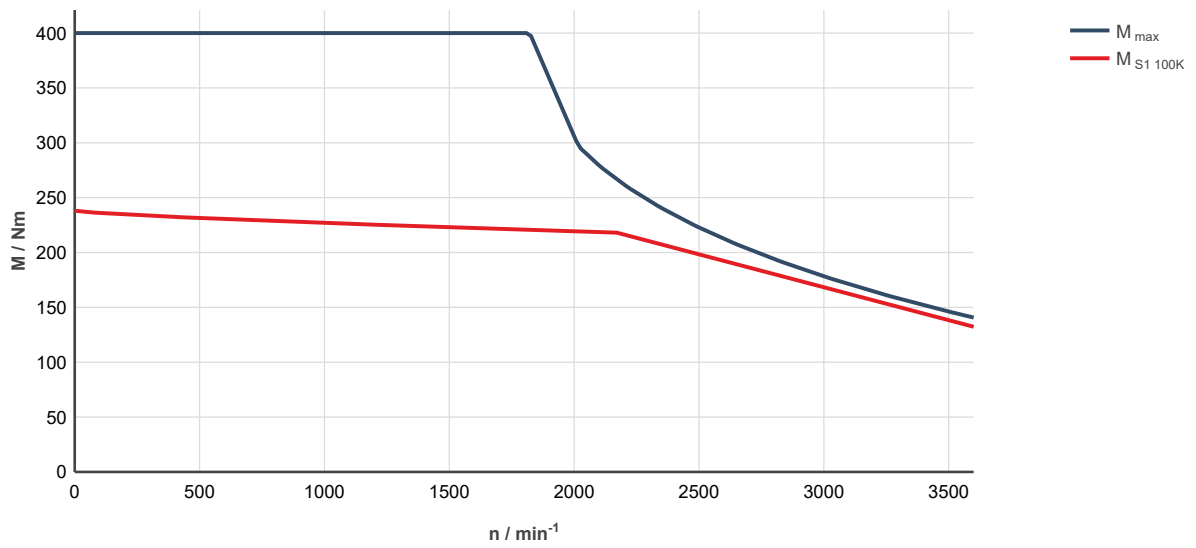
Fig. 338: MS2N13-C1BHL-___0-___-__, ctrlX DRIVE, uncontrolled supply 3 × AC 400 V M_{\text{max}} Characteristic curve applies to maximum torque 20 °C (cold)
