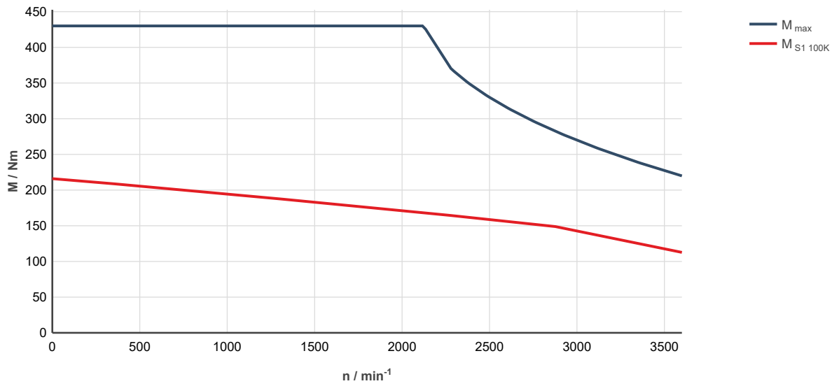
Fig. 324: MS2N13-C1BNC-___0-N___-___, ctrlX DRIVE, uncontrolled supply 3 x AC 400 V
