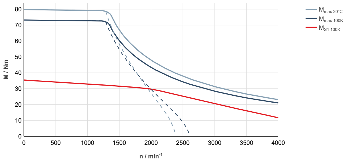
Fig. 137: MS2N07-D0BHA-___0-___-_, ctrlX DRIVE, uncontrolled supply 3 × AC 400 V
