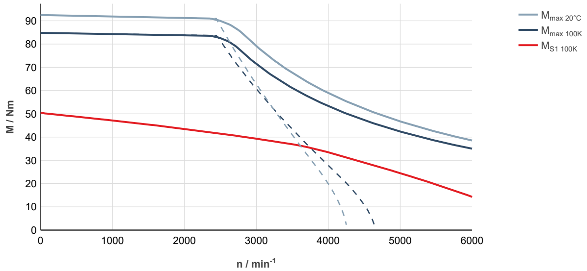
Fig. 176: MS2N07-D1BNL-___0-___-___, ctrIX DRIVE, controlled supply 3 × AC 400 ... 480 V
