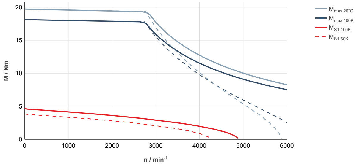
Fig. 45: MS2N04-D0BQN-___0-___-__, ctrlX DRIVE, controlled supply 3 × AC 400 ... 480 V
