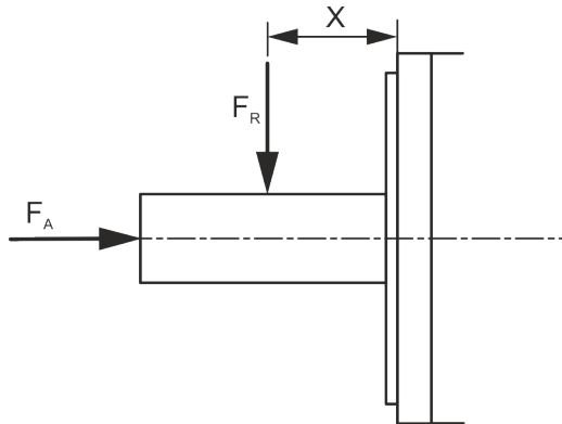
Fig. 16: Point of action of radial force F_R and axial force F_A
