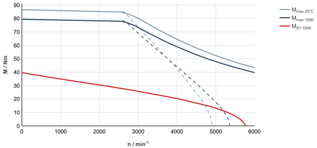
Fig. 235: MS2N10-C1BNA-___0-___-_, ctrlX DRIVE, controlled supply 3 × AC 400 ... 480 V
