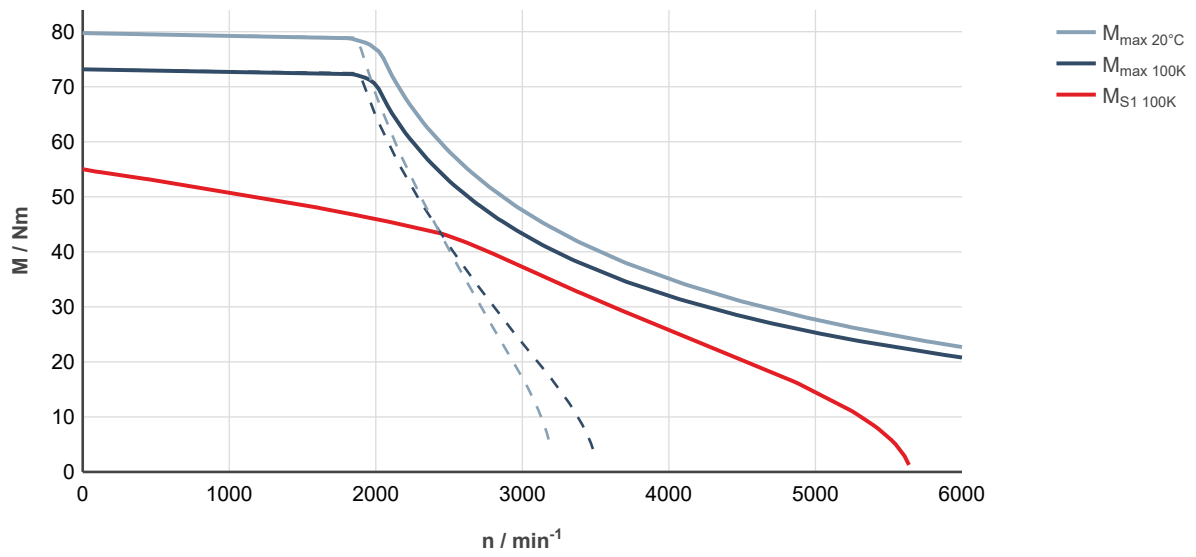
Fig. 171: MS2N07-D0BNL-__0-__-__, ctrlX DRIVE, uncontrolled supply 3 × AC 400 V
