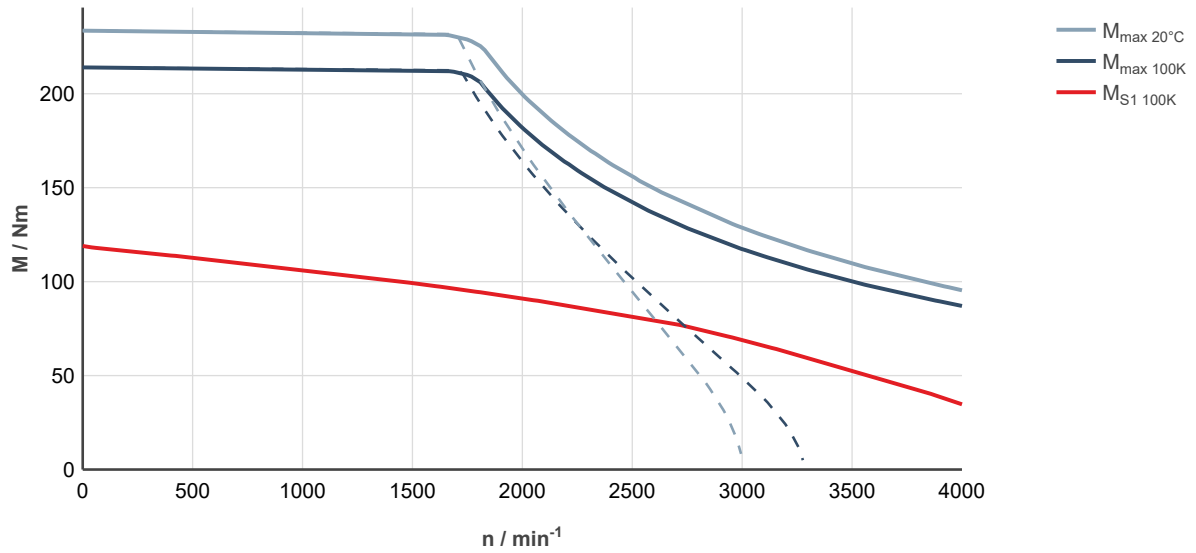
Fig. 245: MS2N10-E0BHA-___0-___-_, ctrlX DRIVE, controlled supply 3 × AC 400 ... 480 V
