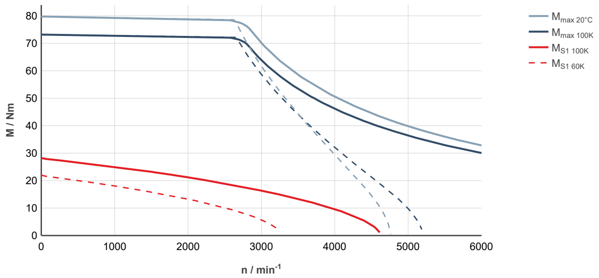
Fig. 105: MS2N07-D0BRN-___0-___-_, ctrlX DRIVE, uncontrolled supply 3 × AC 400 V
