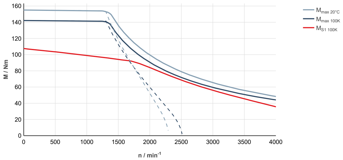
Fig. 268: MS2N10-D0BHL-___0-___-___, ctrIX DRIVE, uncontrolled supply 3 × AC 400 V
