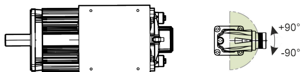
Fig. 372: Rotating area electrical connection “E”
