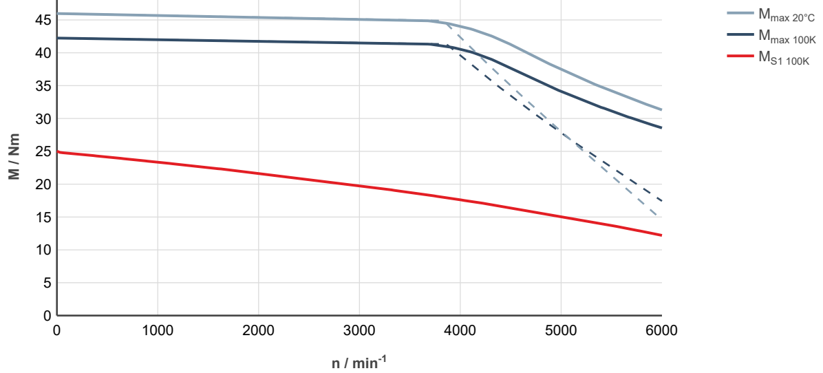
Fig. 168: MS2N07-C1BRL-___0-___-__, ctrlX DRIVE, controlled supply 3 × AC 400 ... 480 V
