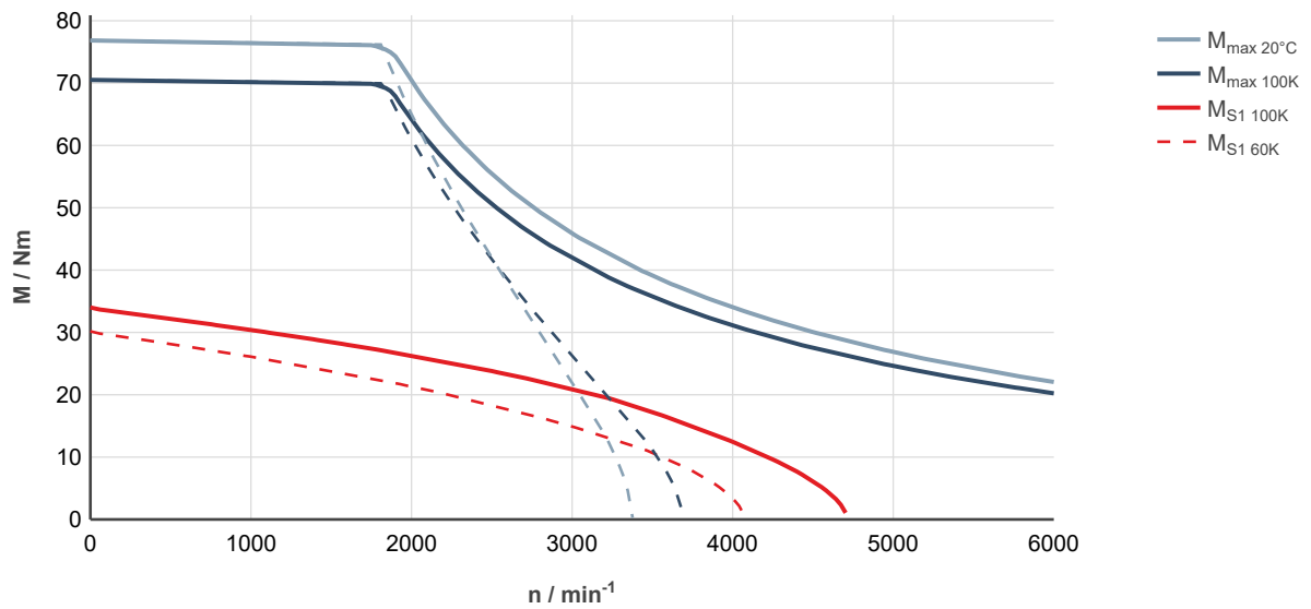
Fig. 196: MS2N10-C0BNN-___0-___- , ctrlX DRIVE, uncontrolled supply 3 × AC 400 V
