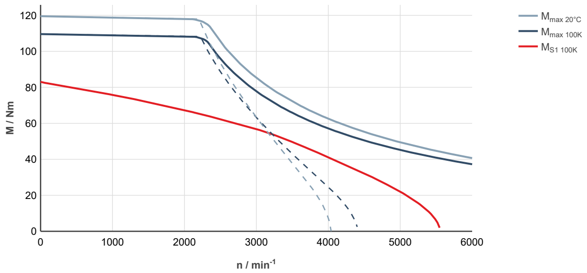
Fig. 181: MS2N07-E0BQL-___0-___-___, ctrIX DRIVE, uncontrolled supply 3 × AC 400 V
