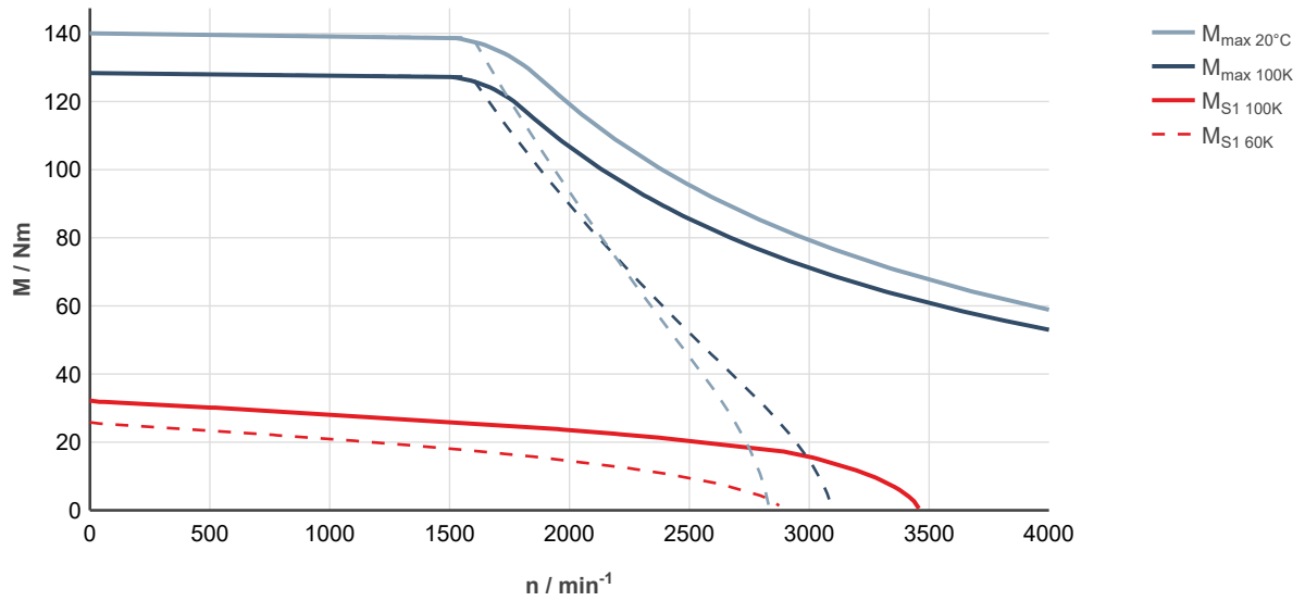
Fig. 124: MS2N07-E1BHN-___0-___-__, ctrlX DRIVE, controlled supply 3 × AC 400 ... 480 V
