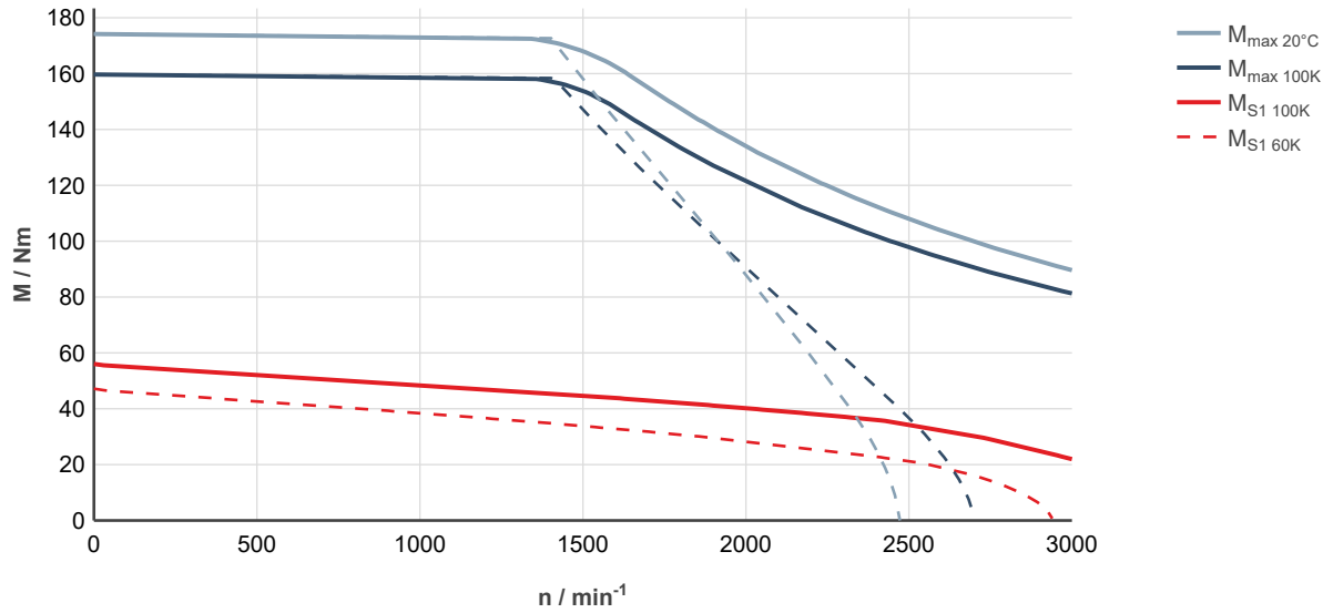
Fig. 207: MS2N10-D1BFN-___0-___-_, ctrlX DRIVE, controlled supply 3 × AC 400 ... 480 V
