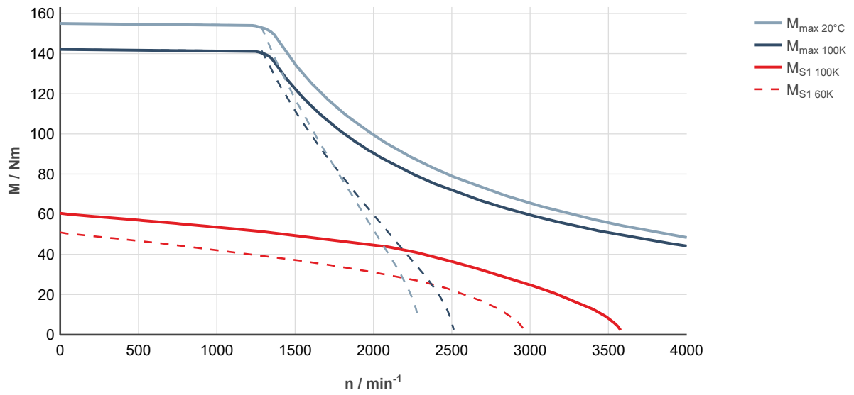
Fig. 202: MS2N10-D0BHN-___0-___-, ctrlX DRIVE, uncontrolled supply 3 × AC 400 V
