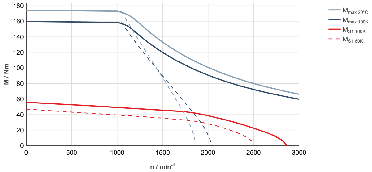
Fig. 206: MS2N10-D1BFN-___0-___-_, ctrlX DRIVE, uncontrolled supply 3 × AC 400 V
