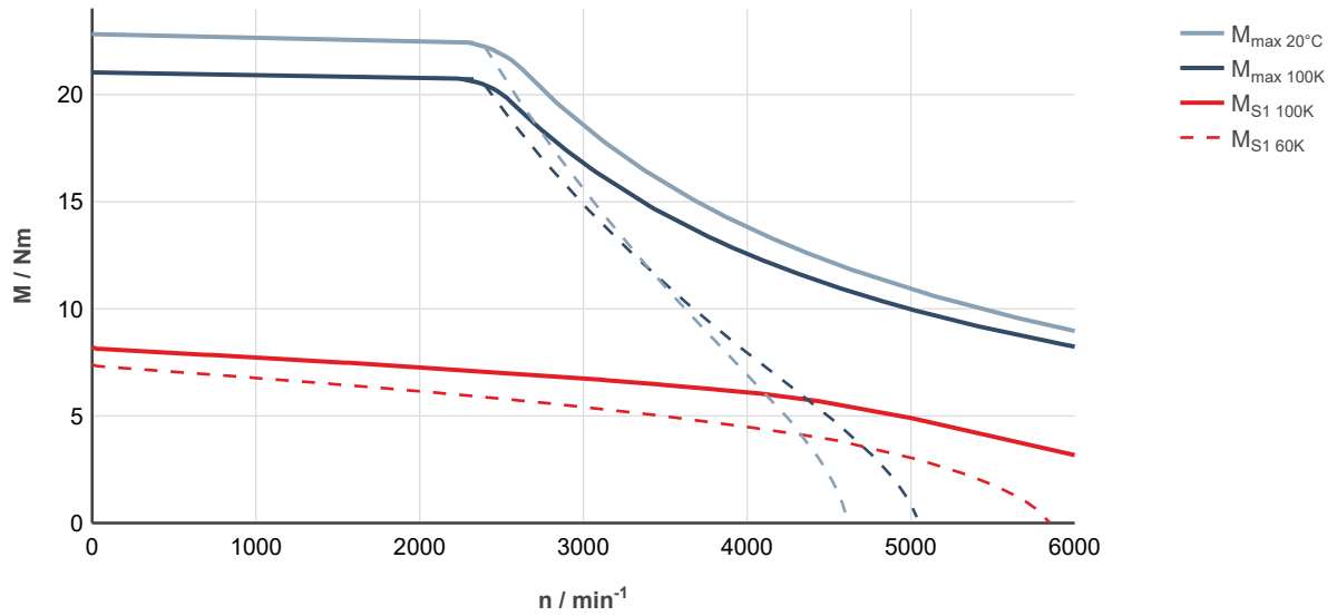
Fig. 90: MS2N07-B1BNN-___0-___-__, ctrlX DRIVE, controlled supply 3 × AC 400 ... 480 V
