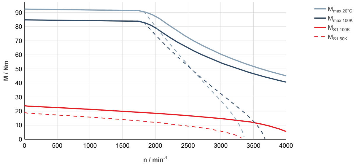
Fig. 110: MS2N07-D1BHN-___0-___-_, ctrlX DRIVE, controlled supply 3 × AC 400 ... 480 V
