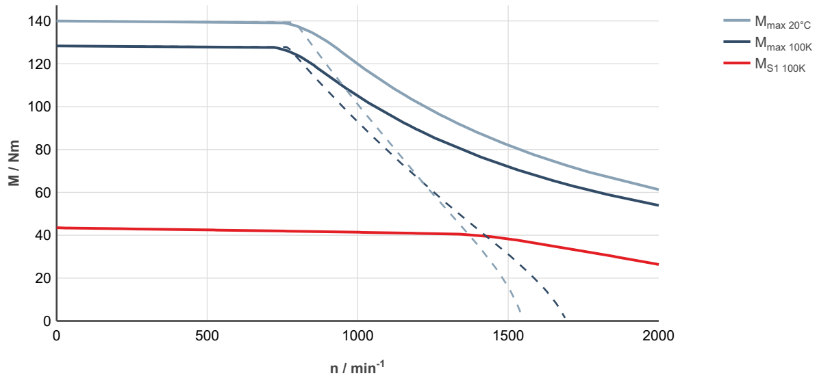
Fig. 158: MS2N07-E1BDA-___0-___-_, ctrlX DRIVE, controlled supply 3 × AC 400 ... 480 V
