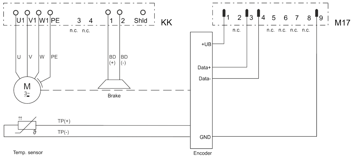
Fig. 360: Double cable connection terminal boxes, digital encoder C and D, brake optional
