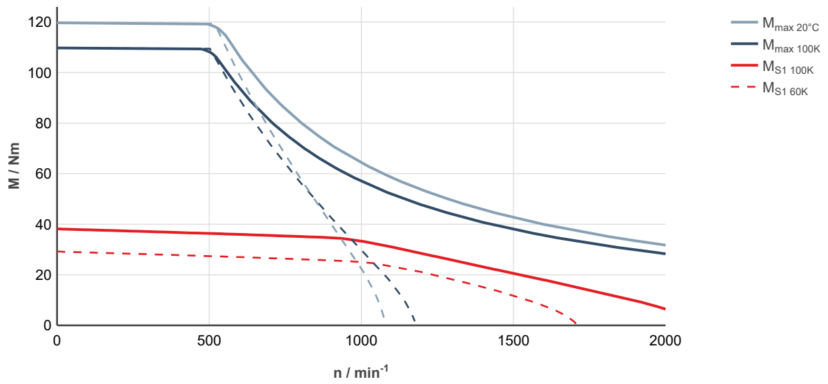
Fig. 113: MS2N07-E0BDN-___0-___-__, ctrlX DRIVE, uncontrolled supply 3 × AC 400 V
