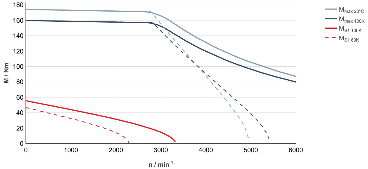
Fig. 209: MS2N10-D1BNN-___0-___-_, ctrlX DRIVE, controlled supply 3 × AC 400 ... 480 V
