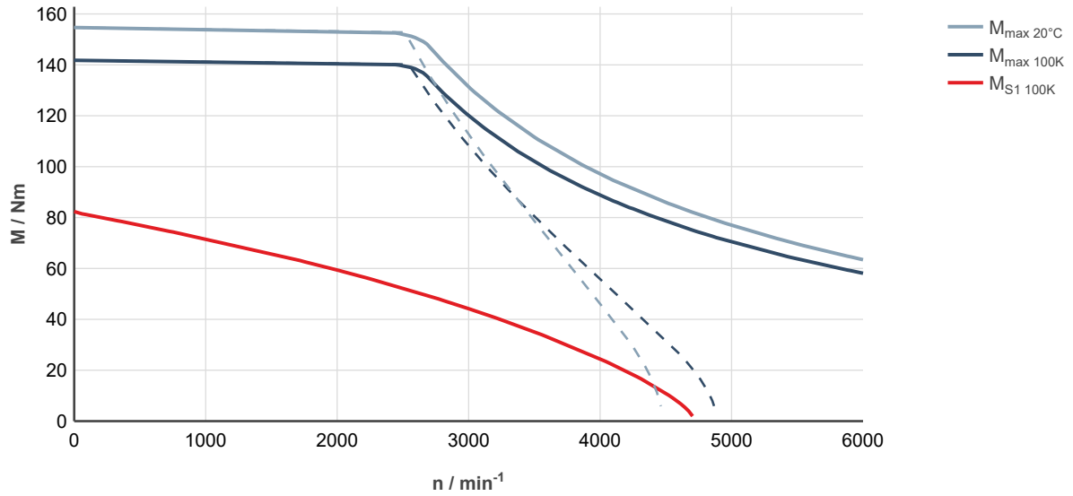
Fig. 239: MS2N10-D0BNA-___0-___-_, ctrlX DRIVE, controlled supply 3 × AC 400 ... 480 V
