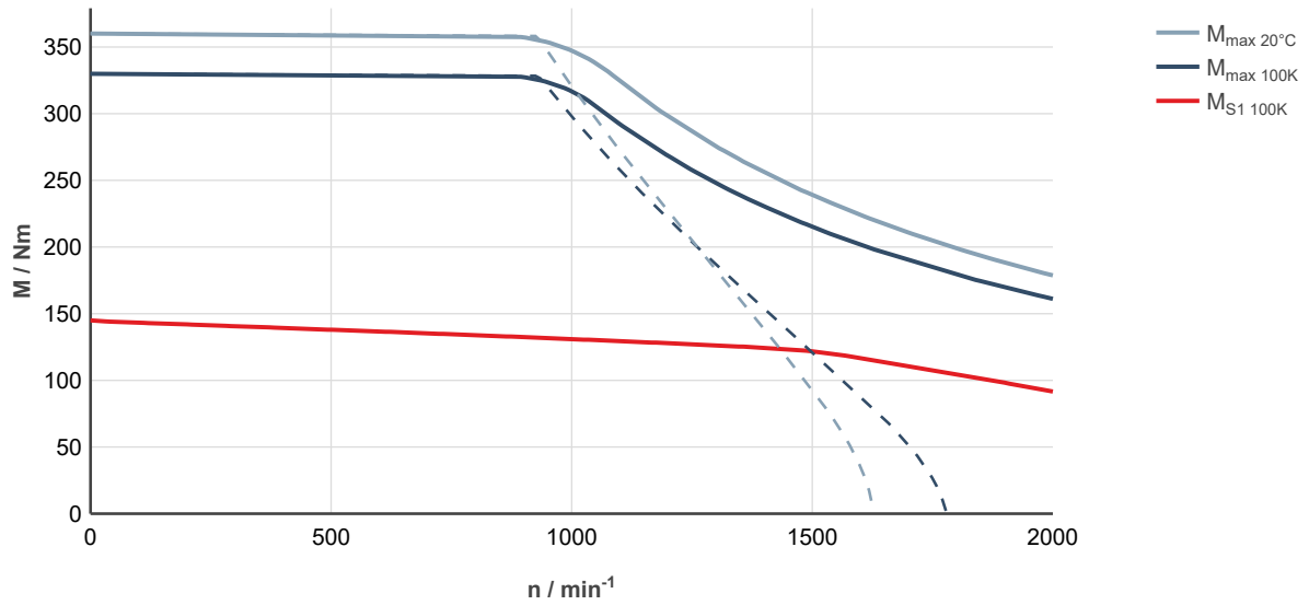
Fig. 257: MS2N10-F1BDA-___0-___-__, ctrlX DRIVE, controlled supply 3 × AC 400 ... 480 V
