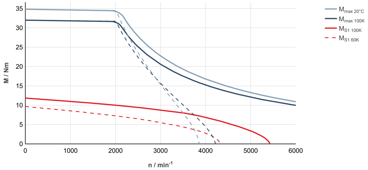
Fig. 74: MS2N06-D0BNN-___0-___-_, ctrlX DRIVE, uncontrolled supply 3 × AC 400 V
