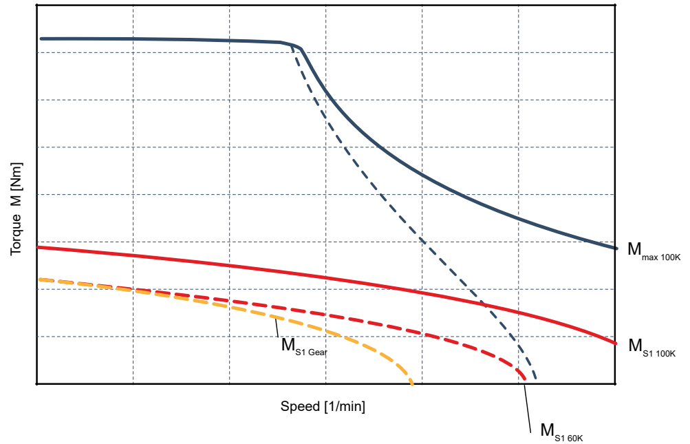
Fig. 22: S1 characteristic curve in gearbox
