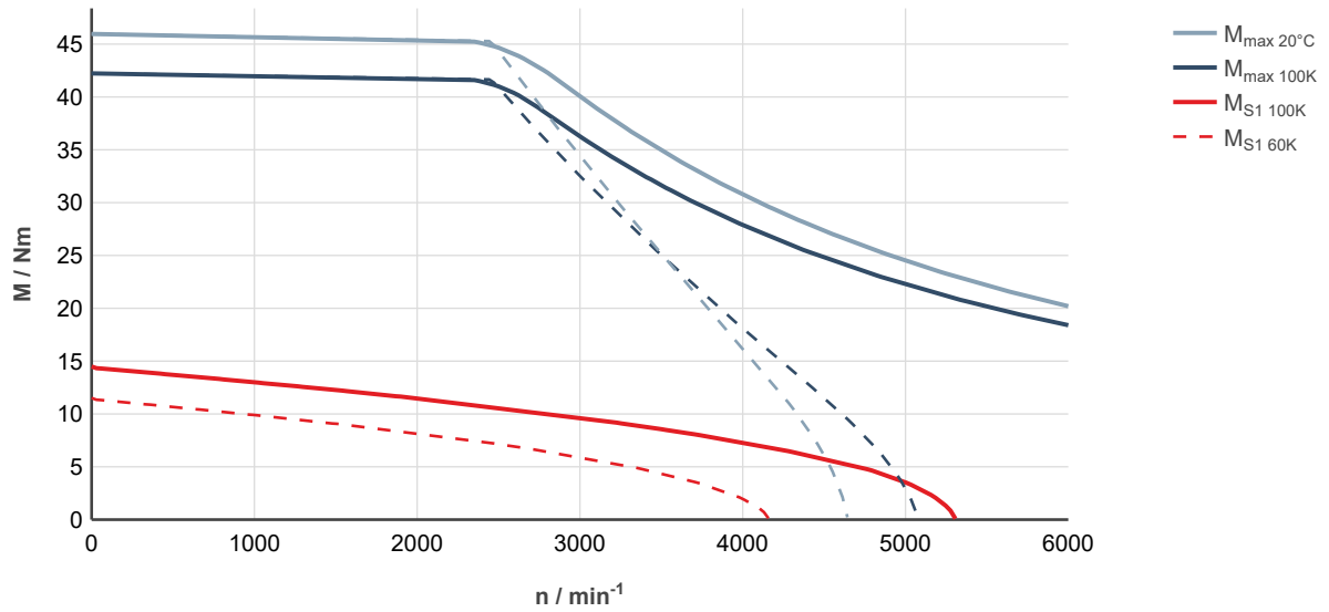
Fig. 96: MS2N07-C1BNN-___0-___-__, ctrlX DRIVE, controlled supply 3 × AC 400 ... 480 V
