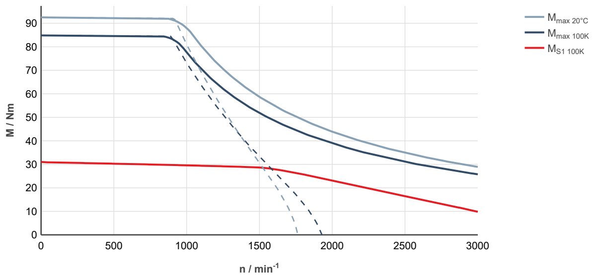
Fig. 143: MS2N07-D1BFA-___0-___-__, ctrlX DRIVE, uncontrolled supply 3 × AC 400 V
