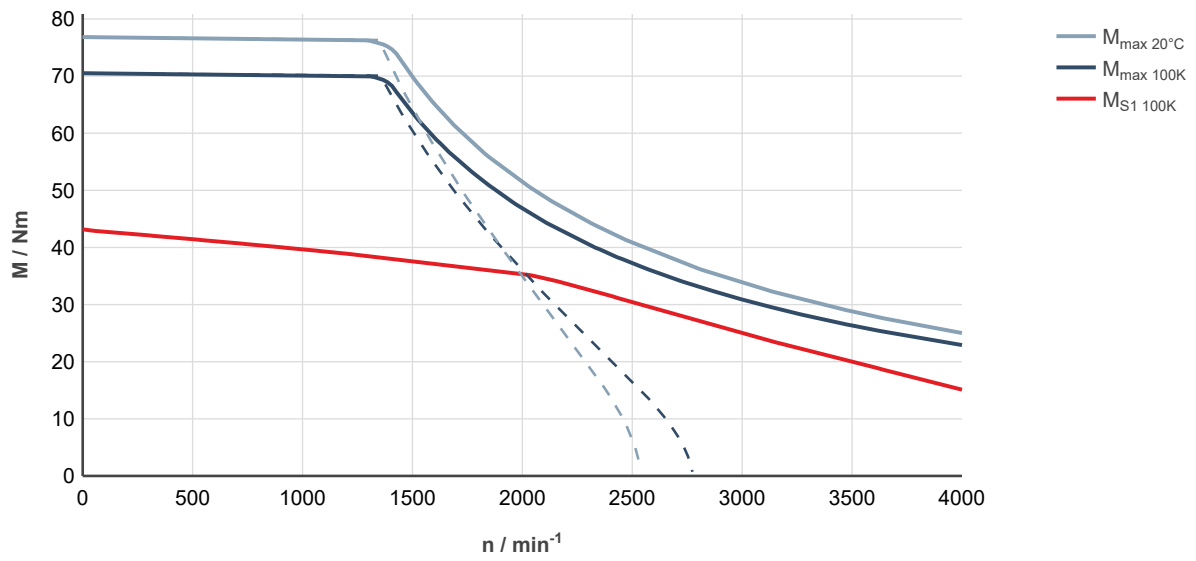
Fig. 228: MS2N10-C0BHA-___0-___-_, ctrlX DRIVE, uncontrolled supply 3 × AC 400 V
