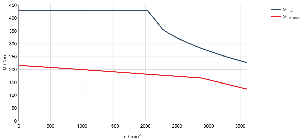
Fig. 323: MS2N13-C1BHC-___0-___-_, ctrIX DRIVE, controlled supply 3 × AC 400 ... 480 V M_{max} Characteristic curve applies to maximum torque 20 °C (cold)
