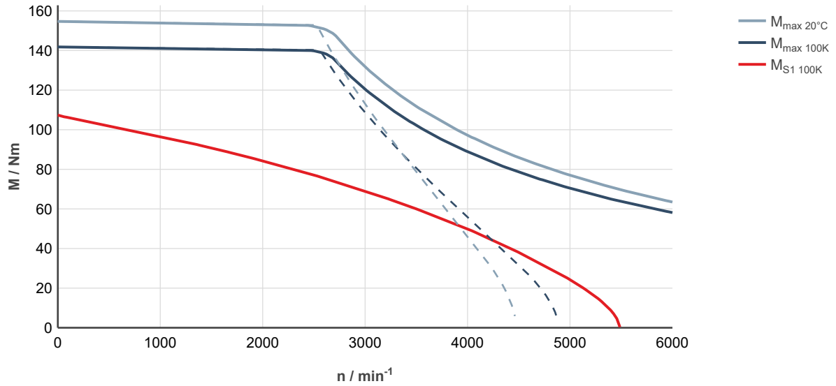
Fig. 271: MS2N10-D0BNL-___0-___-___, ctrIX DRIVE, controlled supply 3 × AC 400 ... 480 V
