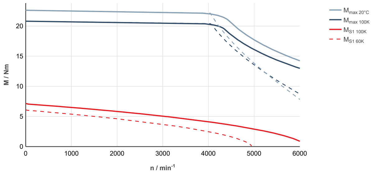
Fig. 57: MS2N05-C0BTN-___0-___-__, ctrlX DRIVE, uncontrolled supply 3 × AC 400 V
