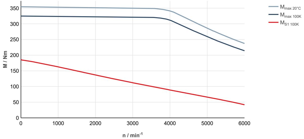
Fig. 289: MS2N10-R0BQL-__0-__-__, ctrlX DRIVE, controlled supply 3 x AC 400 ... 480 V
