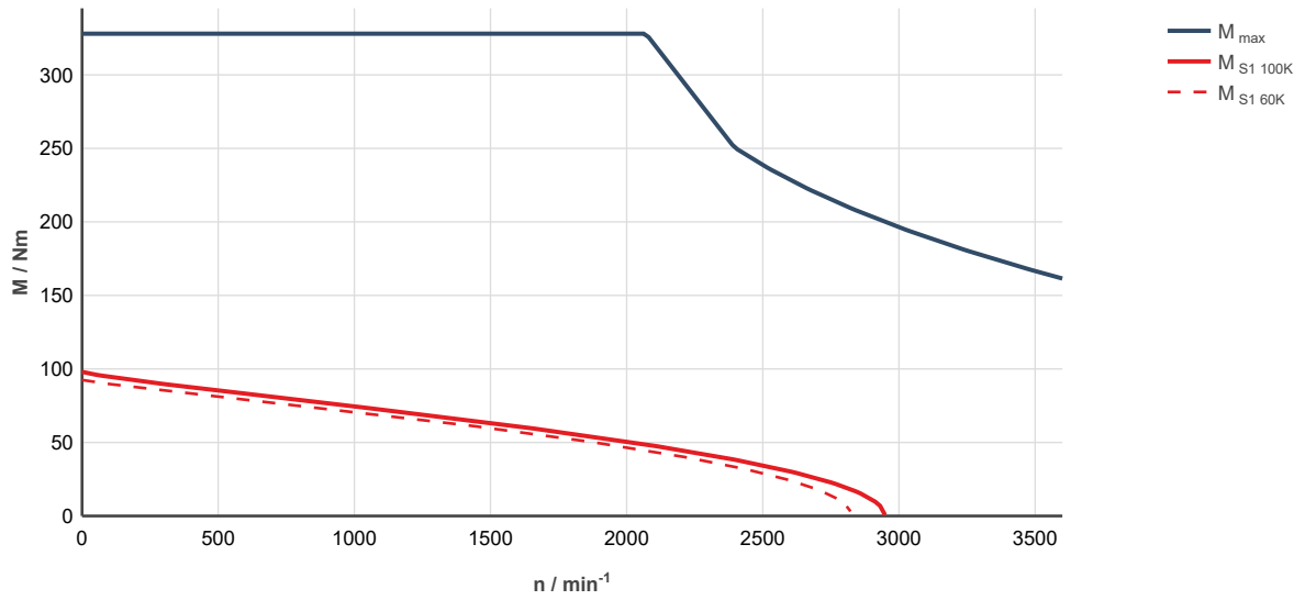
Fig. 303: MS2N13-B1BHN-___0-___-__ (modified), ctrlX DRIVE, controlled supply 3 x AC 400 br ... 480 V
