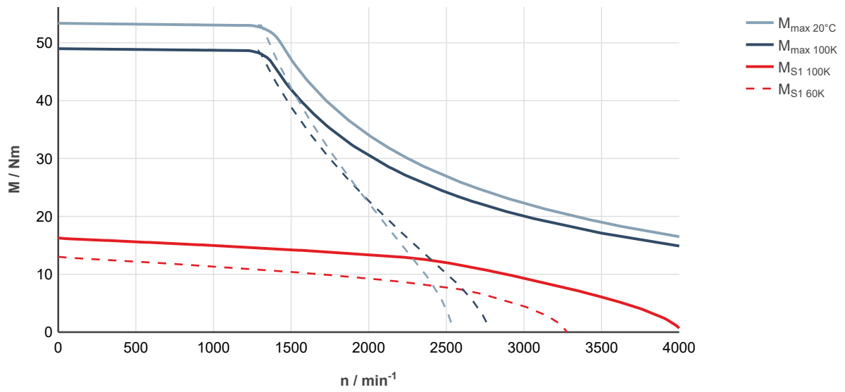
Fig. 80: MS2N06-E0BHN-___0-___-__, ctrlX DRIVE, uncontrolled supply 3 × AC 400 V
