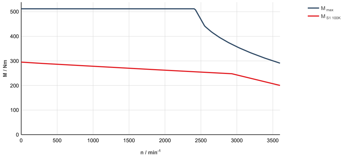
Fig. 343: MS2N13-D1BHL-__0-__-__, ctrlX DRIVE, controlled supply 3 x AC 400 ... 480 V
