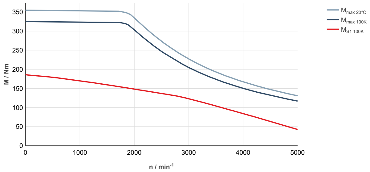
Fig. 286: MS2N10-R0BLL-__0-__-__, ctrlX DRIVE, uncontrolled supply 3 × AC 400 V
