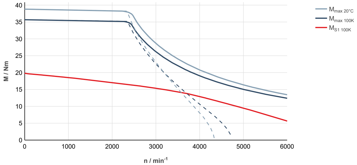
Fig. 128: MS2N07-C0BNA-___0-___-_, ctrlX DRIVE, controlled supply 3 × AC 400 ... 480 V
