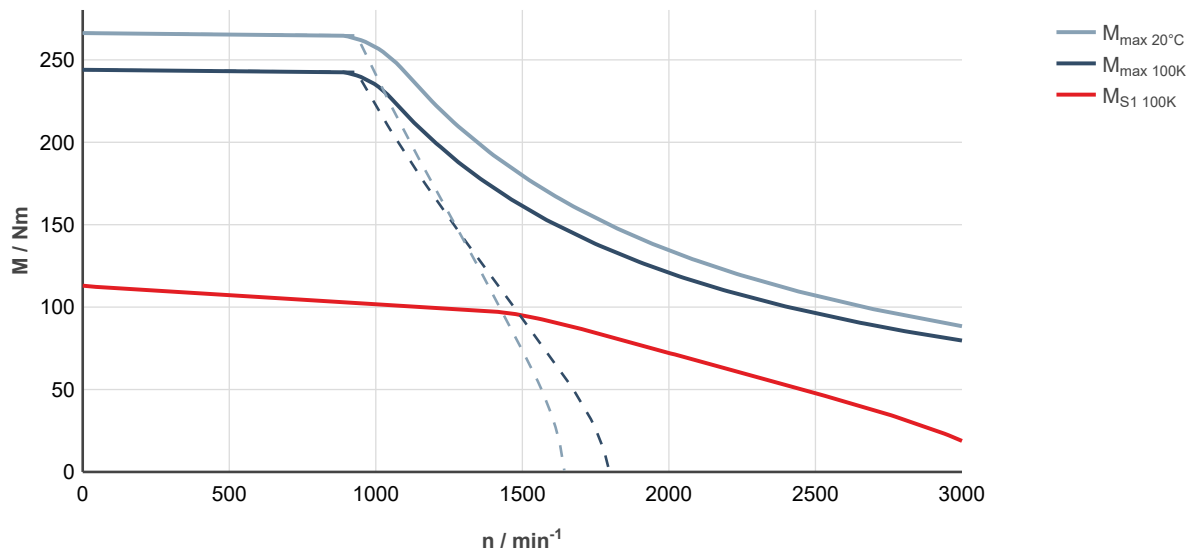
Fig. 248: MS2N10-E1BFA-___0-___-__, ctrlX DRIVE, uncontrolled supply 3 × AC 400 V
