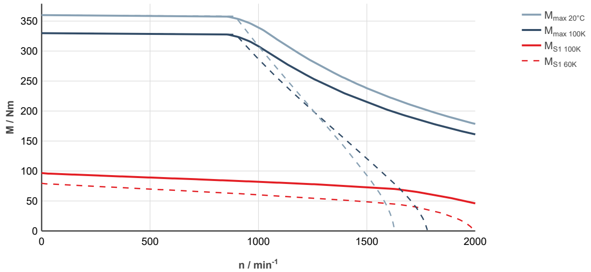
Fig. 223: MS2N10-F1BDN-___0-___-_, ctrlX DRIVE, controlled supply 3 × AC 400 ... 480 V
