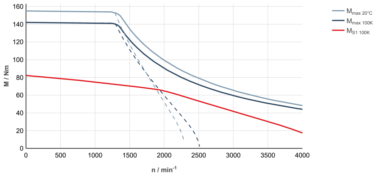
Fig. 236: MS2N10-D0BHA-___0-___-_, ctrlX DRIVE, uncontrolled supply 3 × AC 400 V
