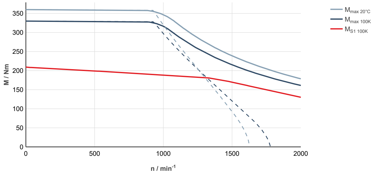
Fig. 283: MS2N10-F1BDL-___0-___-__, ctrlX DRIVE, controlled supply 3 × AC 400 ... 480 V
