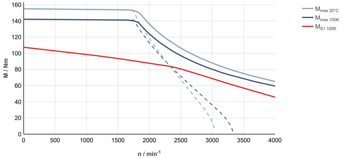
Fig. 269: MS2N10-D0BHL-___0-___-___, ctrIX DRIVE, controlled supply 3 × AC 400 ... 480 V
