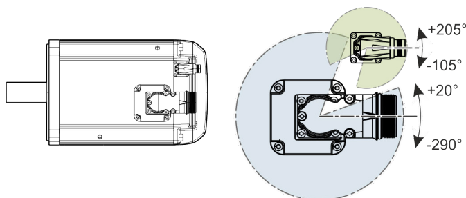
Fig. 368: Rotating area electrical connection "V"
