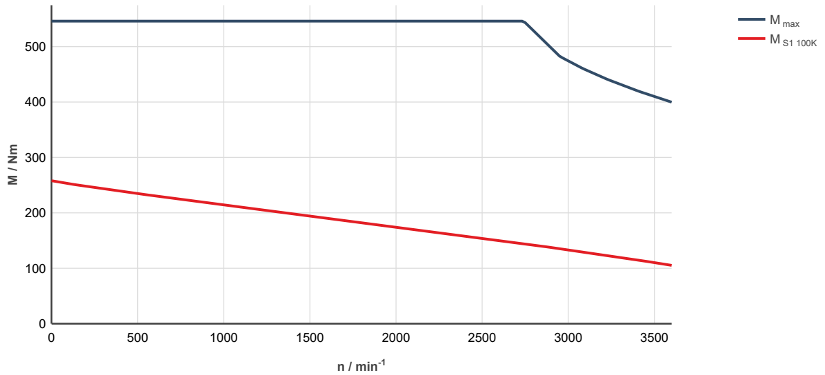
Fig. 329: MS2N13-D1BNC-___0-___-_, ctrlX DRIVE, controlled supply 3 x AC 400 ... 480 V
