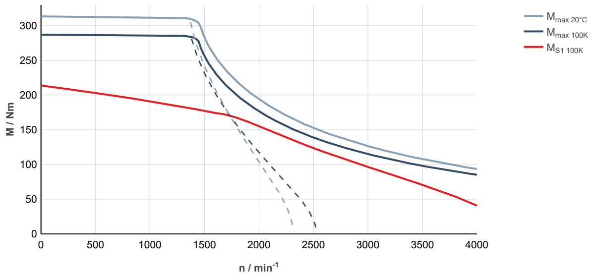
Fig. 280: MS2N10-F0BHL-___0-___-__, ctrlX DRIVE, uncontrolled supply 3 × AC 400 V
