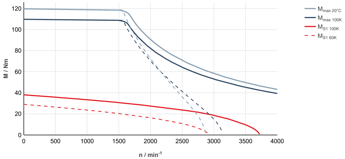
Fig. 114: MS2N07-E0BDN-___0-___-__, ctrlX DRIVE, controlled supply 3 × AC 400 ... 480 V
