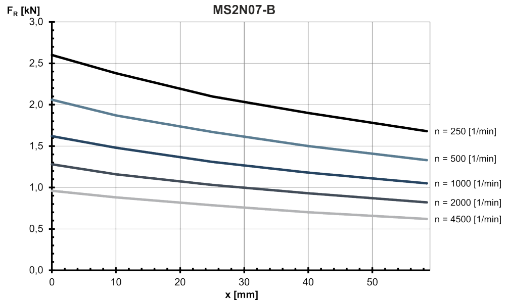
Fig. 188: MS2N07-B: Radial force in distance x from the shaft shoulder at a nominal bearing service life of L_{h10} = 30000 h
