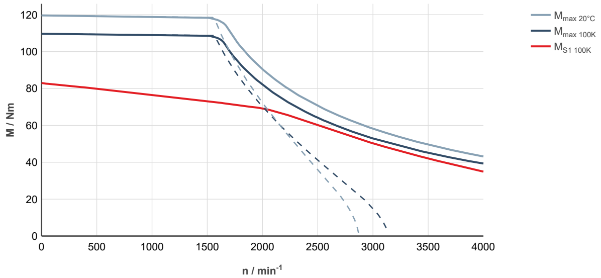
Fig. 178: MS2N07-E0BHL-___0-___-___, ctrlX DRIVE, controlled supply 3 × AC 400 ... 480 V
