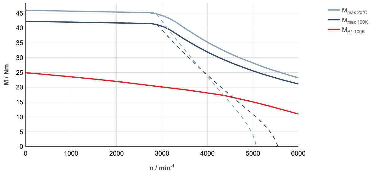
Fig. 167: MS2N07-C1BRL-___0-___-__, ctrlX DRIVE, uncontrolled supply 3 × AC 400 V
