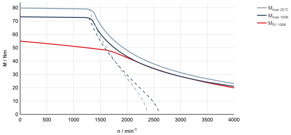
Fig. 169: MS2N07-D0BHL-___0-___-___, ctrIX DRIVE, uncontrolled supply 3 × AC 400 V
