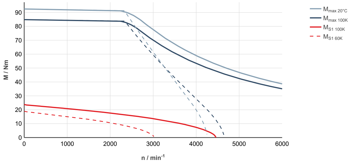
Fig. 112: MS2N07-D1BNN-___0-___-, ctrlX DRIVE, controlled supply 3 × AC 400 ... 480 V
