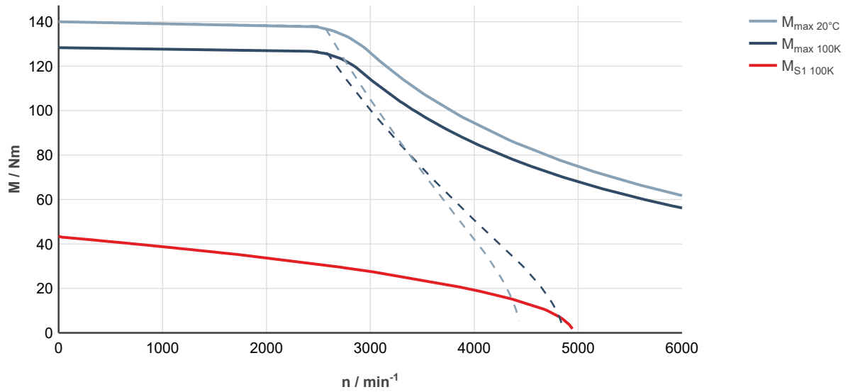
Fig. 162: MS2N07-E1BNA-___0-___-__, ctrlX DRIVE, controlled supply 3 × AC 400 ... 480 V
