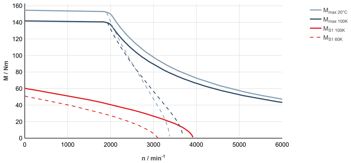
Fig. 204: MS2N10-D0BNN-___0-___-_, ctrlX DRIVE, uncontrolled supply 3 × AC 400 V
