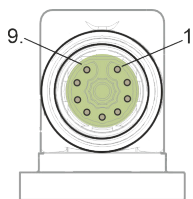
Fig. 366: Connector view of M17 encoder connector
