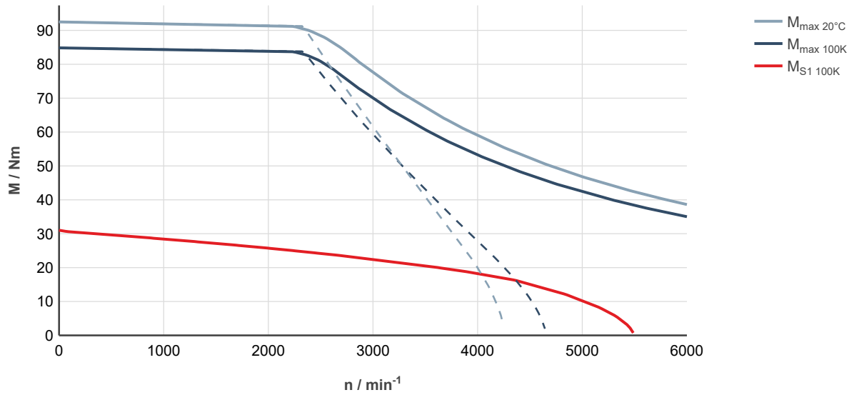
Fig. 148: MS2N07-D1BNA-___0-___- , ctrlX DRIVE, controlled supply 3 × AC 400 ... 480 V
