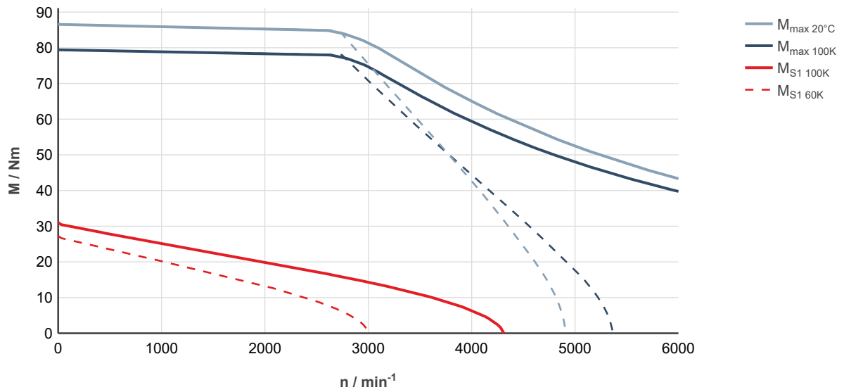
Fig. 201: MS2N10-C1BNN-___0-___-_, ctrlX DRIVE, controlled supply 3 × AC 400 ... 480 V
