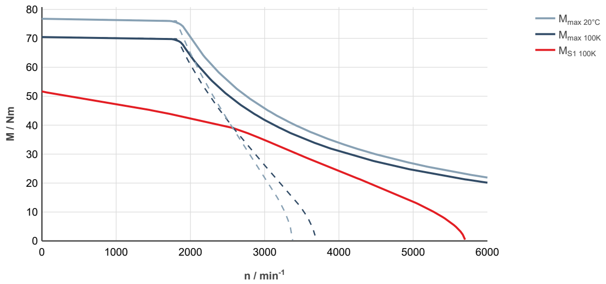
Fig. 264: MS2N10-C0BNL-___0-___-___, ctrIX DRIVE, uncontrolled supply 3 × AC 400 V
