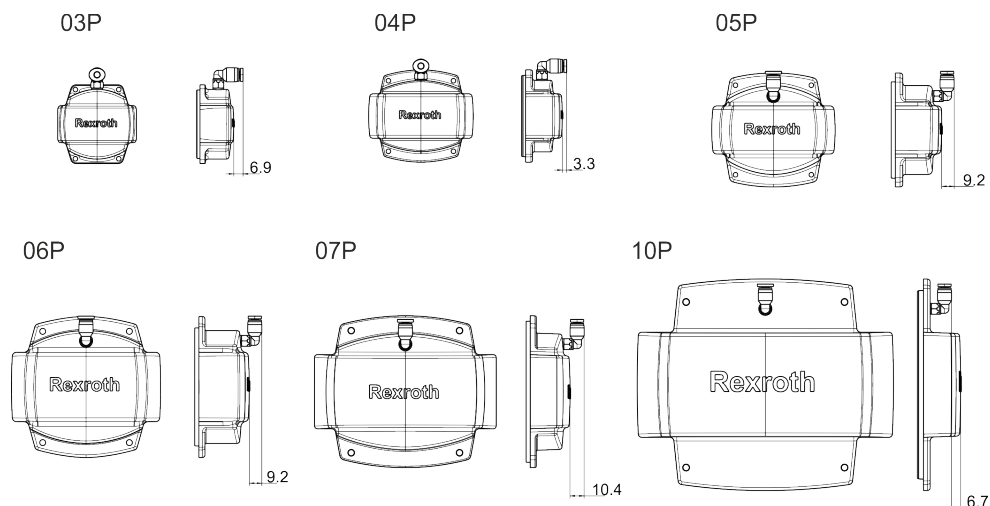
Fig. 17: Sealing air connection variants
