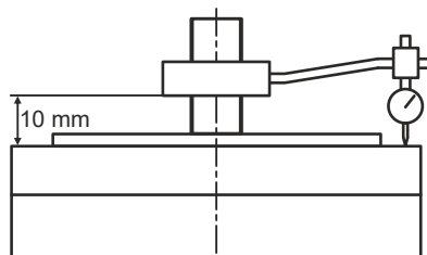
Fig. 15: Measuring system of alignment The coaxiality and the alignment are measured in vertical motor position to exclude the influence of gravitational forces.
