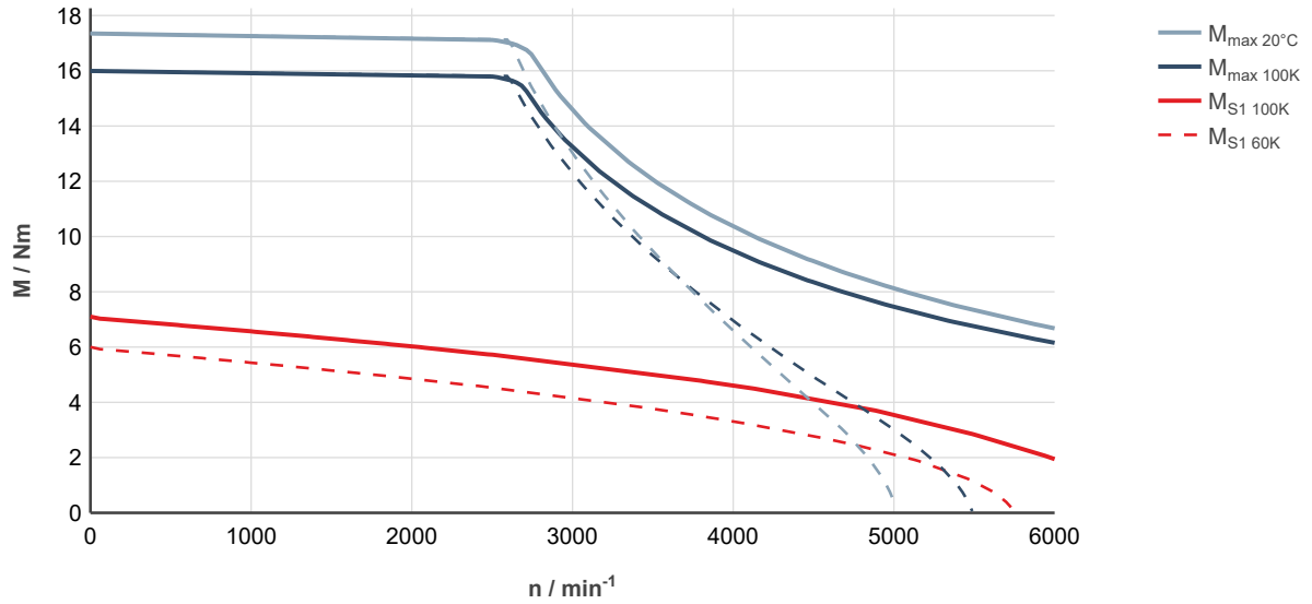
Fig. 71: MS2N06-C0BNN-___0-___-_, ctrlX DRIVE, controlled supply 3 × AC 400 ... 480 V
