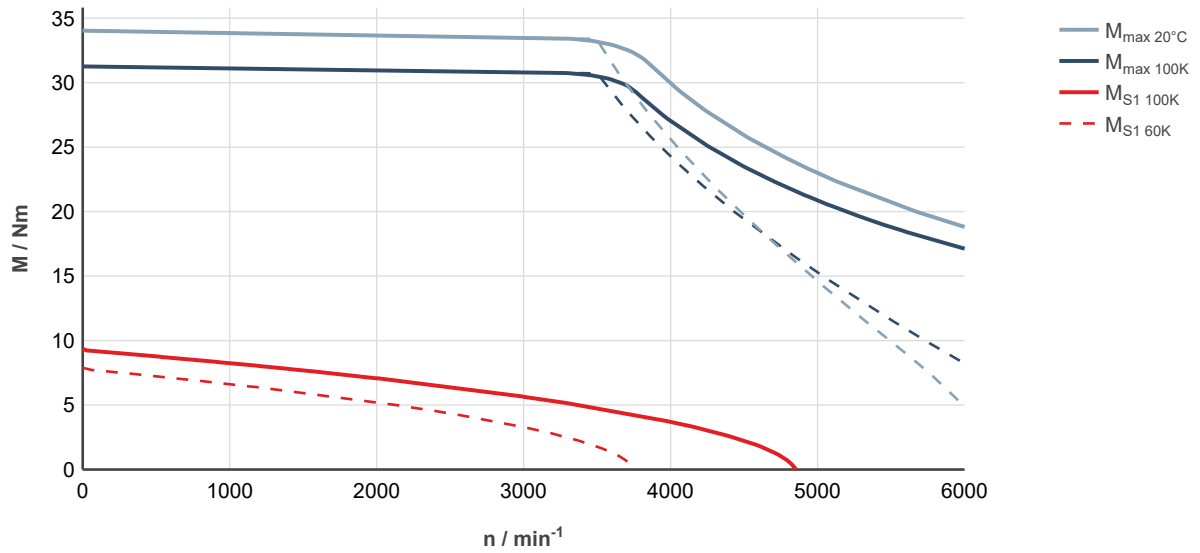
Fig. 62: MS2N05-D0BRN-___0-___-__, ctrlX DRIVE, controlled supply 3 × AC 400 ... 480 V
