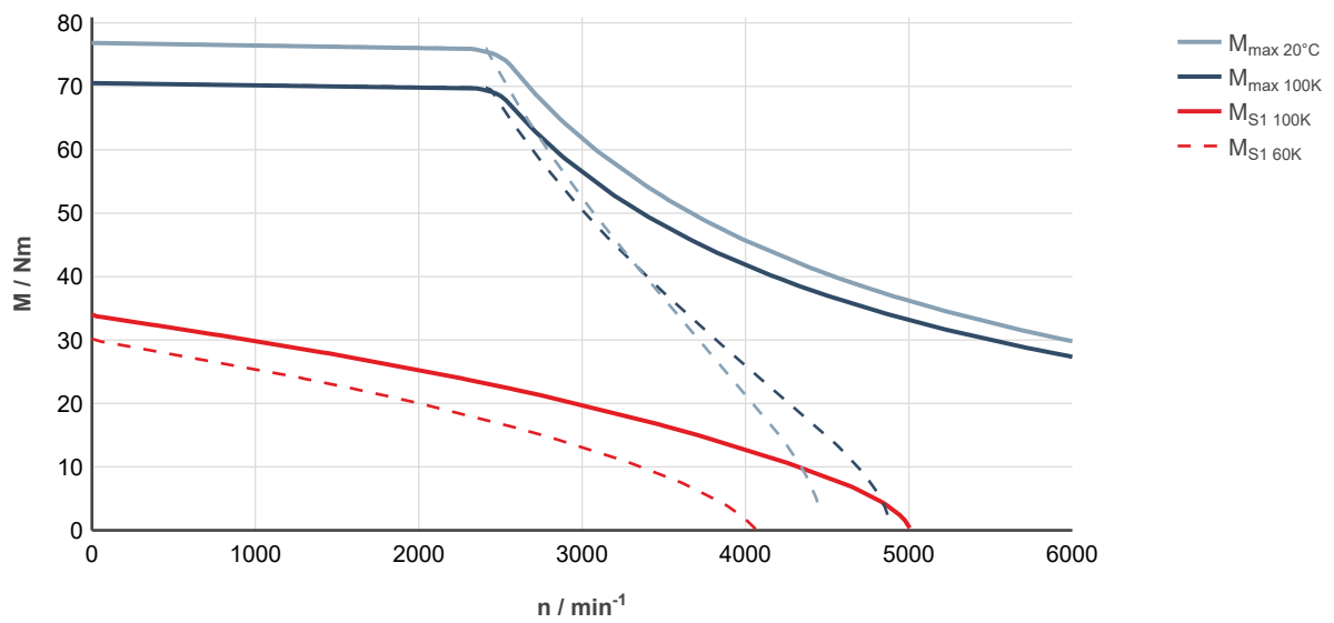
Fig. 197: MS2N10-C0BNN-___0-___- , ctrlX DRIVE, controlled supply 3 × AC 400 ... 480 V
