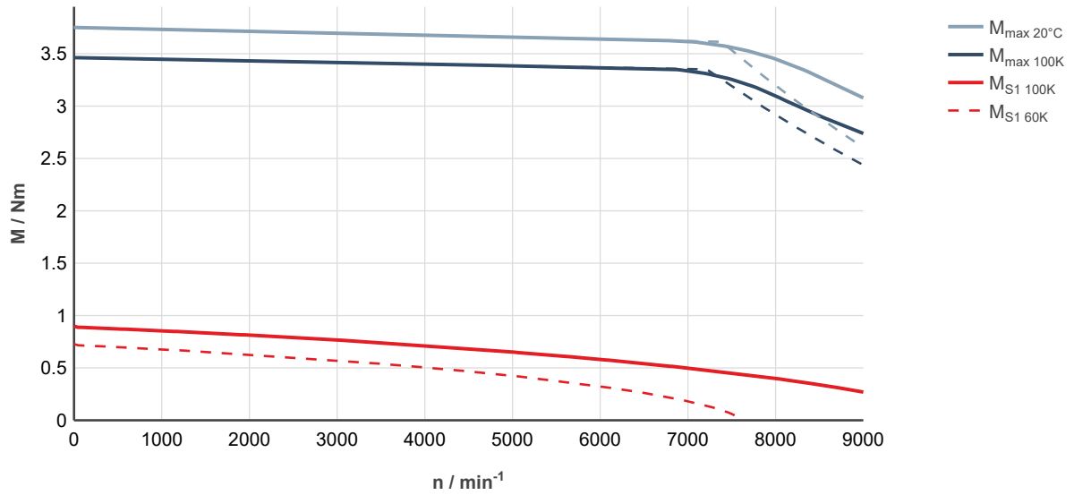
Fig. 26: MS2N03-B0BYN-___0-___-_, ctrlX DRIVE, controlled supply 3 × AC 400 ... 480 V
