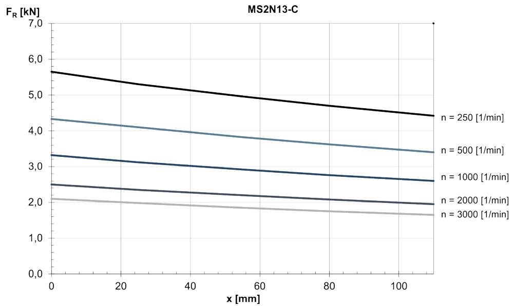
Fig. 354: MS2N13-C: Radial force in distance x from the shaft shoulder at a nominal bearing service life of L_{h10} = 30000 h
