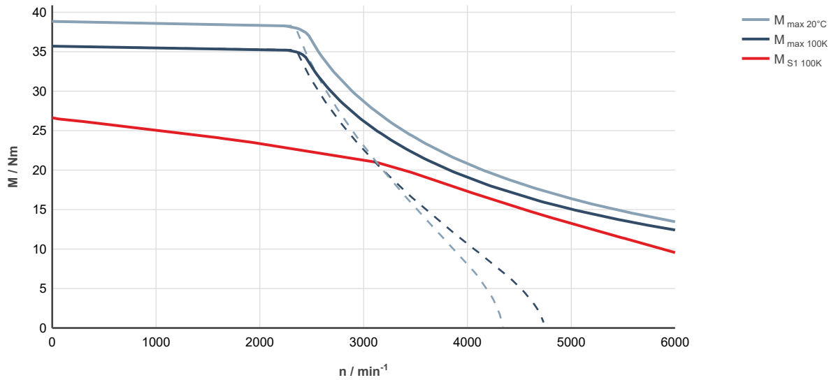
Fig. 164: MS2N07-C0BNL-___0-___-___, ctrIX DRIVE, controlled supply 3 x AC 400 ... 480 V
