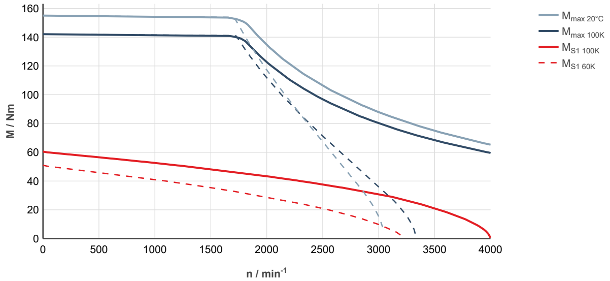
Fig. 203: MS2N10-D0BHN-___0-___-, ctrlX DRIVE, controlled supply 3 × AC 400 ... 480 V
