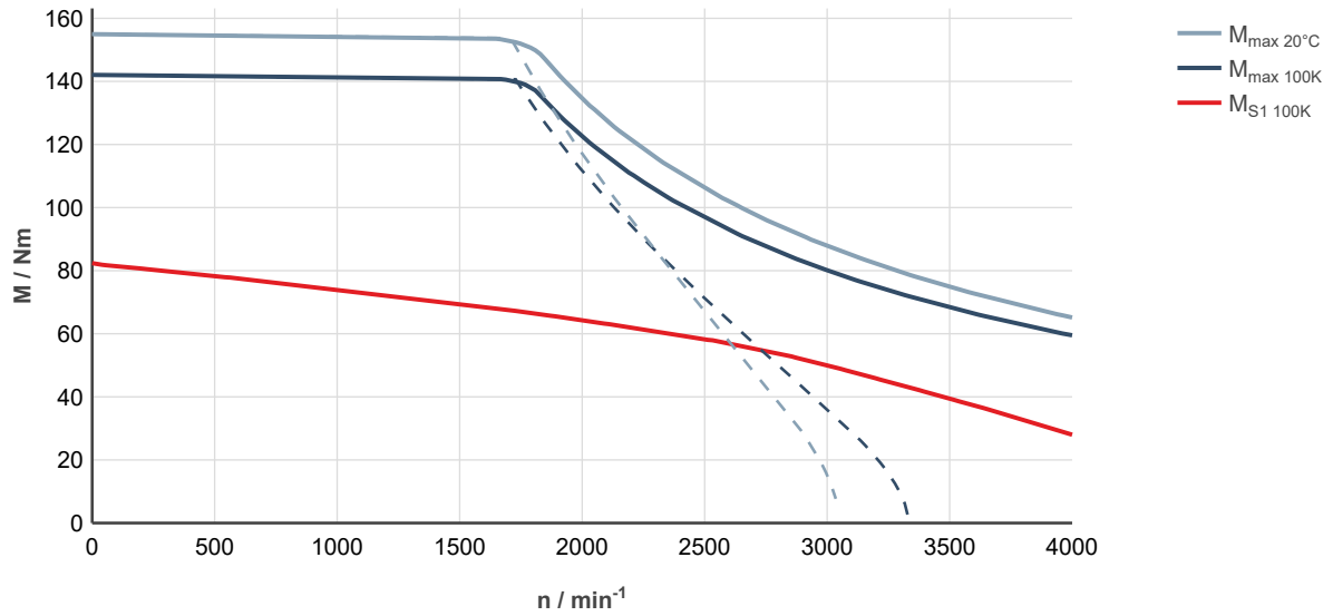
Fig. 237: MS2N10-D0BHA-___0-___-_, ctrlX DRIVE, controlled supply 3 × AC 400 ... 480 V
