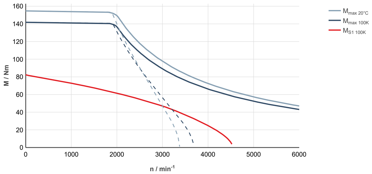
Fig. 238: MS2N10-D0BNA-___0-___-_, ctrlX DRIVE, uncontrolled supply 3 × AC 400 V
