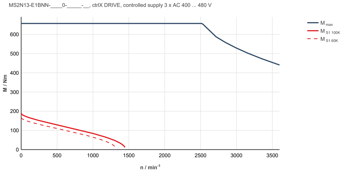
Fig. 317: MS2N13-E1BNN-___0-___-___, ctrlX DRIVE, controlled supply 3 x AC 400 ... 480 V
