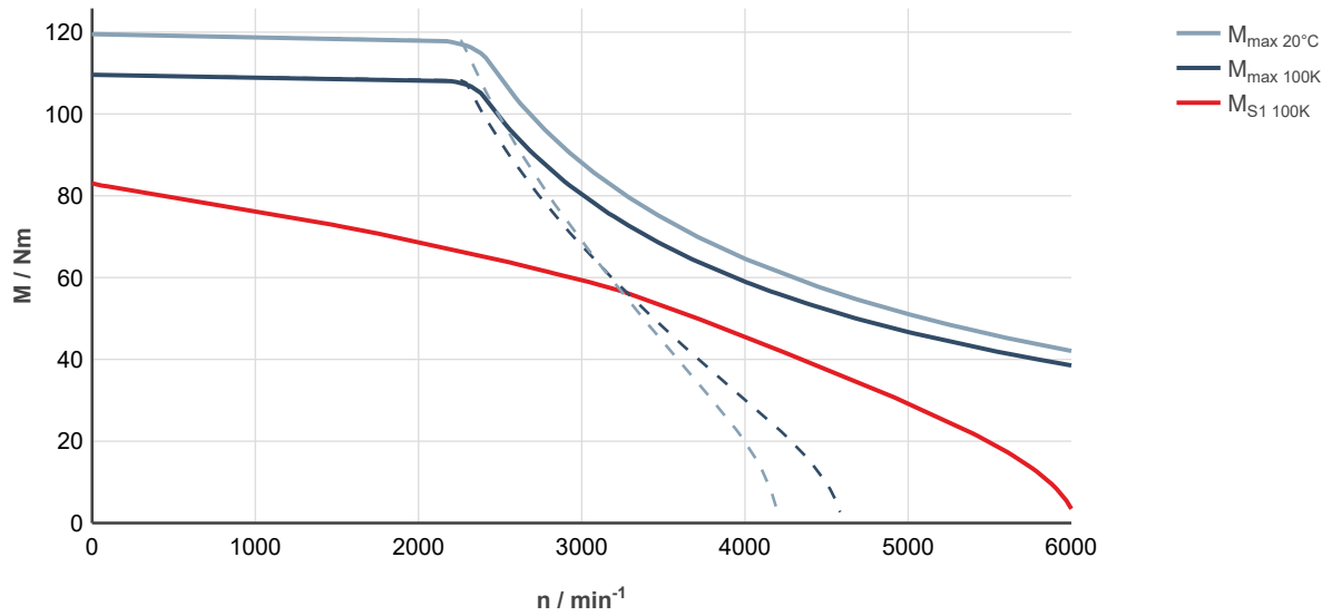
Fig. 180: MS2N07-E0BNL-___0-___-___, ctrlX DRIVE, controlled supply 3 × AC 400 ... 480 V
