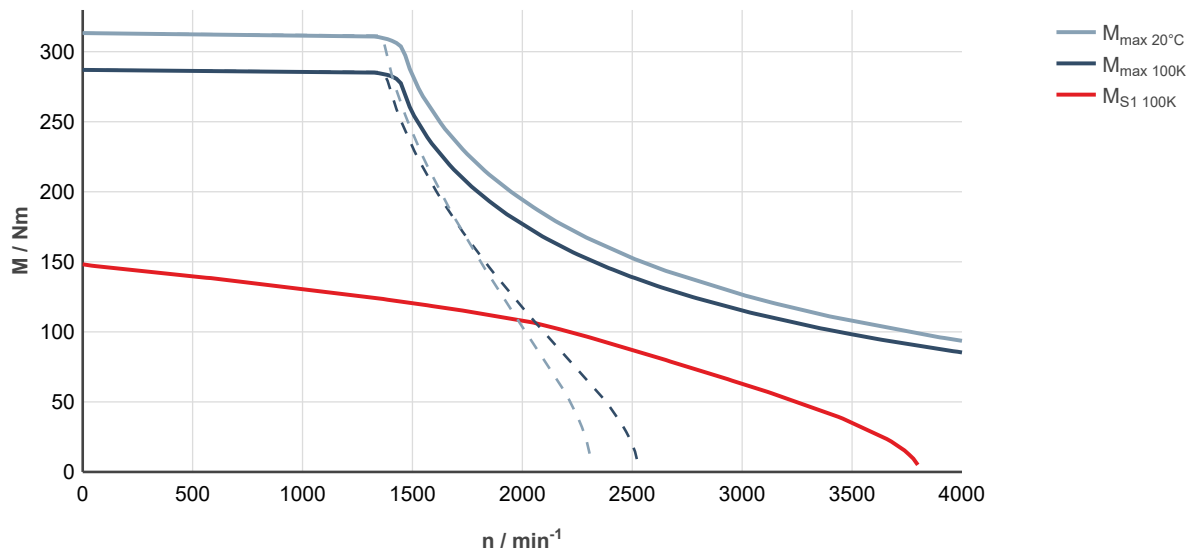
Fig. 254: MS2N10-F0BHA-___0-___-_, ctrIX DRIVE, uncontrolled supply 3 × AC 400 V
