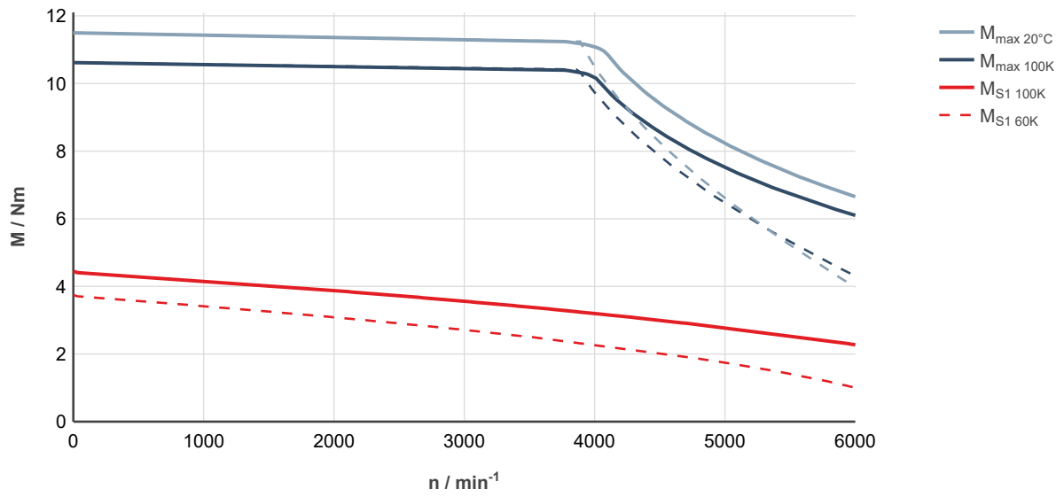
Fig. 53: MS2N05-B0BTN-___0-___-__, ctrlX DRIVE, uncontrolled supply 3 × AC 400 V
