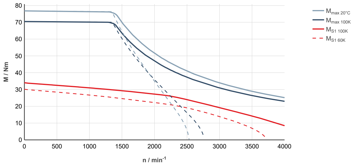
Fig. 194: MS2N10-C0BHN-___0-___-_, ctrlX DRIVE, uncontrolled supply 3 × AC 400 V
