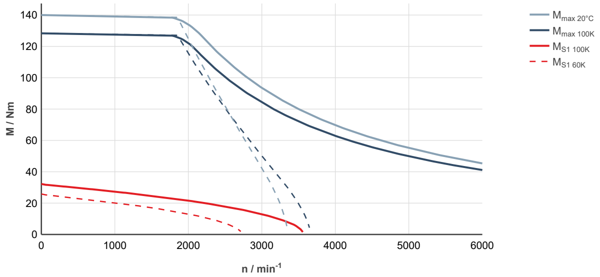
Fig. 125: MS2N07-E1BNN-___0-___-_, ctrlX DRIVE, uncontrolled supply 3 × AC 400 V
