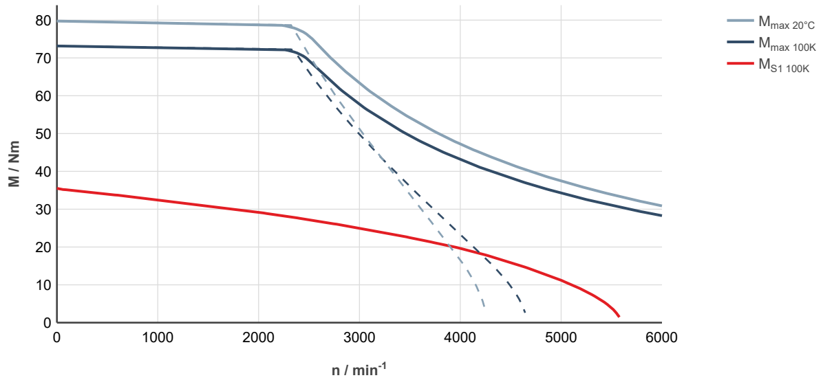
Fig. 140: MS2N07-D0BNA-___0-___-_, ctrlX DRIVE, controlled supply 3 × AC 400 ... 480 V
