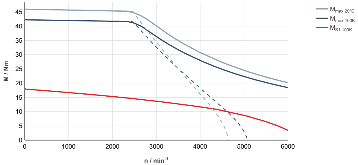
Fig. 132: MS2N07-C1BNA-___0-___-_, ctrlX DRIVE, controlled supply 3 × AC 400 ... 480 V
