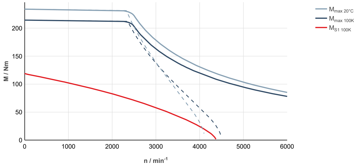
Fig. 247: MS2N10-E0BNA-___0-___-__, ctrlX DRIVE, controlled supply 3 × AC 400 ... 480 V
