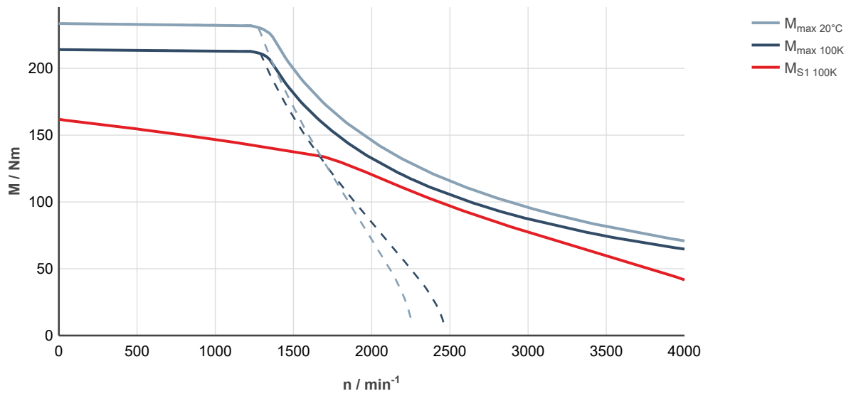
Fig. 274: MS2N10-E0BHL-___0-___-__, ctrlX DRIVE, uncontrolled supply 3 × AC 400 V
