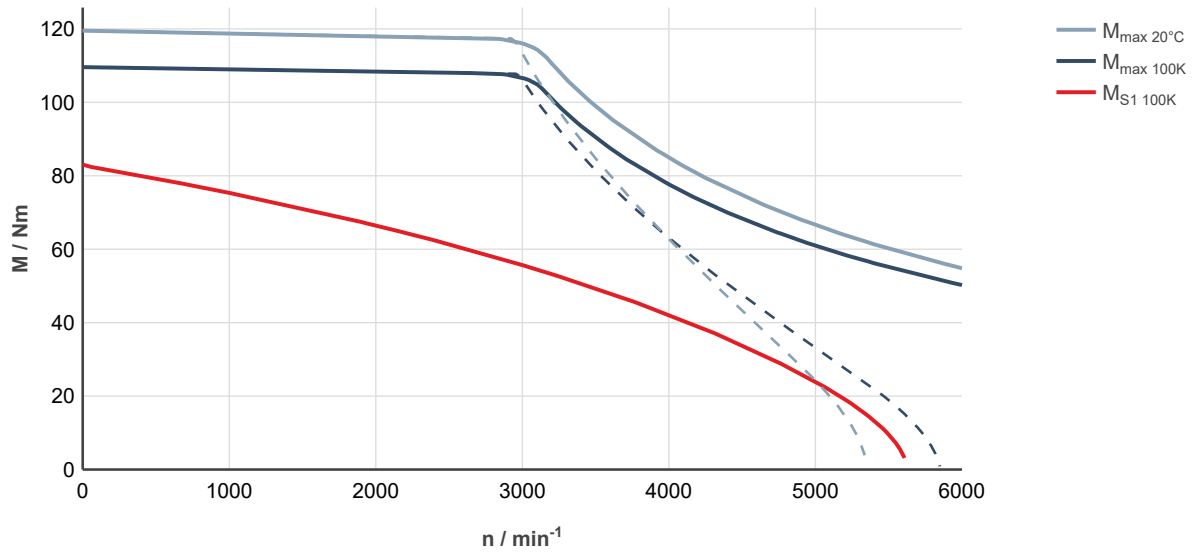
Fig. 182: MS2N07-E0BQL-___0-___-___, ctrIX DRIVE, controlled supply 3 × AC 400 ... 480 V
