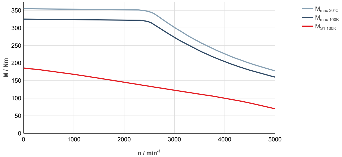
Fig. 287: MS2N10-R0BLL-__0-__-__, ctrlX DRIVE, controlled supply 3 x AC 400 ... 480 V
