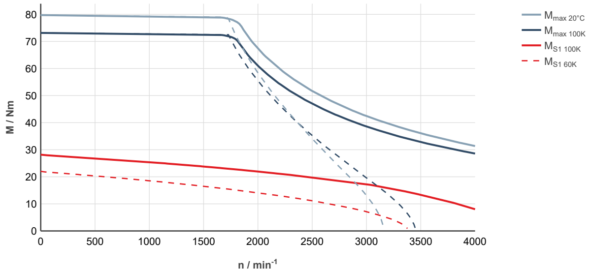
Fig. 102: MS2N07-D0BHN-___0-___-_, ctrlX DRIVE, controlled supply 3 × AC 400 ... 480 V
