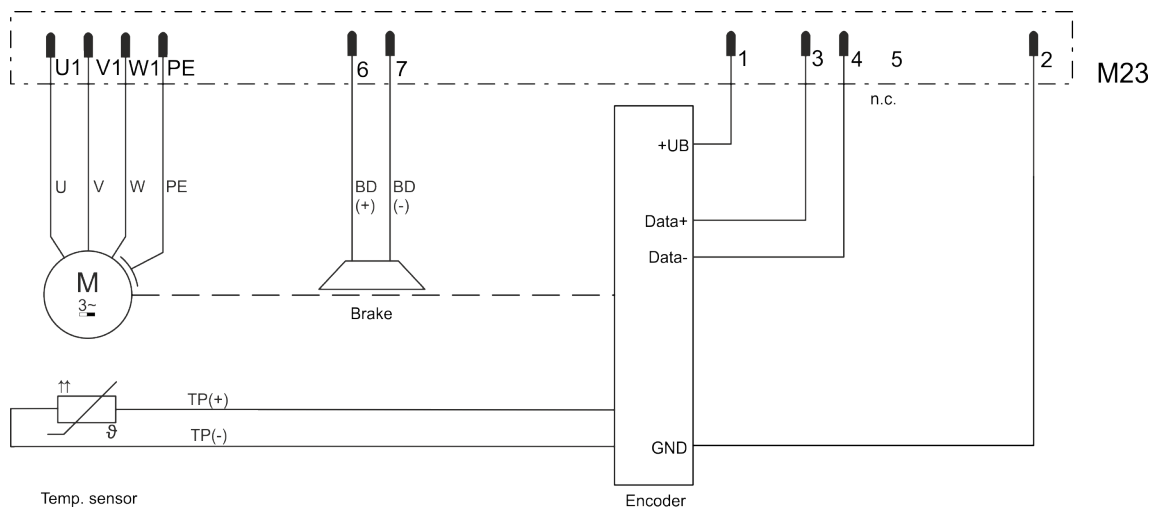
Fig. 358: M23 Single cable connection, digital encoder C, D, H, optional brake
