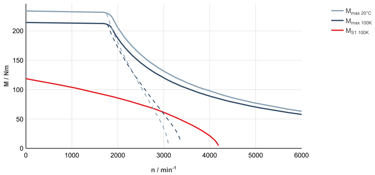
Fig. 246: MS2N10-E0BNA-___0-___-__, ctrlX DRIVE, uncontrolled supply 3 × AC 400 V
