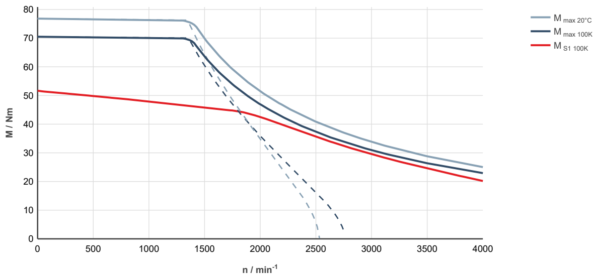
Fig. 262: MS2N10-C0BHL-___0-___-_0, ctrlX DRIVE, uncontrolled supply 3 × AC 400 V
