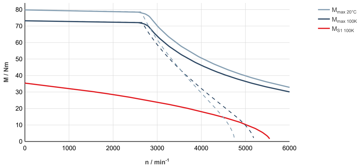
Fig. 141: MS2N07-D0BRA-___0-___-_, ctrlX DRIVE, uncontrolled supply 3 × AC 400 V
