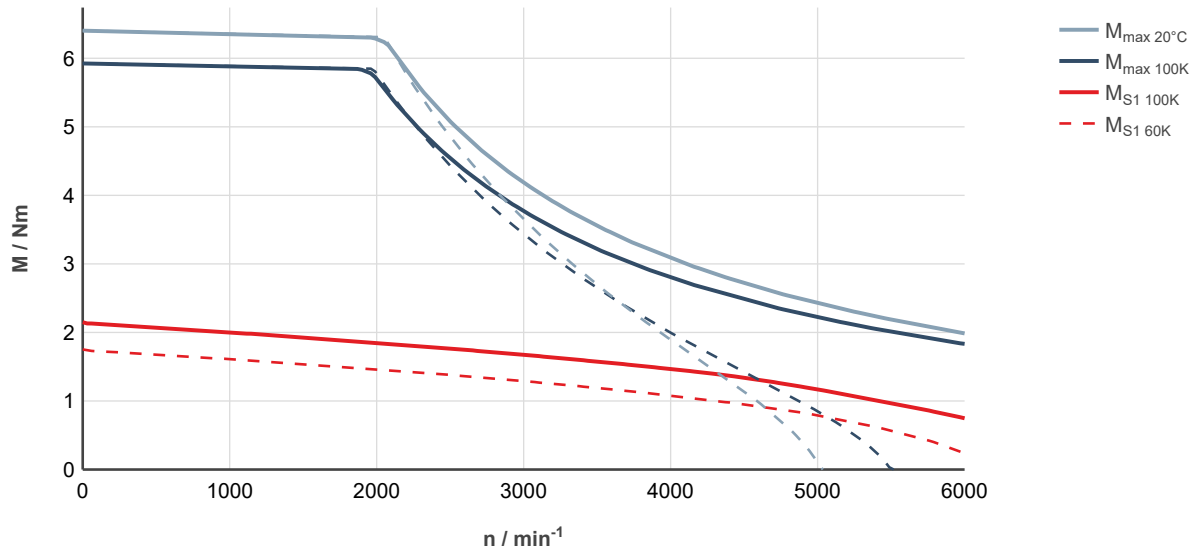
Fig. 35: MS2N04-B0BNN-___0-___-___, ctrlX DRIVE, controlled supply 3 × AC 400 ... 480 V
