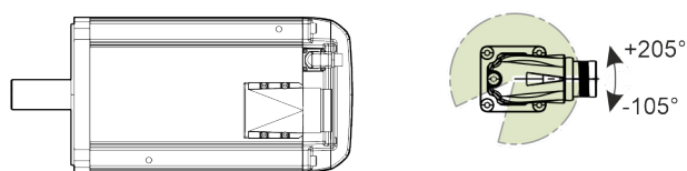
Fig. 369: Rotating area electrical connection “A/B”
