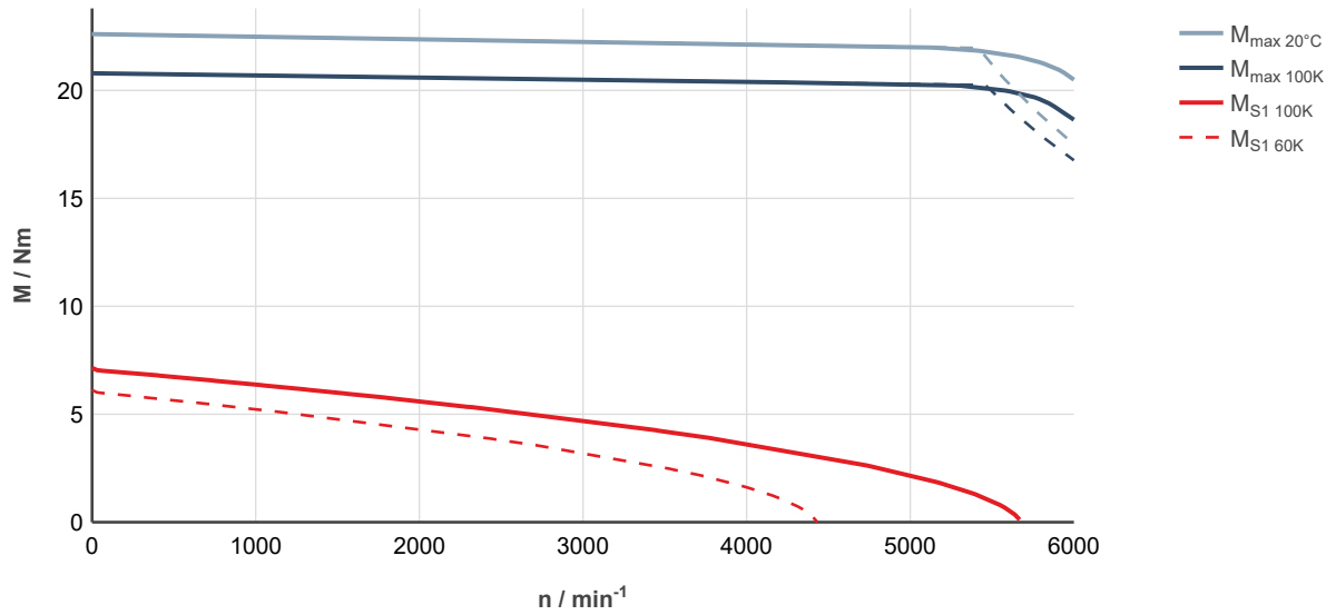
Fig. 58: MS2N05-C0BTN-___0-___-__, ctrlX DRIVE, controlled supply 3 × AC 400 ... 480 V
