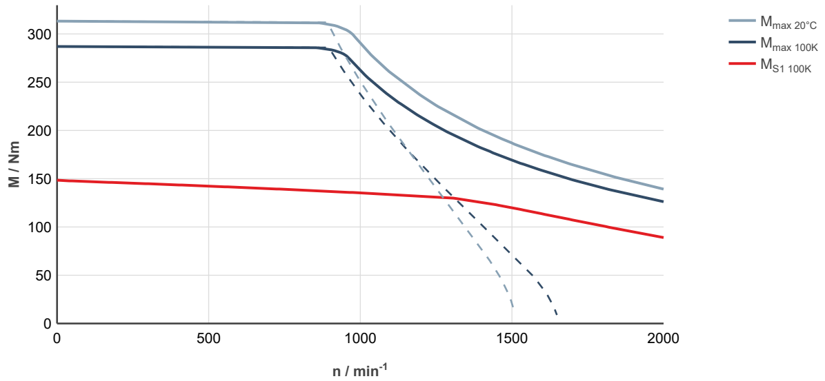
Fig. 253: MS2N10-F0BDA-___0-___-_, ctrlX DRIVE, controlled supply 3 × AC 400 ... 480 V
