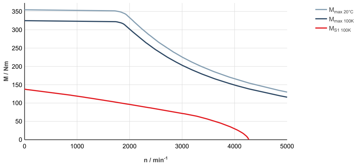
Fig. 260: MS2N10-R0BLA-___0-___-__, ctrlX DRIVE, uncontrolled supply 3 × AC 400 V
