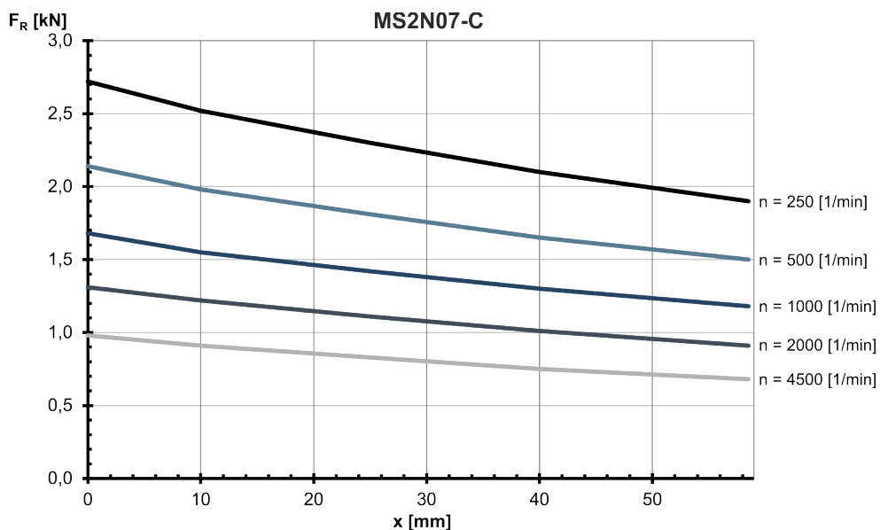
Fig. 189: MS2N07-C: Radial force in distance x from the shaft shoulder at a nominal bearing service life of L_{h10} = 30000 h
