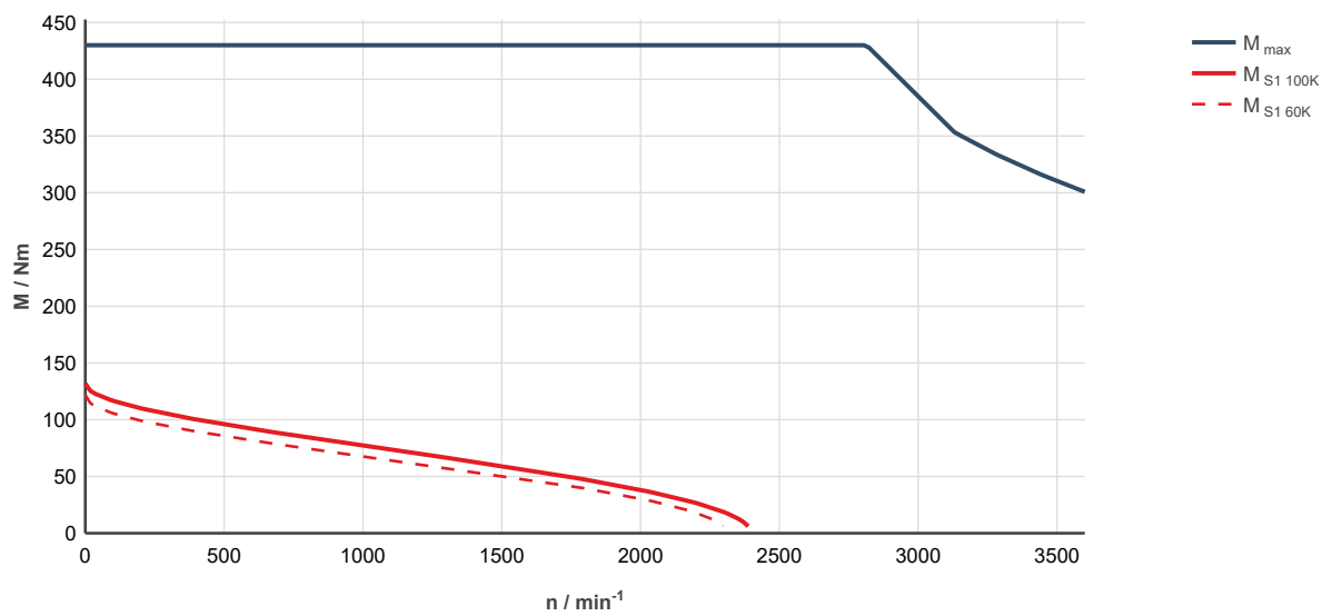
Fig. 309: MS2N13-C1BNN-___0-___-_, ctrlX DRIVE, controlled supply 3 x AC 400 ... 480 V
