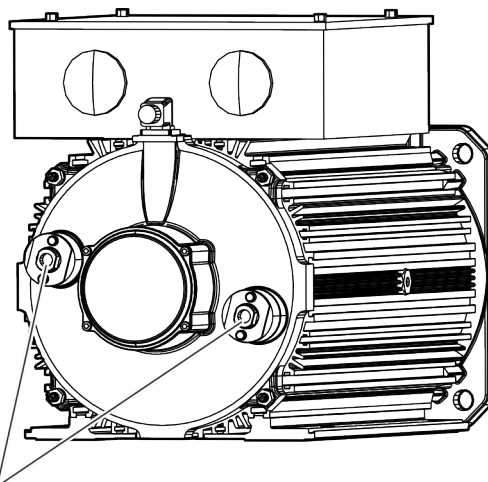
Fig. 394: Coolant connection MS2N13-__L__E__
