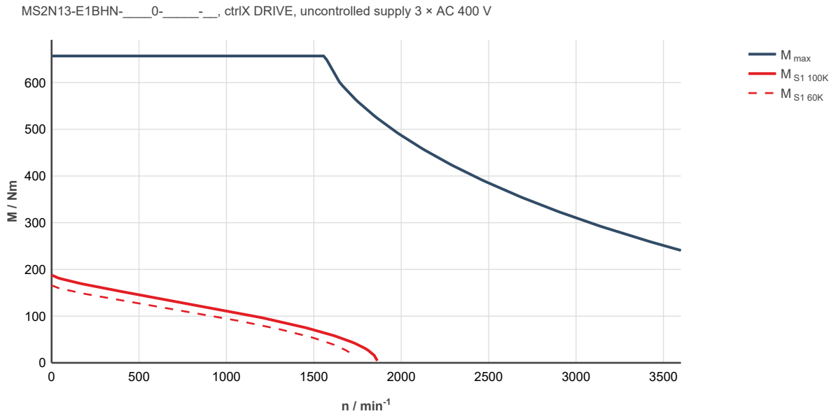
Fig. 314: MS2N13-E1BHN-___0-___-___, ctrlX DRIVE, uncontrolled supply 3 × AC 400 V
