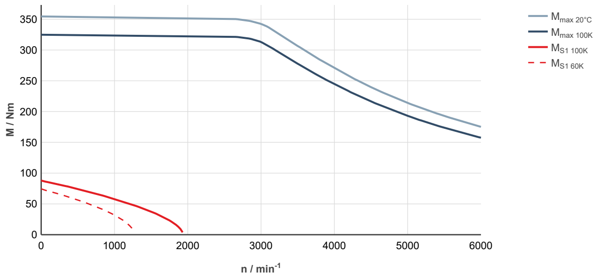
Fig. 226: MS2N10-R0BQN-___0-N___-, ctrlX DRIVE, uncontrolled supply 3 × AC 400 V
