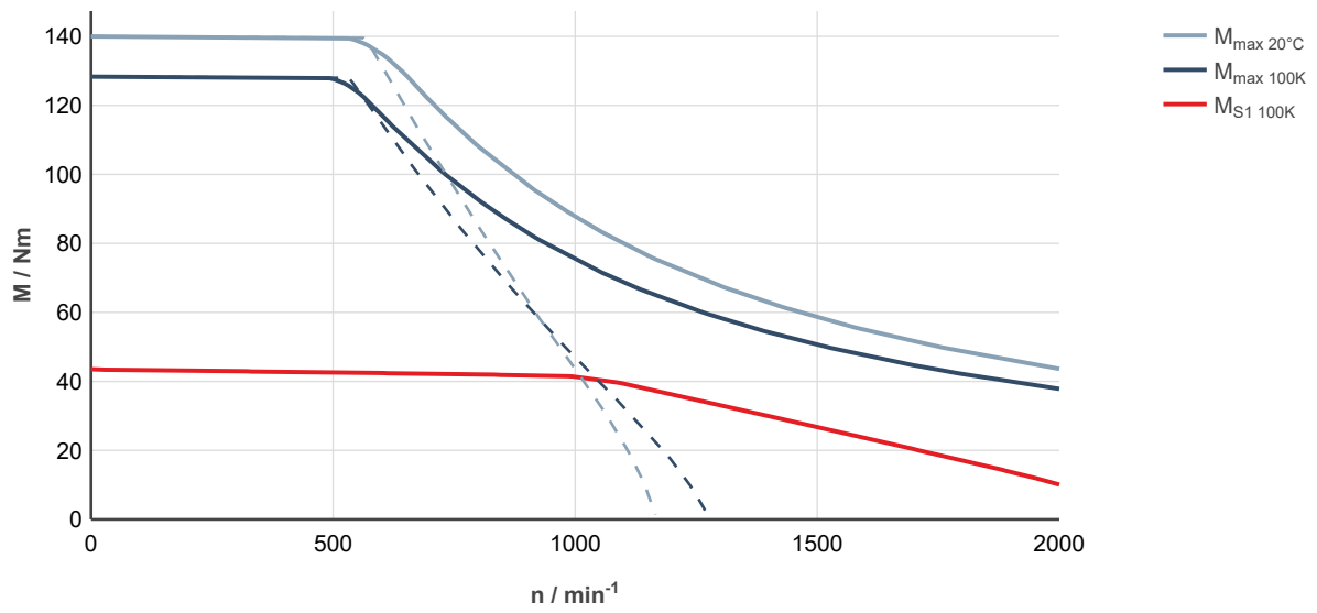
Fig. 157: MS2N07-E1BDA-___0-___-_, ctrlX DRIVE, uncontrolled supply 3 × AC 400 V
