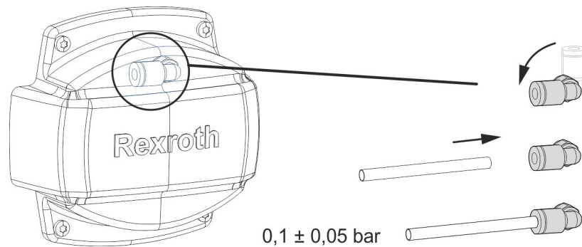
Fig. 397: Connection compressed air hose for using sealing air.
