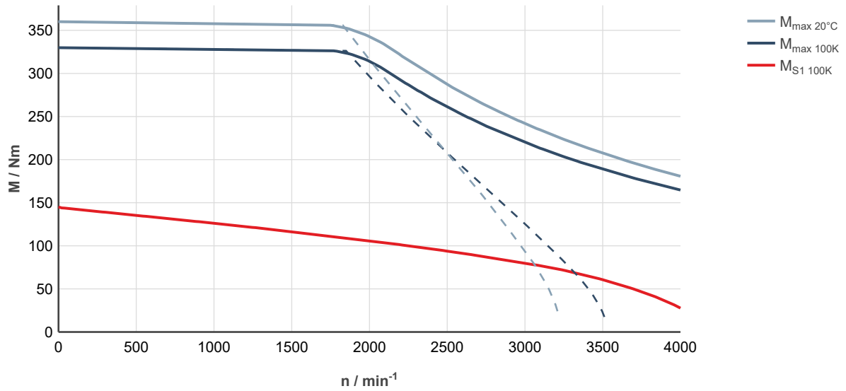
Fig. 259: MS2N10-F1BHA-___0-___-_, ctrIX DRIVE, controlled supply 3 × AC 400 ... 480 V
