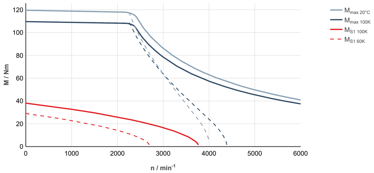
Fig. 119: MS2N07-E0BQN-___0-___-, ctrlX DRIVE, uncontrolled supply 3 × AC 400 V
