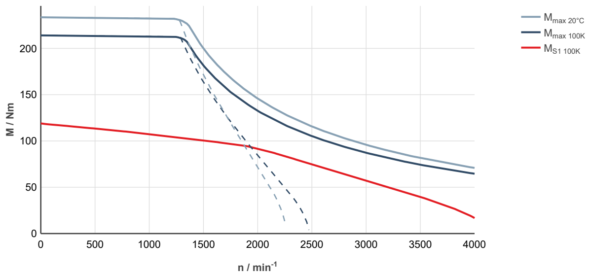
Fig. 244: MS2N10-E0BHA-___0-___-_, ctrlX DRIVE, uncontrolled supply 3 × AC 400 V
