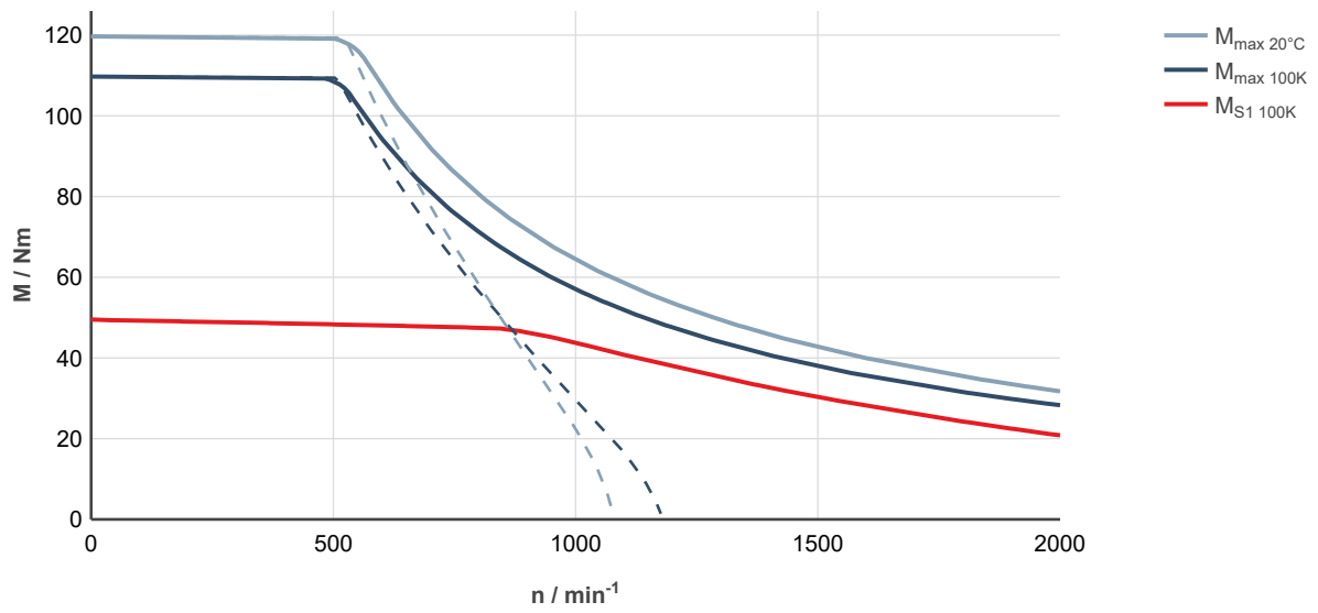
Fig. 149: MS2N07-E0BDA-___0-___-__, ctrlX DRIVE, uncontrolled supply 3 × AC 400 V
