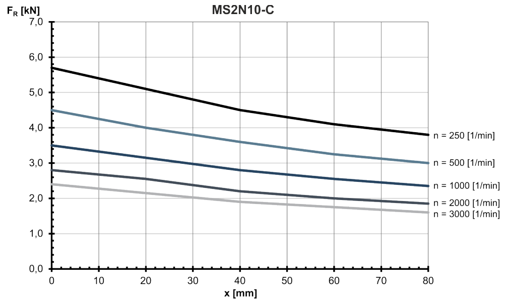
Fig. 297: MS2N10-C: Radial force in distance x from the shaft shoulder at a nominal bearing service life of L_{h10} = 30000 h
