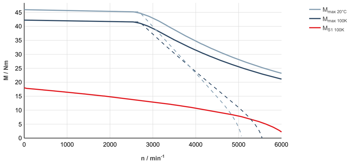
Fig. 133: MS2N07-C1BRA-___0-___-__, ctrlX DRIVE, uncontrolled supply 3 × AC 400 V
