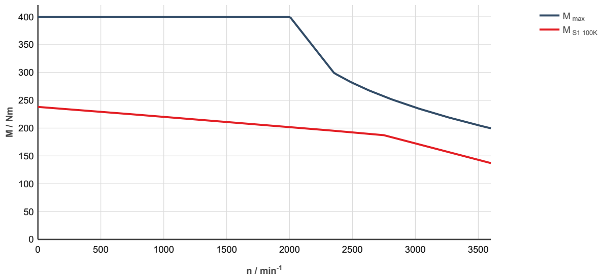
Fig. 340: MS2N13-C1BNL-___0-___-___, ctrIX DRIVE, uncontrolled supply 3 × AC 400 V
