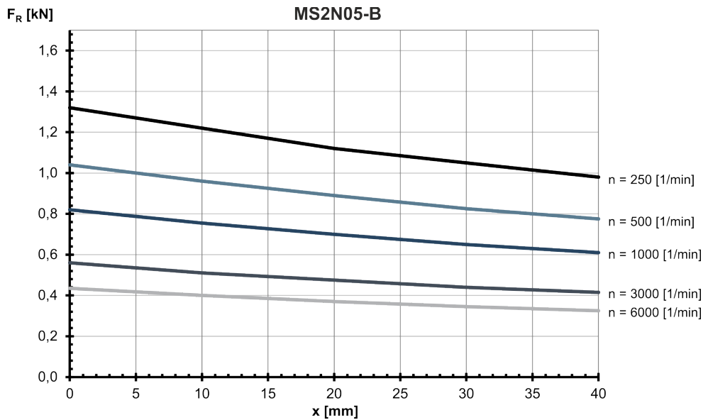
Fig. 65: MS2N05-B: Radial force in distance x from the shaft shoulder at a nominal bearing service life of L_{h10} = 30000 h
