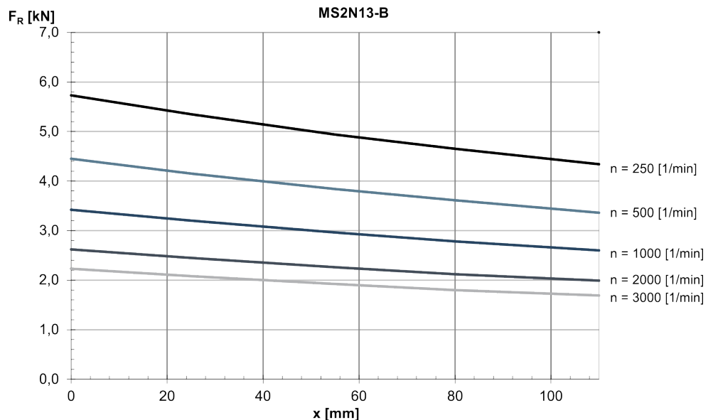
Fig. 353: MS2N13-B: Radial force in distance x from the shaft shoulder at a nominal bearing service life of L_{h10} = 30000 h
