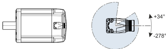
Fig. 379: Rotating area electrical connection "S"
