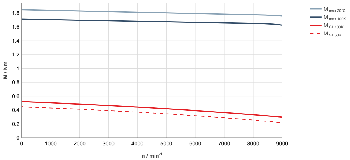
Fig. 23: MS2N03-A0BYN-___0-___-__, ctrlX DRIVE, uncontrolled supply 3 × AC 400 V
