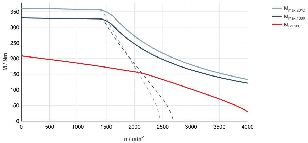
Fig. 284: MS2N10-F1BHL-___0-___-__, ctrlX DRIVE, uncontrolled supply 3 × AC 400 V
