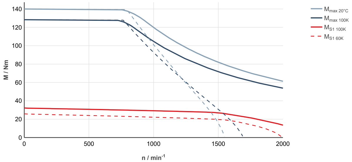
Fig. 122: MS2N07-E1BDN-___0-___-_, ctrlX DRIVE, controlled supply 3 × AC 400 ... 480 V
