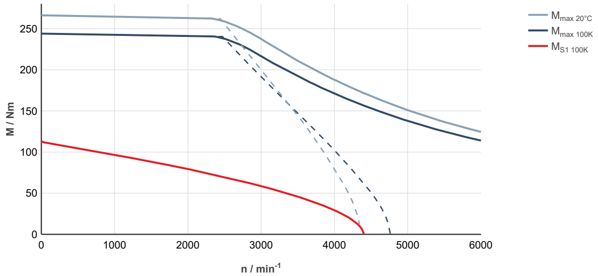
Fig. 251: MS2N10-E1BNA-___0-___-_, ctrIX DRIVE, controlled supply 3 × AC 400 ... 480 V
