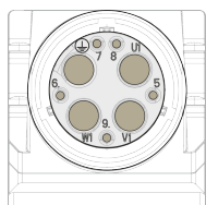
Fig. 384: Connector view of M58 performance connector
