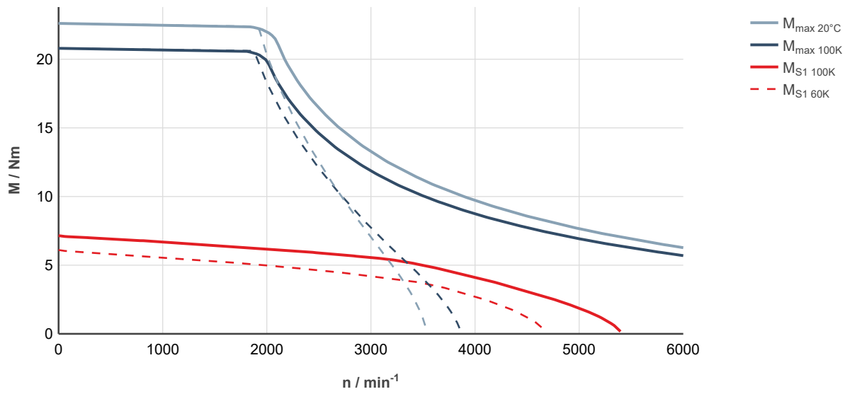
Fig. 55: MS2N05-C0BNN-___0-___-_, ctrlX DRIVE, uncontrolled supply 3 × AC 400 V
