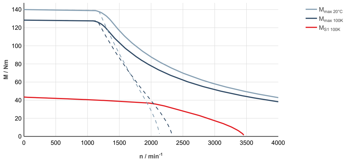
Fig. 159: MS2N07-E1BHA-___0-___-_, ctrlX DRIVE, uncontrolled supply 3 × AC 400 V
