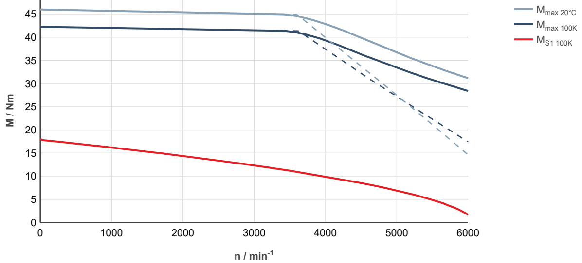
Fig. 134: MS2N07-C1BRA-___0-___-__, ctrlX DRIVE, controlled supply 3 × AC 400 ... 480 V
