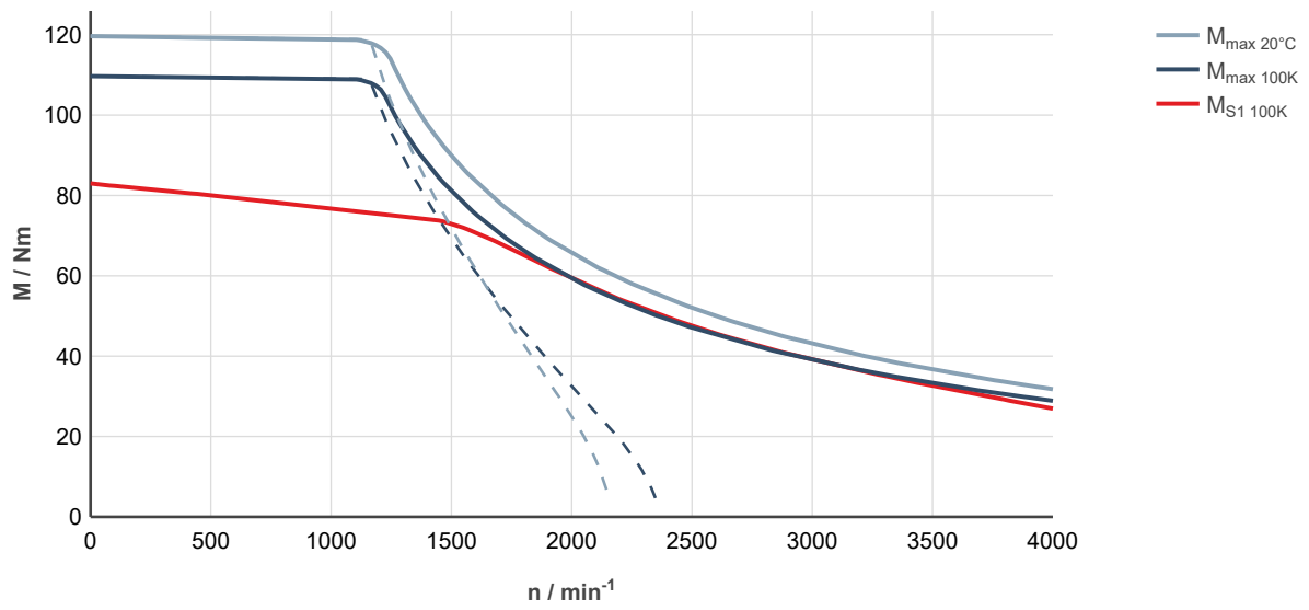
Fig. 177: MS2N07-E0BHL-___0-___-___, ctrlX DRIVE, uncontrolled supply 3 × AC 400 V
