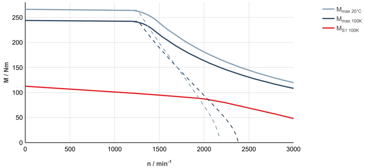
Fig. 249: MS2N10-E1BFA-___0-___-__, ctrlX DRIVE, controlled supply 3 × AC 400 ... 480 V
