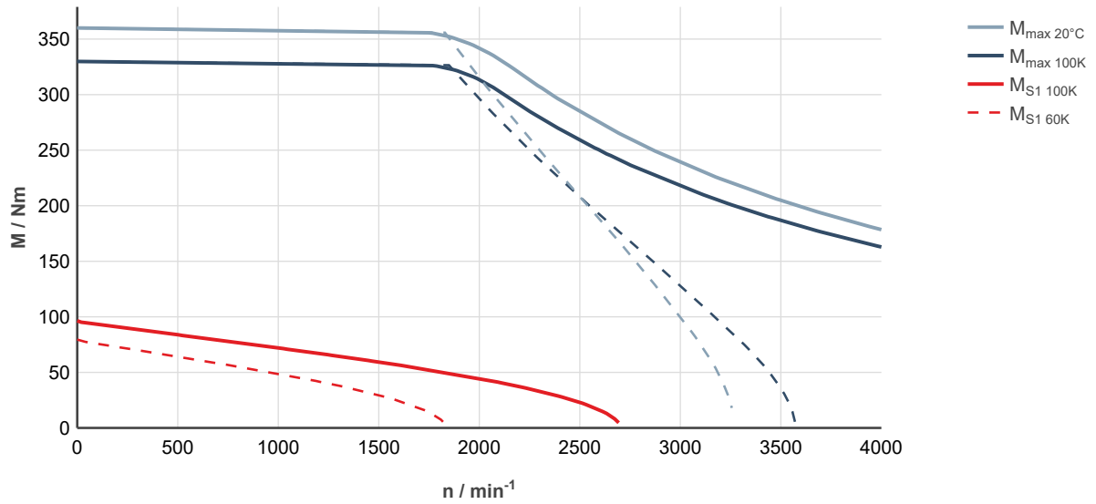
Fig. 225: MS2N10-F1BHN-___0-___-_, ctrlX DRIVE, controlled supply 3 × AC 400 ... 480 V
