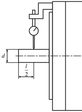
Fig. 13: Measuring system of concentricity tolerance Measurement takes place in distance l/2 (shaft end center), rectangular to the motor flange.
