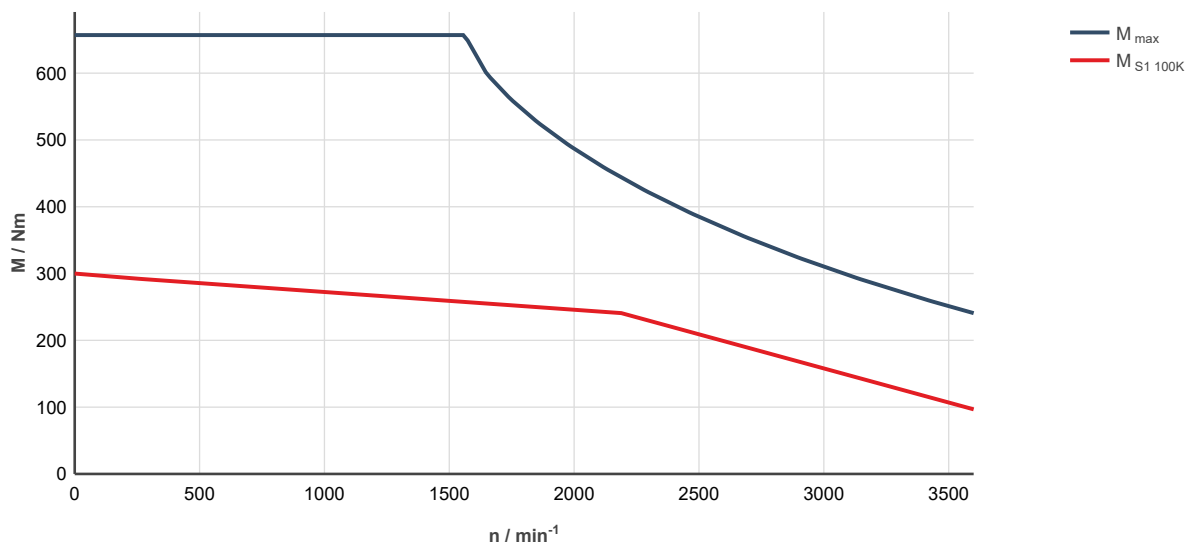
Fig. 330: MS2N13-E1BHC-___0-___-_, ctrlX DRIVE, uncontrolled supply 3 × AC 400 V M_{\text{max}} Characteristic curve applies to maximum torque 20 °C (cold)
