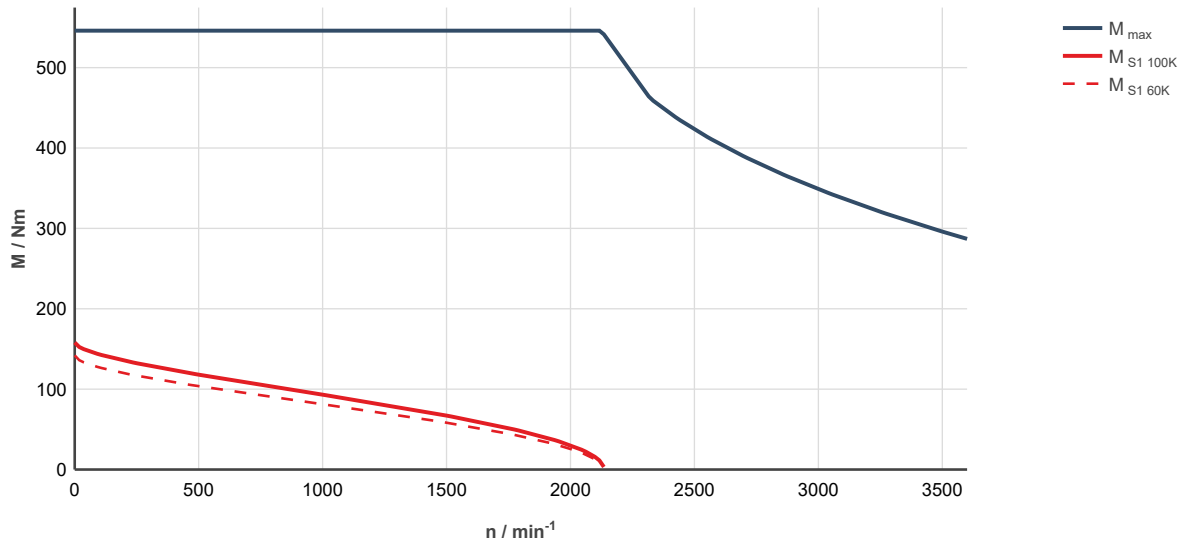
Fig. 311: MS2N13-D1BHN-___0-___-_, ctrlX DRIVE, controlled supply 3 x AC 400 ... 480 V
