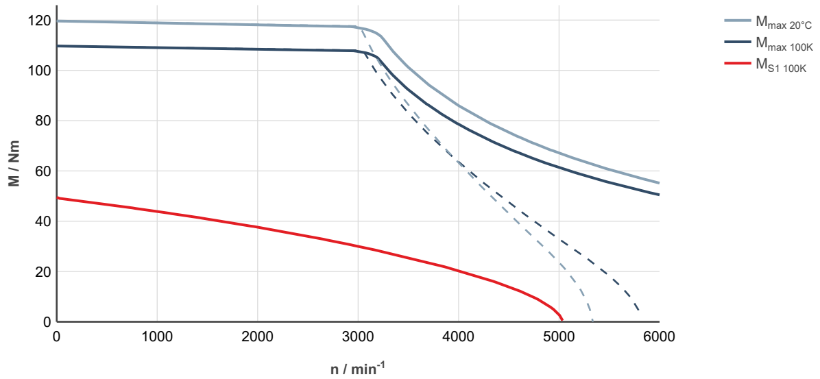
Fig. 156: MS2N07-E0BQA-___0-___-_, ctrlX DRIVE, controlled supply 3 × AC 400 ... 480 V
