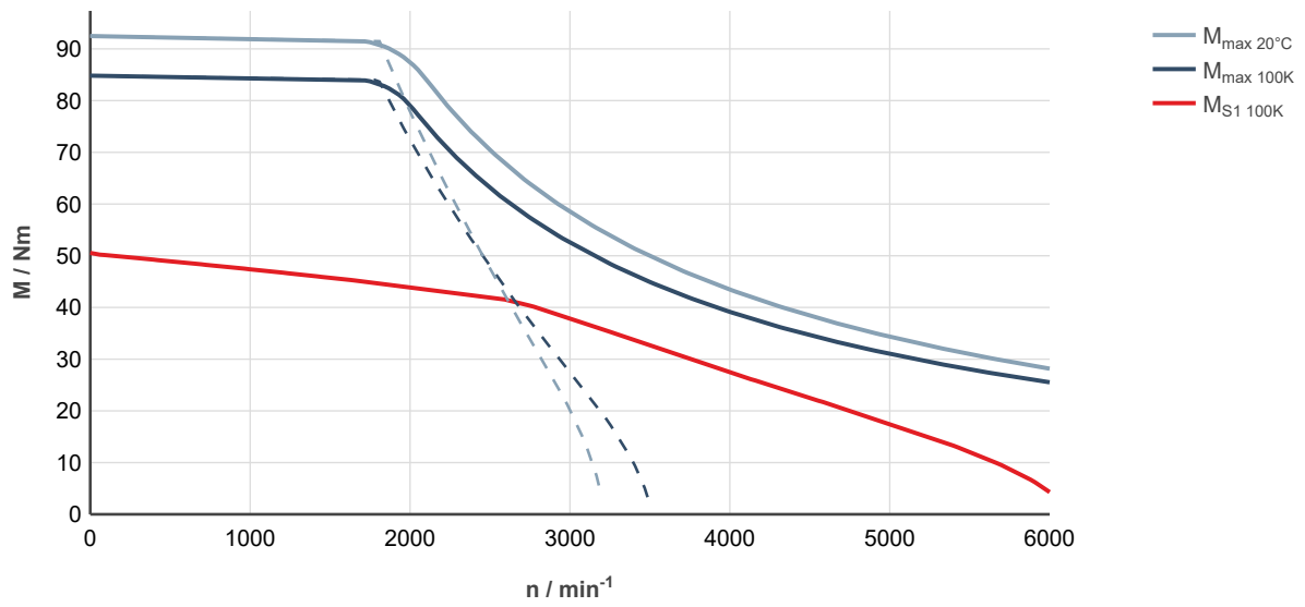
Fig. 175: MS2N07-D1BNL-___0-___-___, ctrIX DRIVE, uncontrolled supply 3 × AC 400 V
