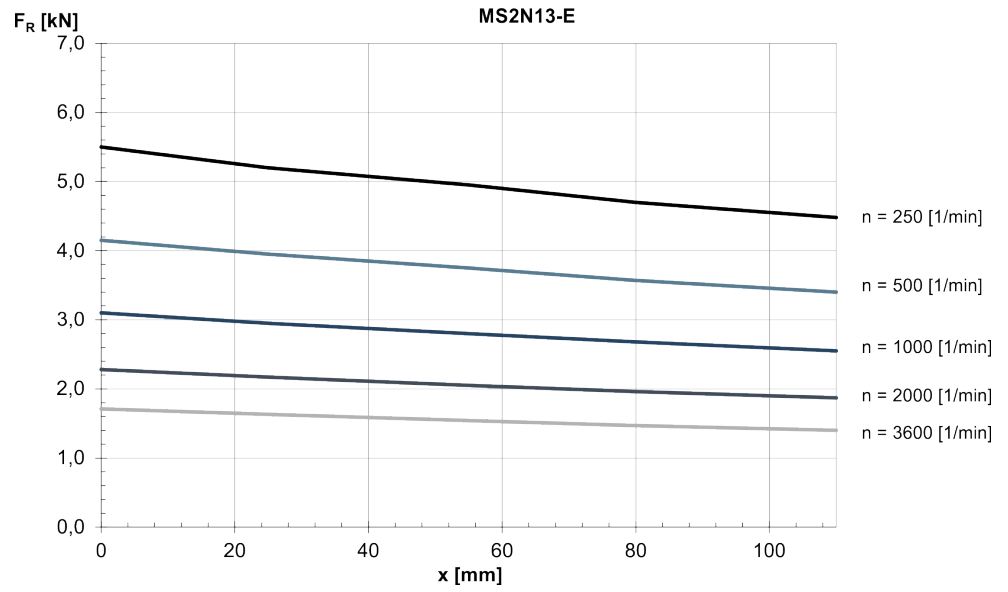
Fig. 356: MS2N13-E: Radial force in distance x from the shaft shoulder at a nominal bearing service life of L_{h10} = 30000 h
