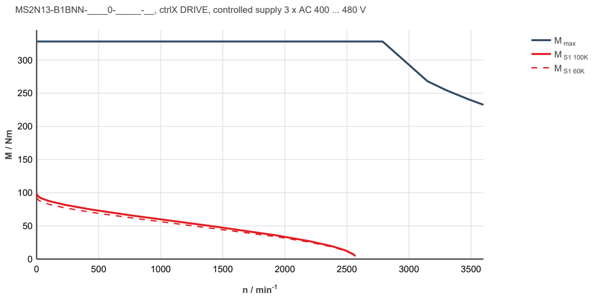
Fig. 305: MS2N13-B1BNN-___0-___-___, ctrlX DRIVE, controlled supply 3 x AC 400 ... 480 V
