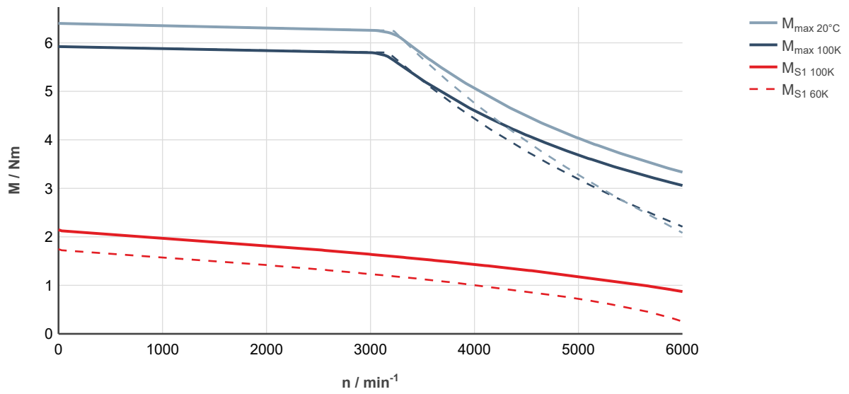
Fig. 36: MS2N04-B0BTN-___0-___-__, ctrlX DRIVE, uncontrolled supply 3 × AC 400 V
