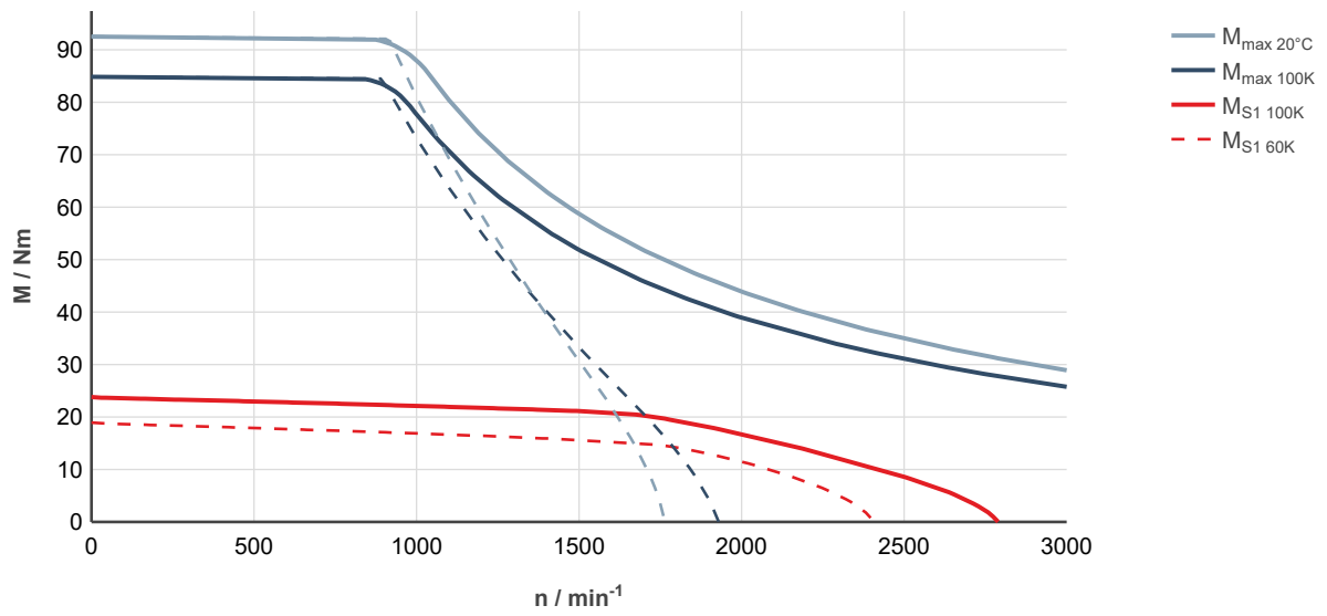
Fig. 107: MS2N07-D1BFN-___0-___-_, ctrlX DRIVE, uncontrolled supply 3 × AC 400 V
