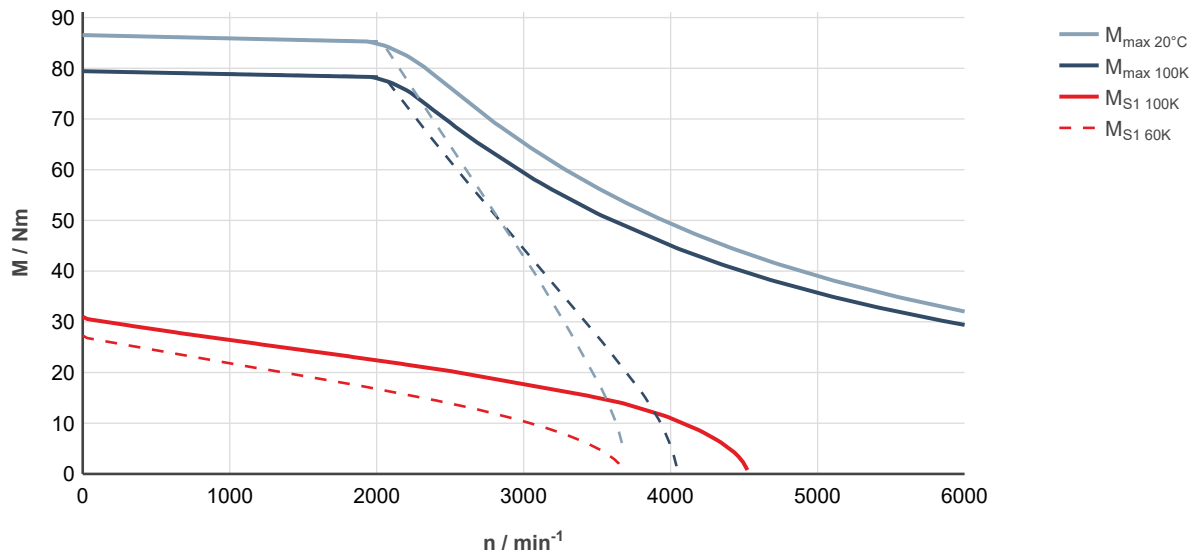
Fig. 200: MS2N10-C1BNN-___0-___-_, ctrlX DRIVE, uncontrolled supply 3 × AC 400 V
