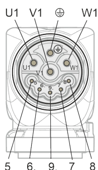
Fig. 380: Connector view of M23 performance connector
