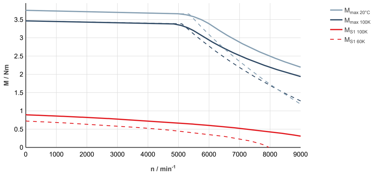
Fig. 25: MS2N03-B0BYN-___0-___-_, ctrlX DRIVE, uncontrolled supply 3 × AC 400 V
