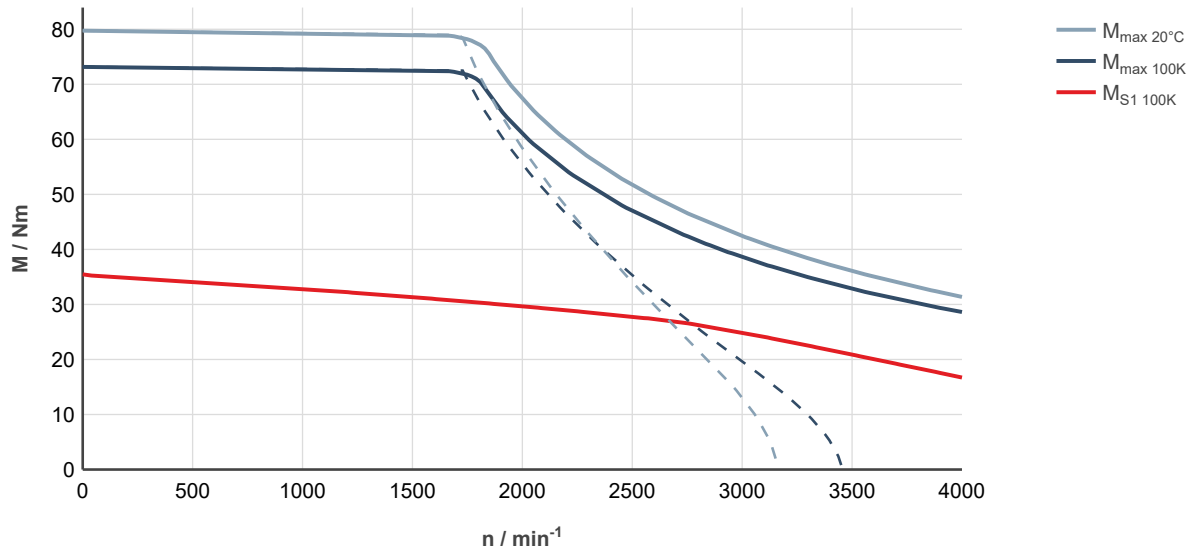
Fig. 138: MS2N07-D0BHA-___0-___-_, ctrlX DRIVE, controlled supply 3 × AC 400 ... 480 V
