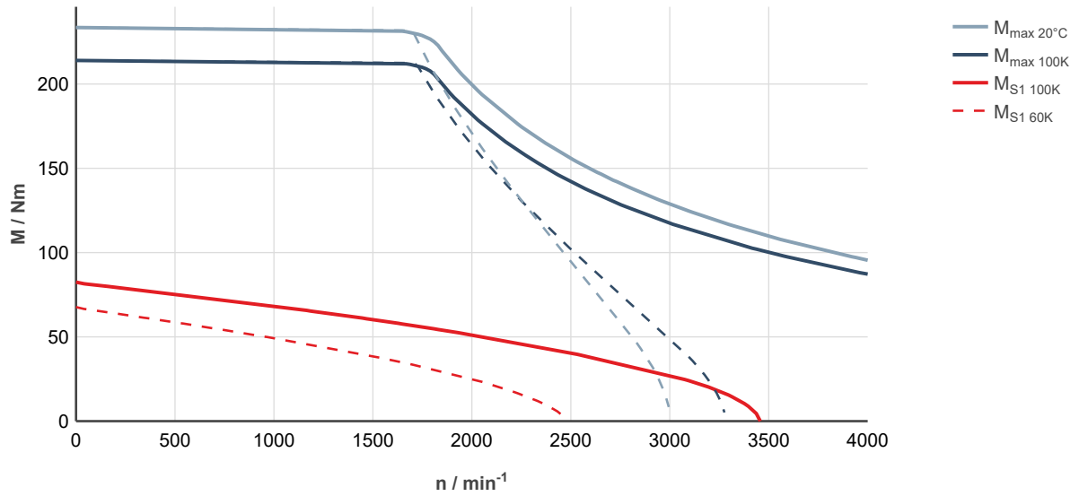
Fig. 211: MS2N10-E0BHN-___0-___-_, ctrlX DRIVE, controlled supply 3 × AC 400 ... 480 V
