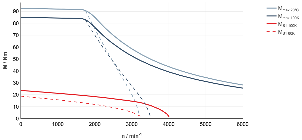
Fig. 111: MS2N07-D1BNN-___0-___-, ctrlX DRIVE, uncontrolled supply 3 × AC 400 V
