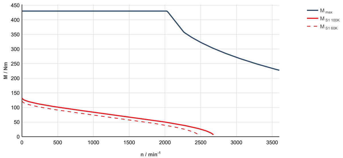
Fig. 307: MS2N13-C1BHN-___0-___-_, ctrlX DRIVE, controlled supply 3 x AC 400 ... 480 V
