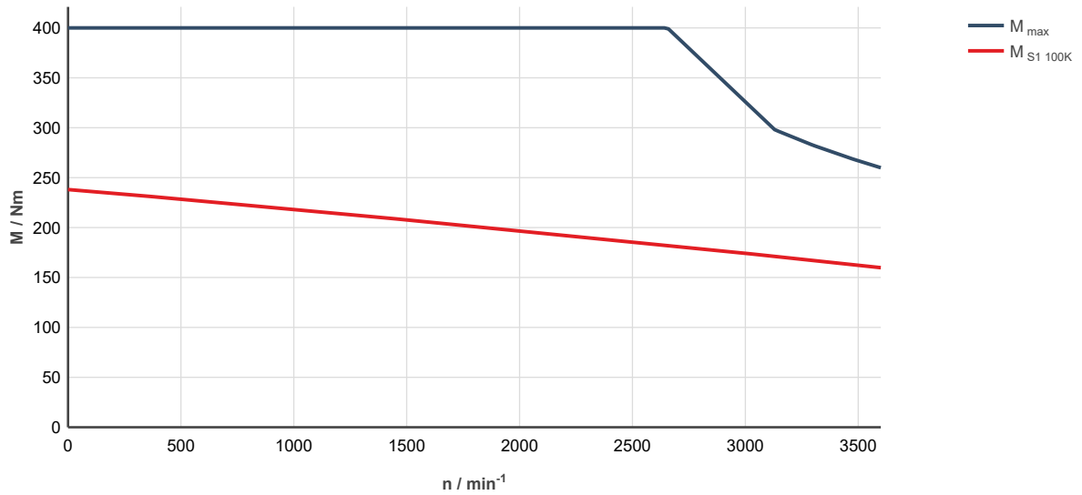
Fig. 341: MS2N13-C1BNL-___0-___-___, ctrIX DRIVE, controlled supply 3 x AC 400 ... 480 V
