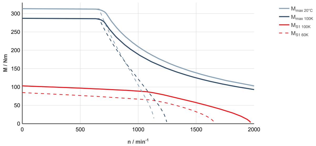
Fig. 218: MS2N10-F0BDN-___0-___-_, ctrlX DRIVE, uncontrolled supply 3 × AC 400 V
