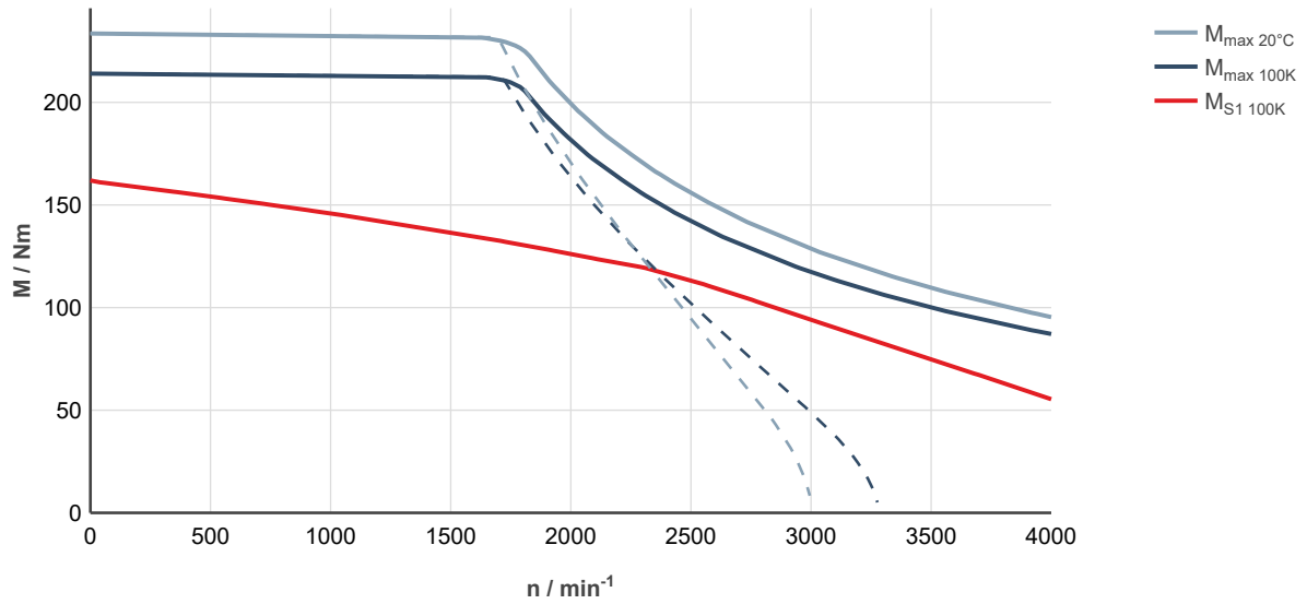
Fig. 275: MS2N10-E0BHL-___0-___-__, ctrlX DRIVE, controlled supply 3 × AC 400 ... 480 V
