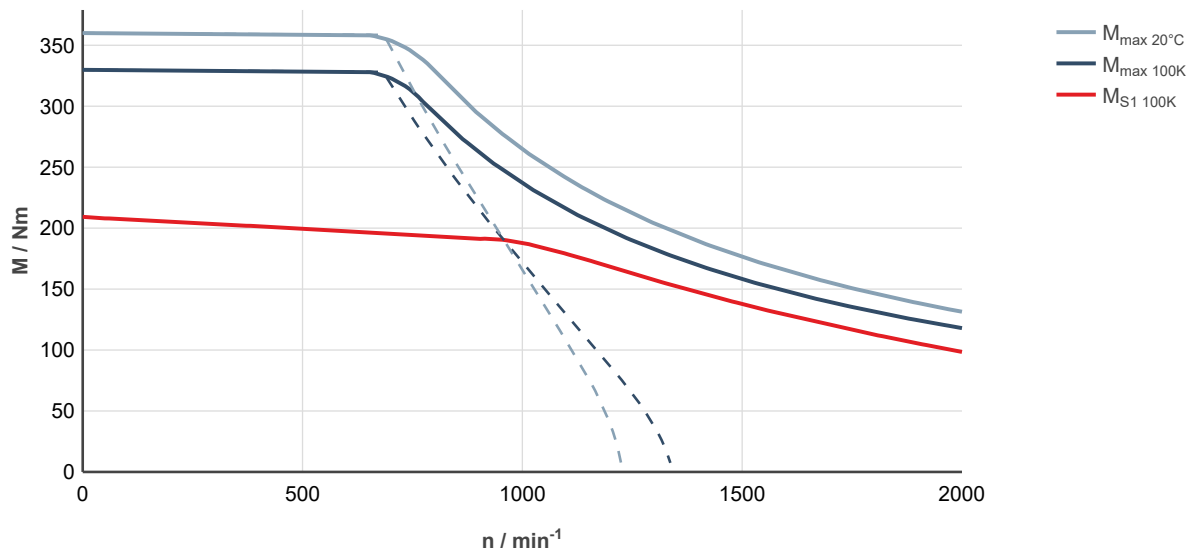
Fig. 282: MS2N10-F1BDL-___0-___-__, ctrlX DRIVE, uncontrolled supply 3 × AC 400 V
