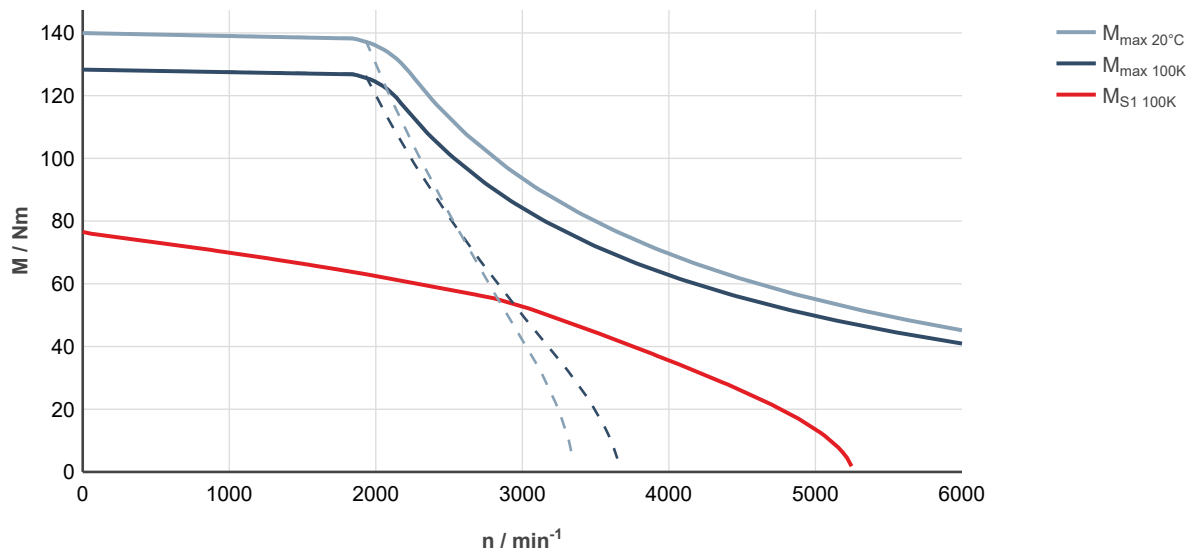
Fig. 183: MS2N07-E1BNL-__0-__-__, ctrlX DRIVE, uncontrolled supply 3 × AC 400 V
