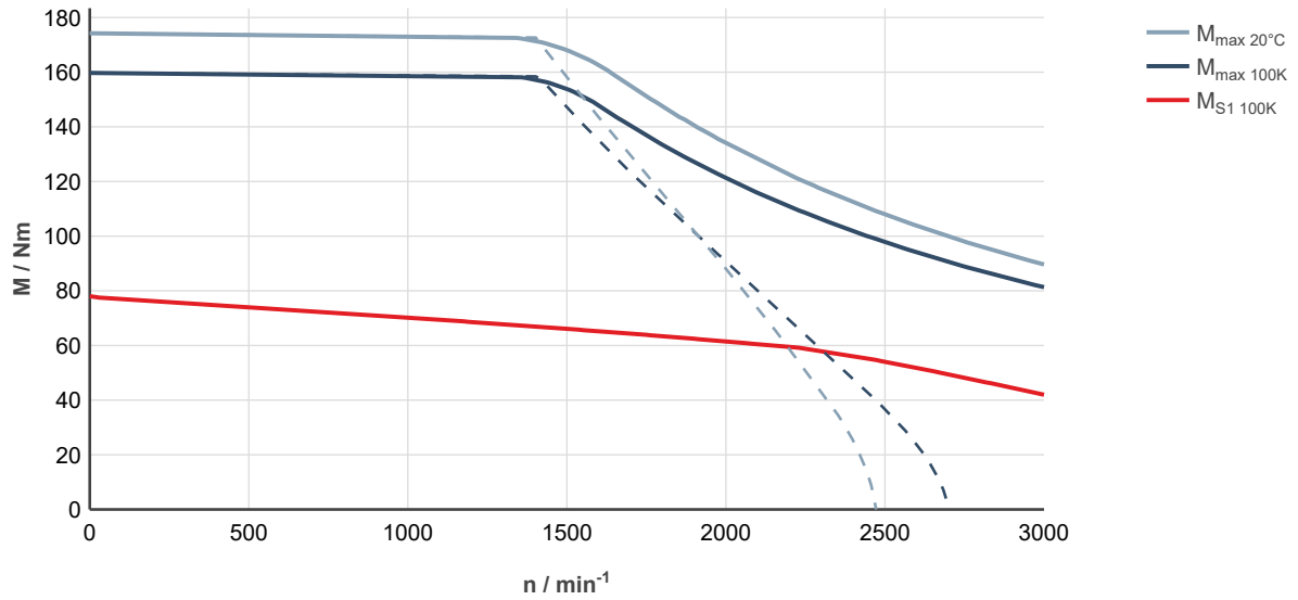
Fig. 241: MS2N10-D1BFA-___0-___-__, ctrlX DRIVE, controlled supply 3 × AC 400 ... 480 V
