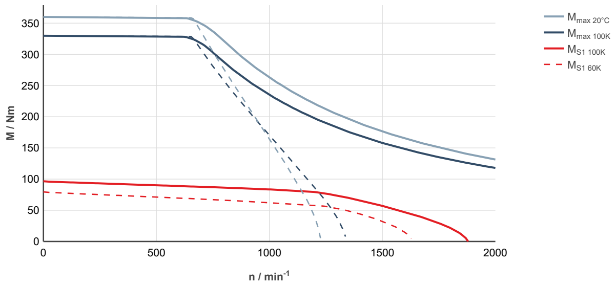
Fig. 222: MS2N10-F1BDN-___0-___-_, ctrlX DRIVE, uncontrolled supply 3 × AC 400 V
