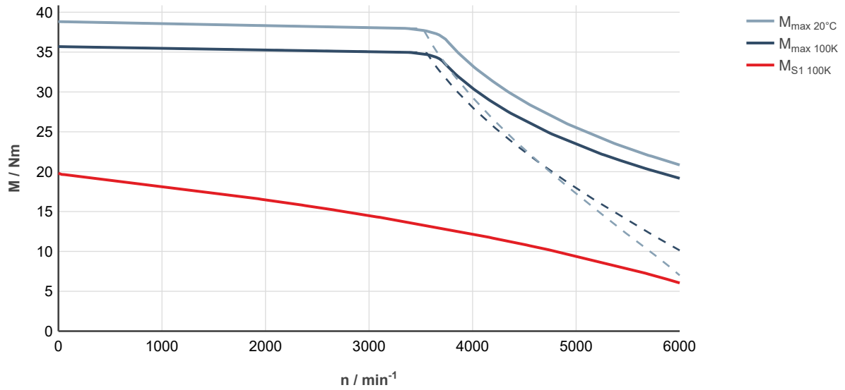
Fig. 130: MS2N07-C0BQA-___0-___-_, ctrlX DRIVE, controlled supply 3 × AC 400 ... 480 V
