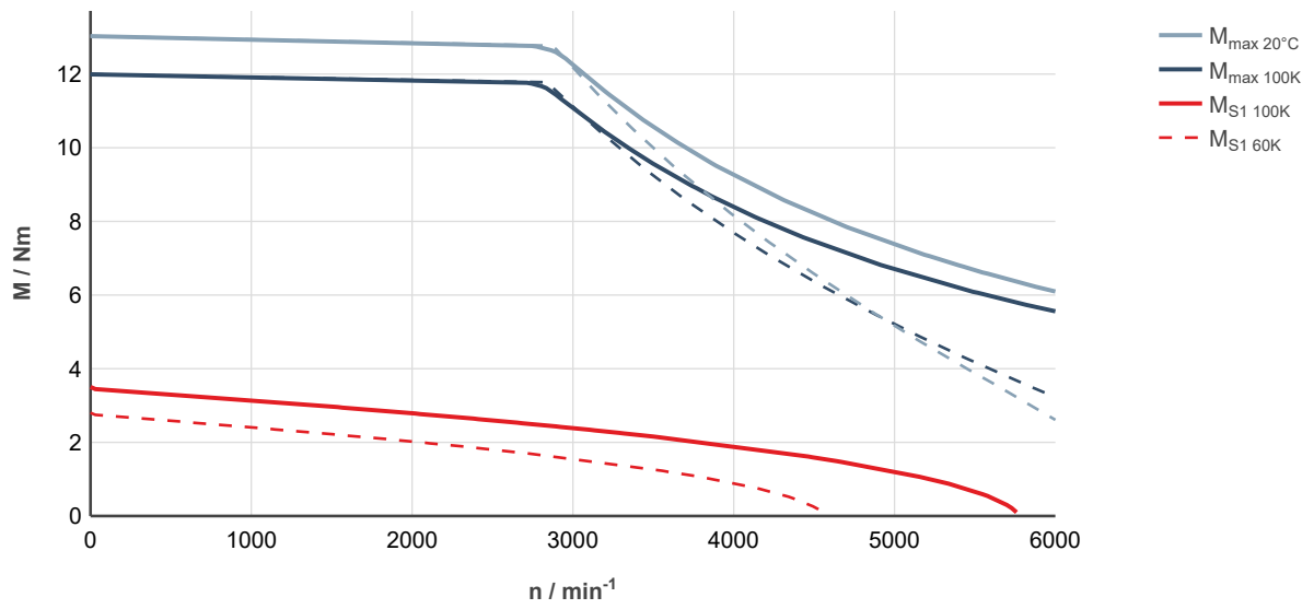
Fig. 40: MS2N04-C0BTN-___0-___-__, ctrlX DRIVE, uncontrolled supply 3 × AC 400 V
