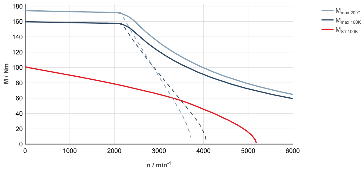
Fig. 272: MS2N10-D1BNL-___0-___-___, ctrIX DRIVE, uncontrolled supply 3 × AC 400 V
