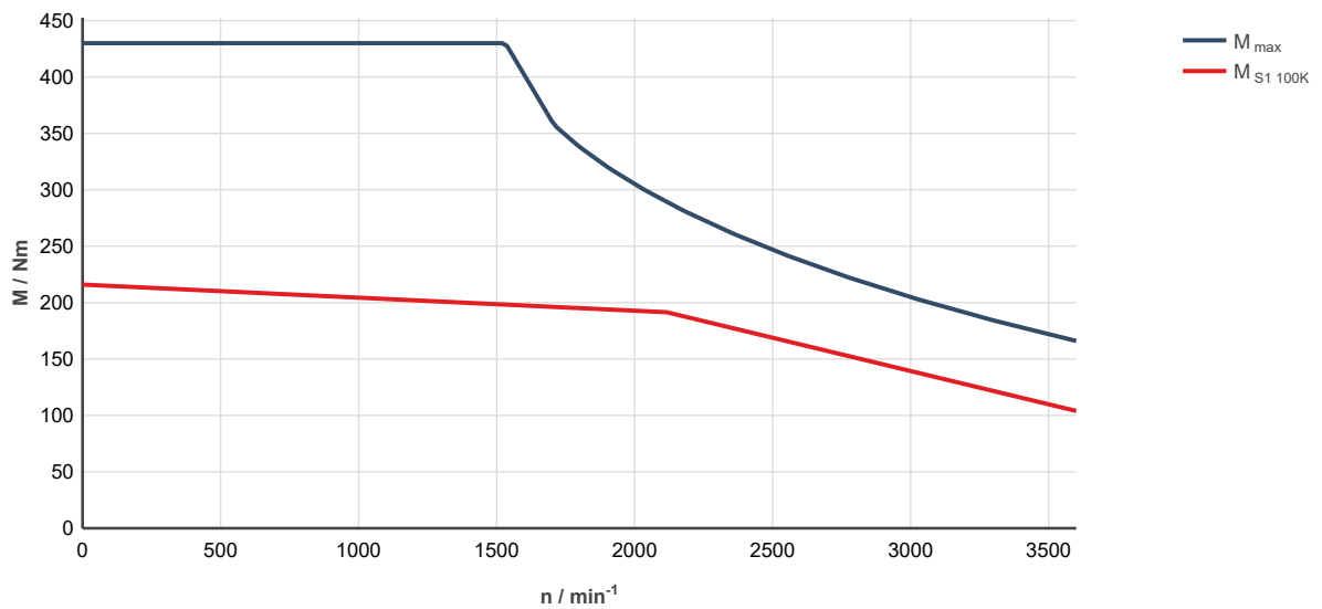
Fig. 322: MS2N13-C1BHC-___0-___-_, ctrIX DRIVE, uncontrolled supply 3 × AC 400 V M_{max} Characteristic curve applies to maximum torque 20 °C (cold)
