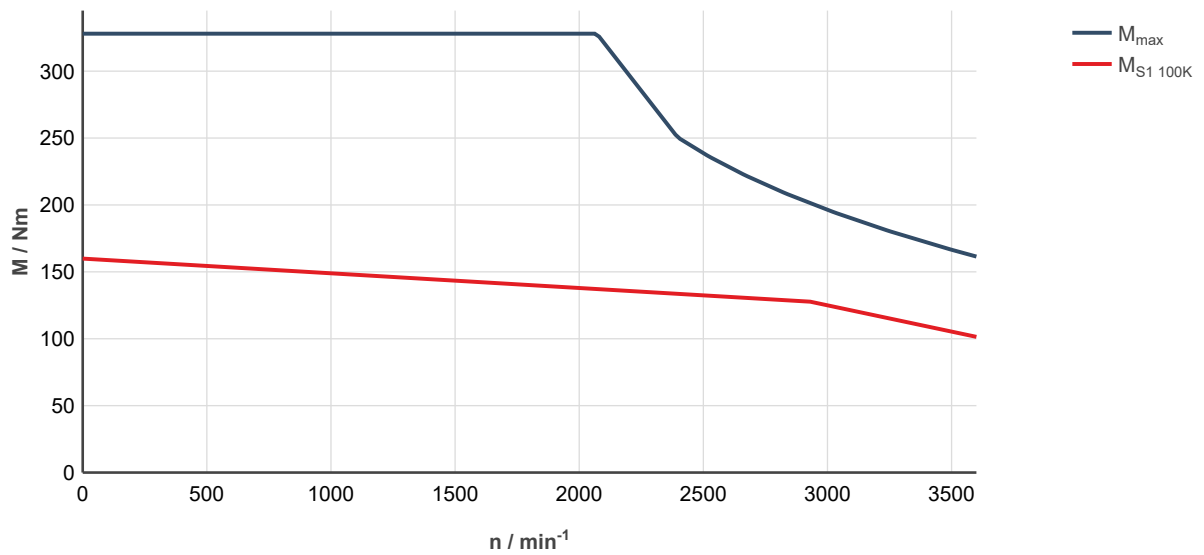
Fig. 319: MS2N13-B1BHC-___0-___-_, ctrIX DRIVE, controlled supply 3 × AC 400 ... 480 V M_{\text{max}} Characteristic curve applies to maximum torque 20 °C (cold)
