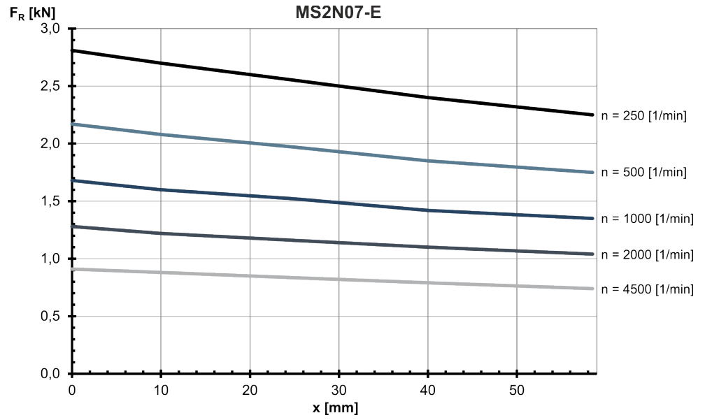
Fig. 191: MS2N07-E: Radial force in distance x from the shaft shoulder at a nominal bearing service life of L_{h10} = 30000 h
