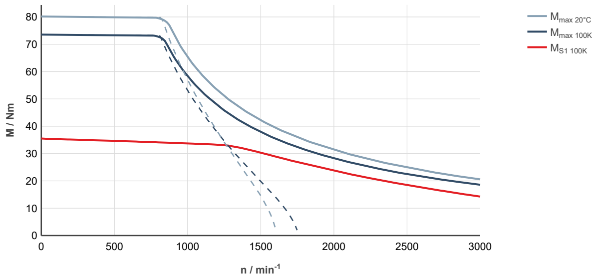
Fig. 135: MS2N07-D0BFA-...0-...-..., ctrlX DRIVE, uncontrolled supply 3 × AC 400 V
