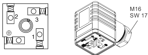
Fig. 386: RLSxxxx_Single components fan connector
