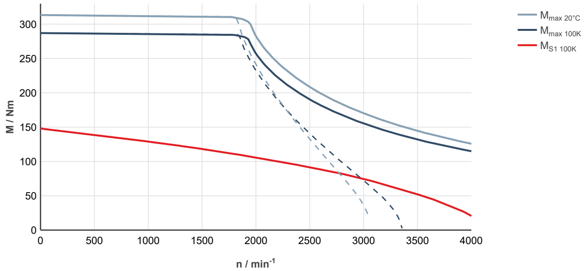
Fig. 255: MS2N10-F0BHA-___0-___-_, ctrIX DRIVE, controlled supply 3 × AC 400 ... 480 V
