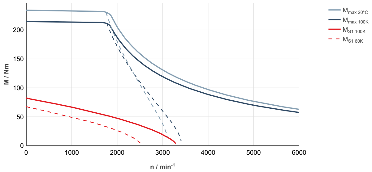
Fig. 212: MS2N10-E0BNN-___0-___-_, ctrlX DRIVE, uncontrolled supply 3 × AC 400 V
