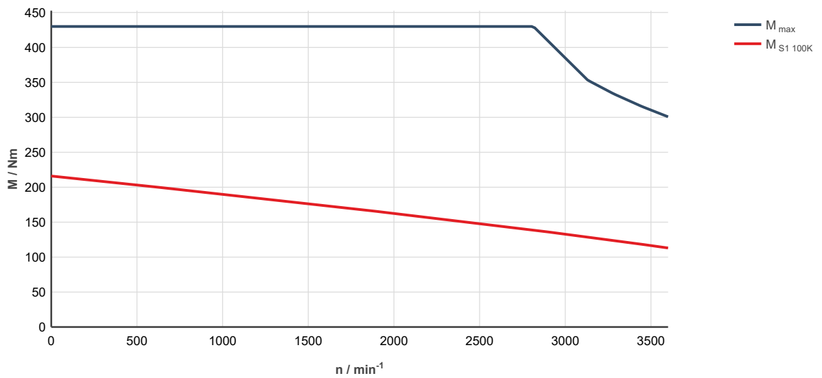
Fig. 325: MS2N13-C1BNC-___0-N___-___, ctrlX DRIVE, controlled supply 3 x AC 400 ... 480 V
