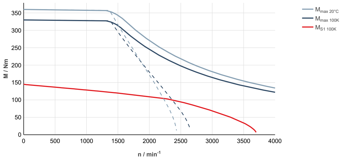
Fig. 258: MS2N10-F1BHA-___0-___-_, ctrIX DRIVE, uncontrolled supply 3 × AC 400 V
