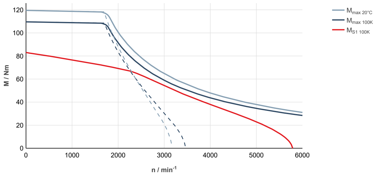
Fig. 179: MS2N07-E0BNL-___0-___-___, ctrlX DRIVE, uncontrolled supply 3 × AC 400 V
