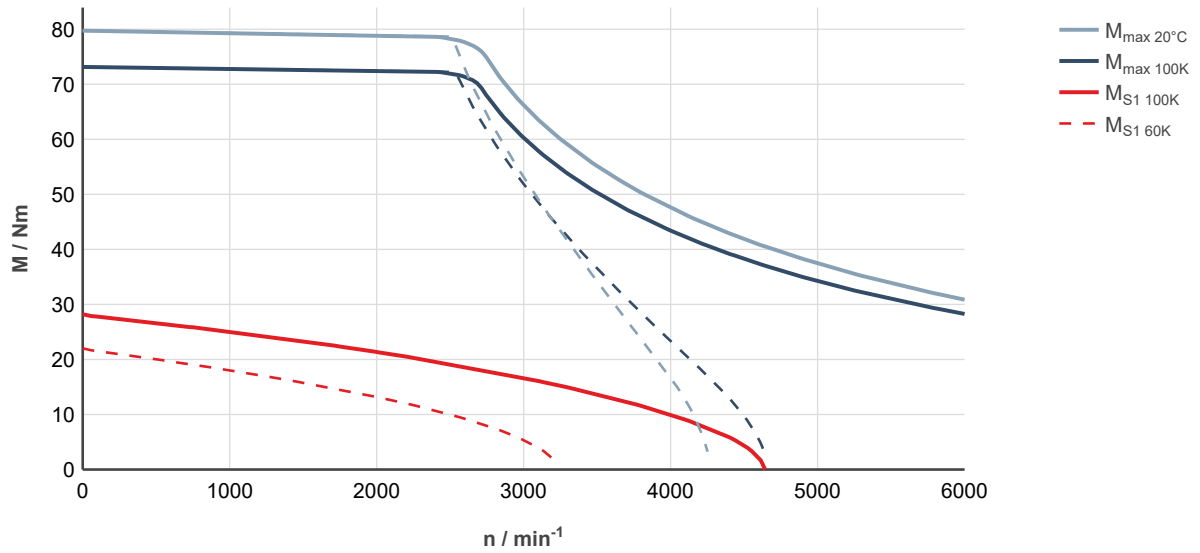
Fig. 104: MS2N07-D0BNN-___0-___-, ctrlX DRIVE, controlled supply 3 × AC 400 ... 480 V
