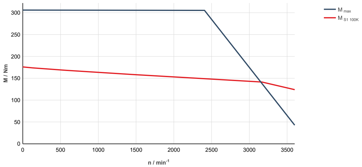
Fig. 336: MS2N13-B1BNL-___0-___-__, ctrlX DRIVE, uncontrolled supply 3 × AC 400 V
