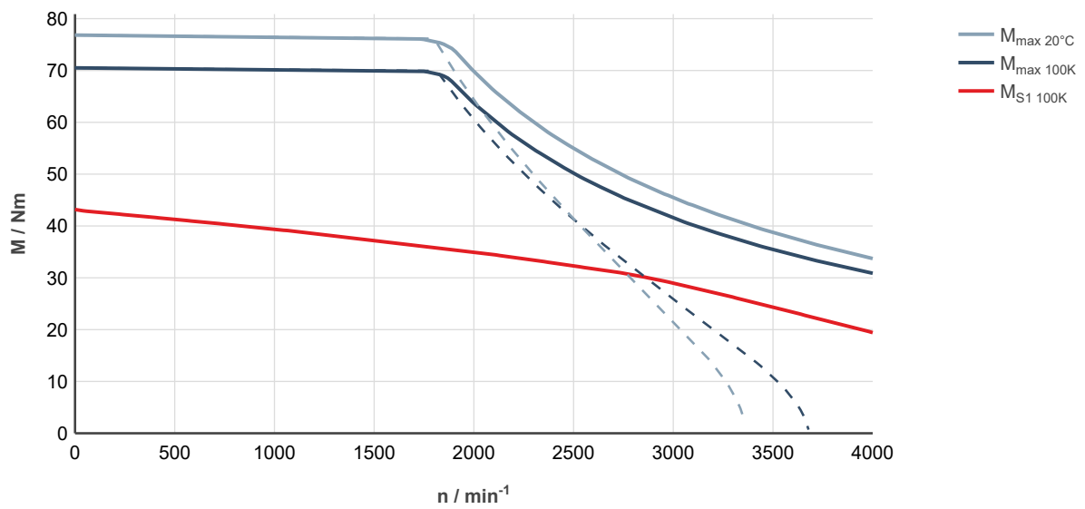
Fig. 229: MS2N10-C0BHA-___0-___-_, ctrlX DRIVE, controlled supply 3 × AC 400 ... 480 V
