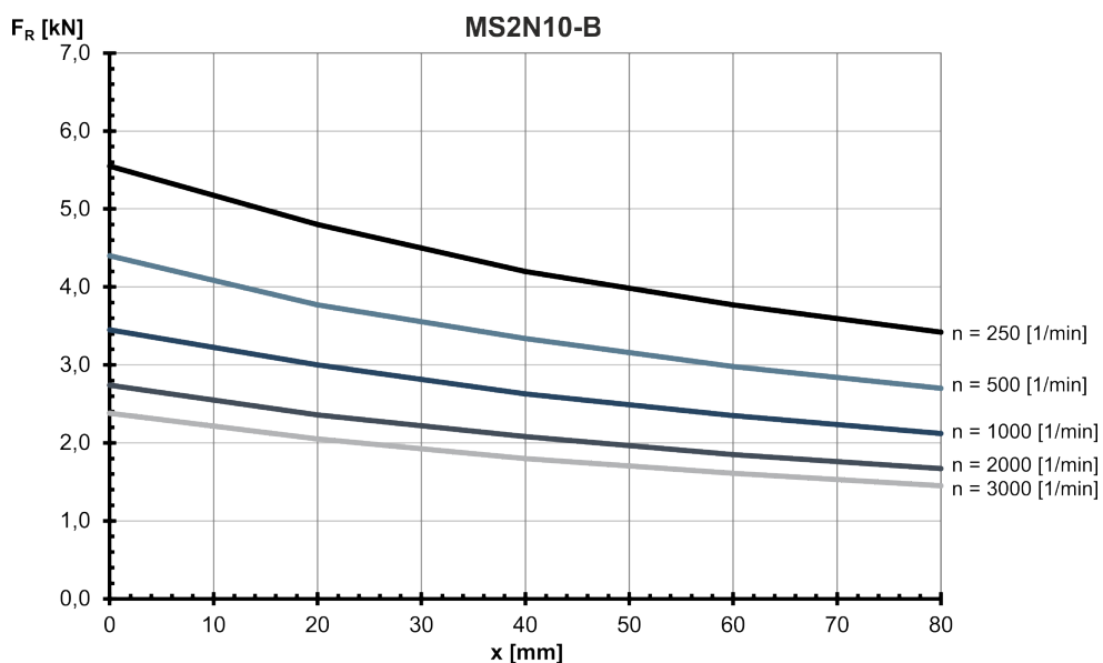
Fig. 296: MS2N10-B: Radial force in distance x from the shaft shoulder at a nominal bearing service life of L_{h10} = 30000 h
