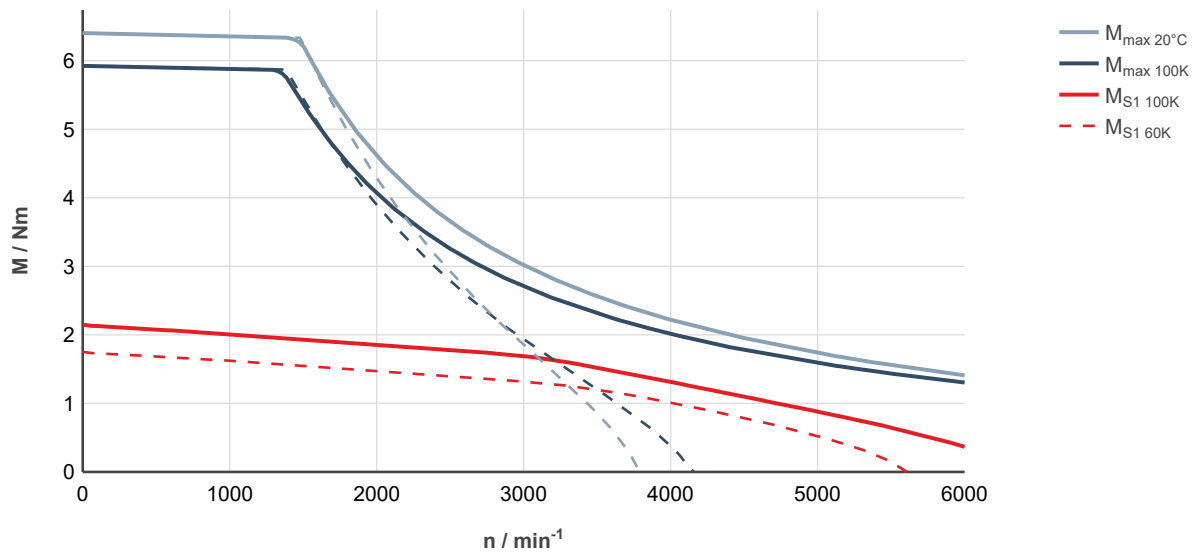
Fig. 34: MS2N04-B0BNN-___0-___-___, ctrlX DRIVE, uncontrolled supply 3 × AC 400 V
