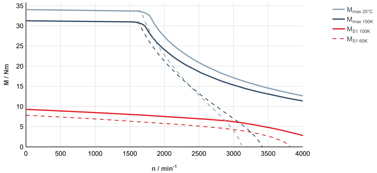
Fig. 60: MS2N05-D0BHN-___0-___-_, ctrlX DRIVE, controlled supply 3 × AC 400 ... 480 V
