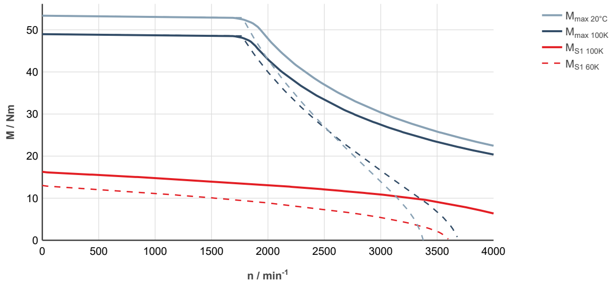
Fig. 81: MS2N06-E0BHN-___0-___-__, ctrlX DRIVE, controlled supply 3 × AC 400 ... 480 V
