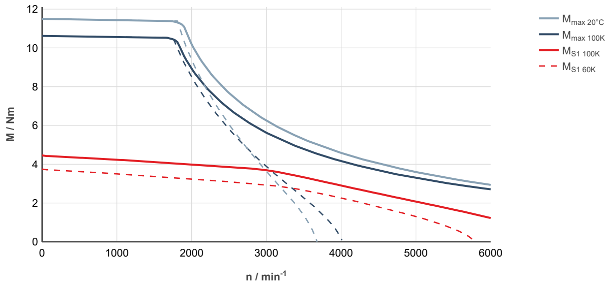
Fig. 51: MS2N05-B0BNN-___0-___-__, ctrlX DRIVE, uncontrolled supply 3 × AC 400 V
