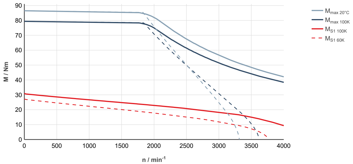
Fig. 199: MS2N10-C1BHN-___0-___-_, ctrlX DRIVE, controlled supply 3 × AC 400 ... 480 V
