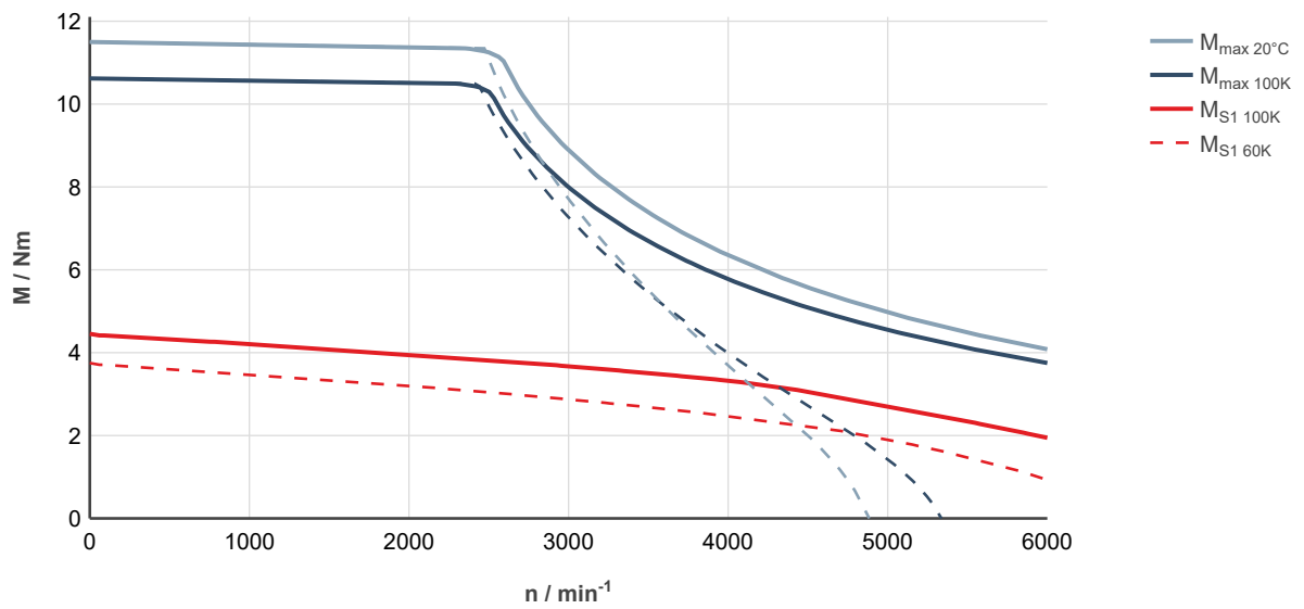
Fig. 52: MS2N05-B0BNN-___0-___-__, ctrlX DRIVE, controlled supply 3 × AC 400 ... 480 V
