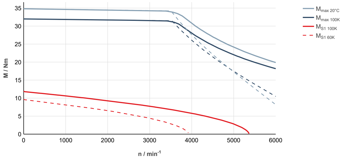
Fig. 77: MS2N06-D0BRN-___0-___-__, ctrlX DRIVE, controlled supply 3 × AC 400 ... 480 V
