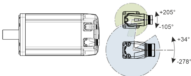
Fig. 367: Rotating area electrical connection "U"
