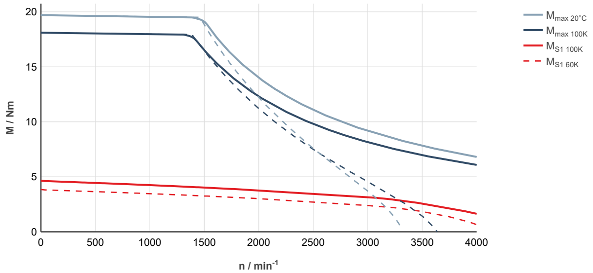
Fig. 43: MS2N04-D0BHN-___0-___-_, ctrlX DRIVE, controlled supply 3 × AC 400 ... 480 V
