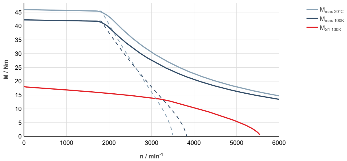
Fig. 131: MS2N07-C1BNA-___0-___-_, ctrlX DRIVE, uncontrolled supply 3 × AC 400 V
